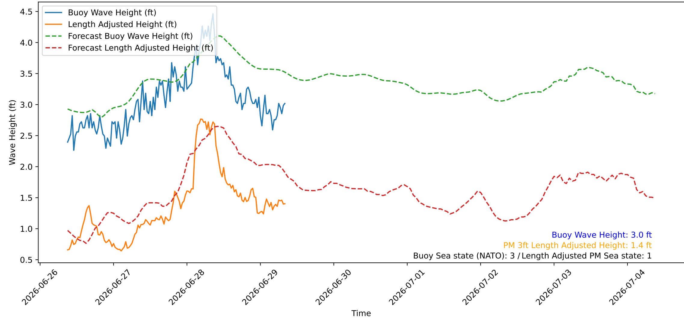
Wave Heights over Time for Red Beach at 2026-06-29 08:50:47
