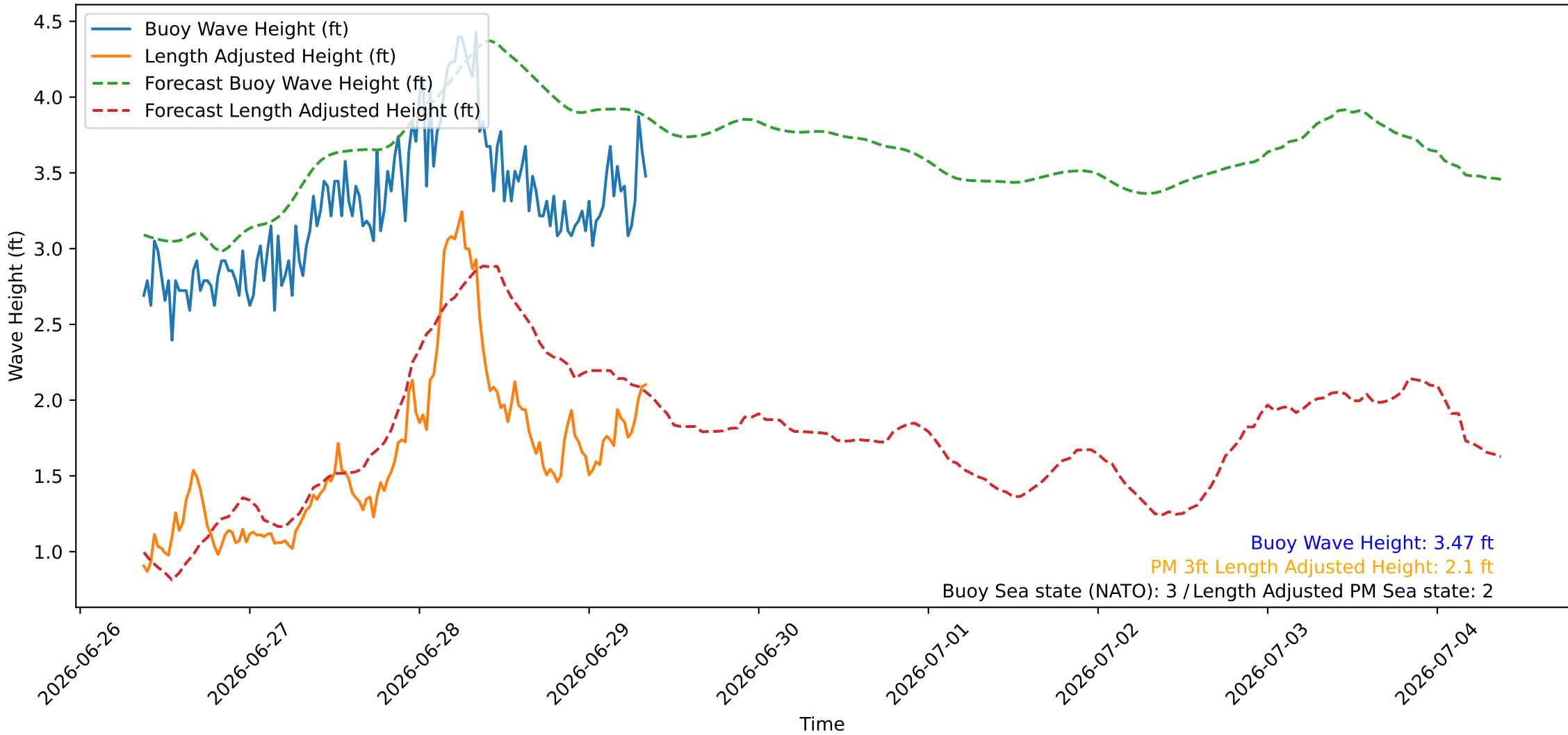
Wave Heights over Time for Oceanside Harbor at 2026-06-29 08:50:26
