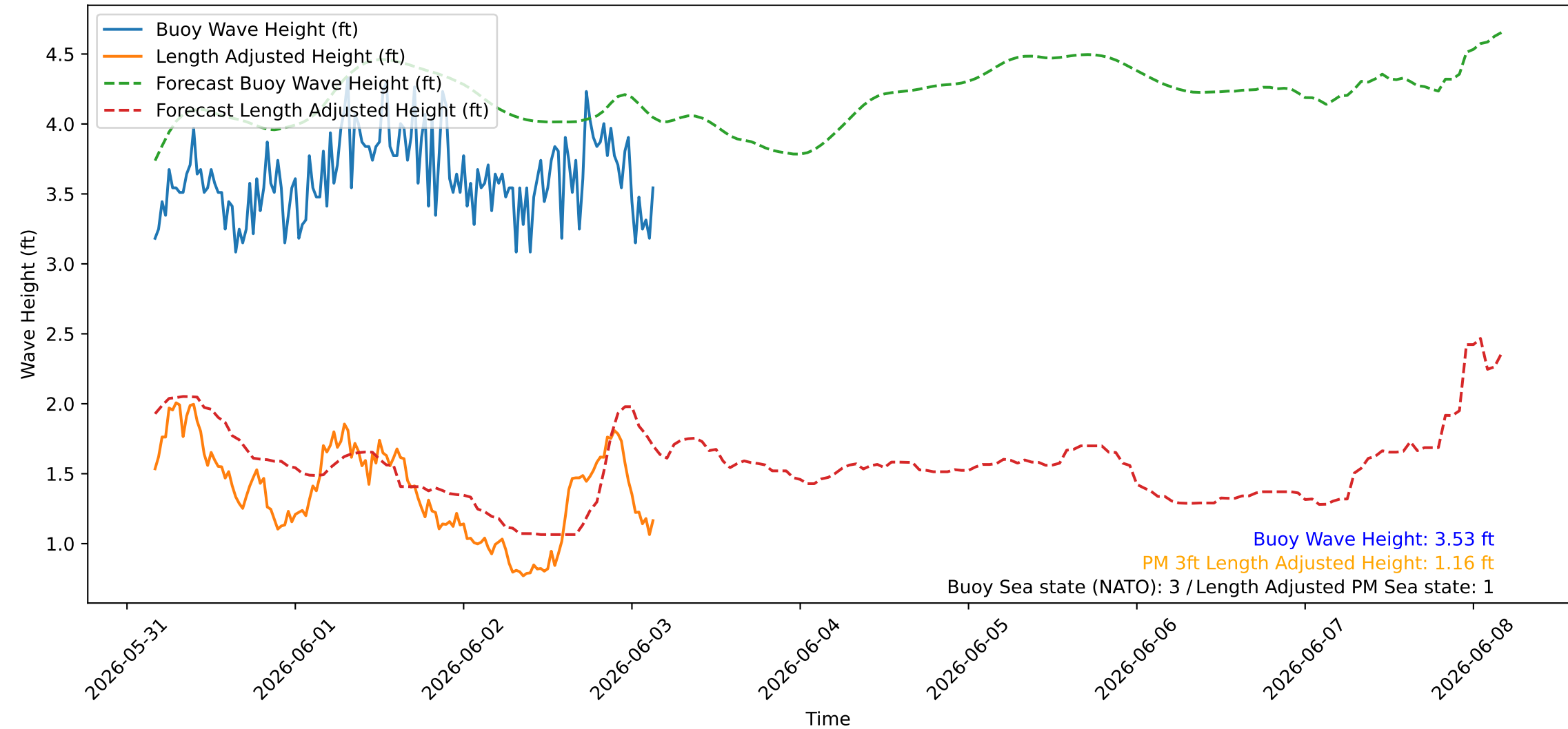
Wave Heights over Time for Green Beach at 2026-06-03 03:51:08
