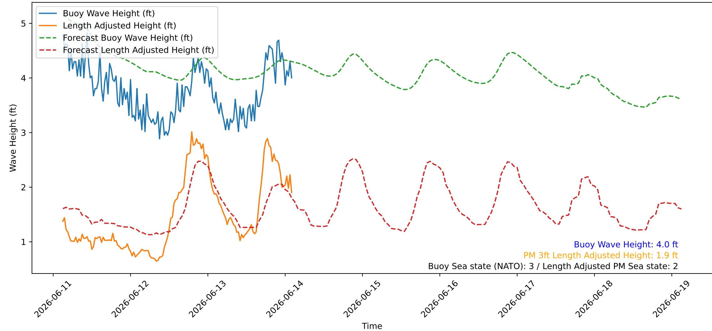
Wave Heights over Time for Green Beach at 2026-06-14 02:51:10
