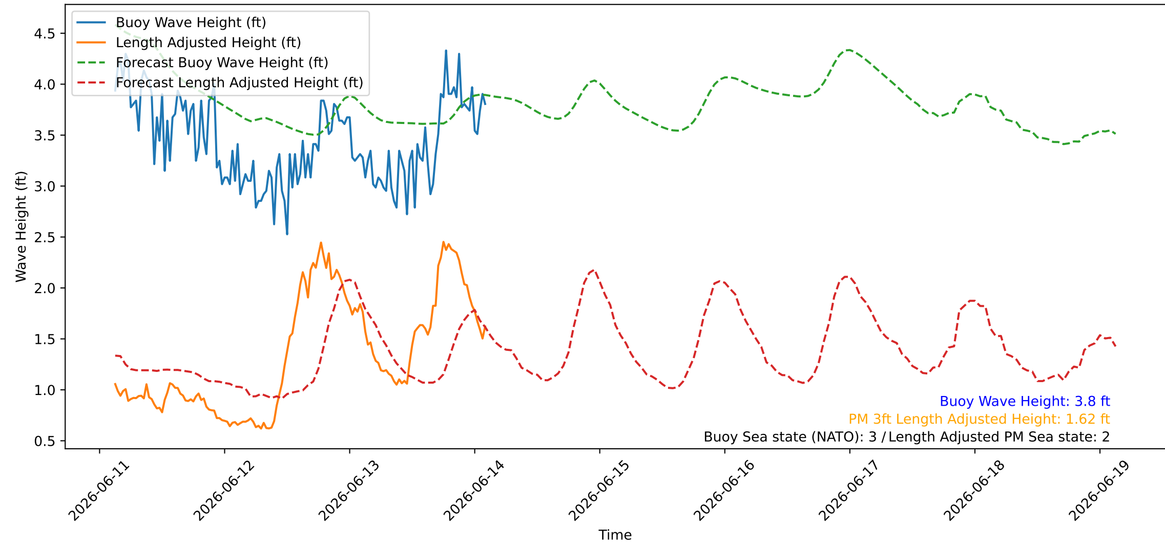
Wave Heights over Time for Red Beach at 2026-06-14 02:50:47
