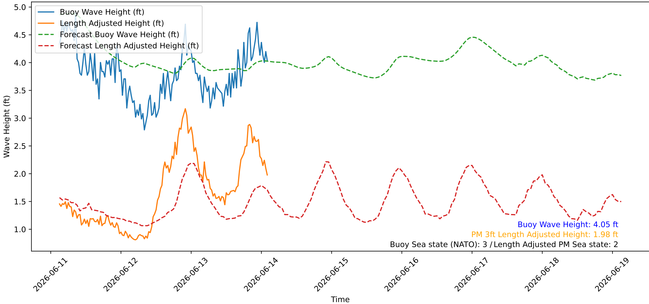
Wave Heights over Time for Oceanside Harbor at 2026-06-14 02:50:26
