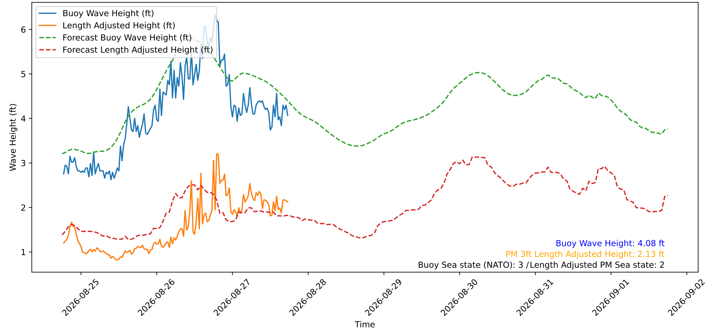
Wave Heights over Time for Green Beach at 2026-08-27 18:11:14
