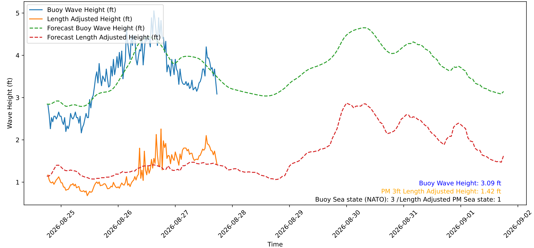
Wave Heights over Time for Red Beach at 2026-08-27 18:10:51
