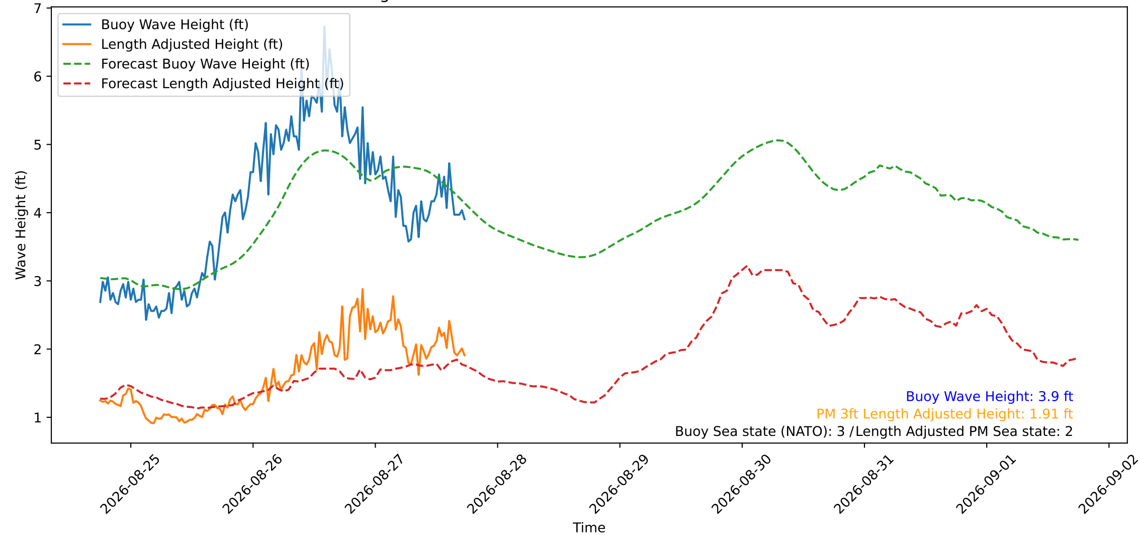
Wave Heights over Time for Oceanside Harbor at 2026-08-27 18:10:31
