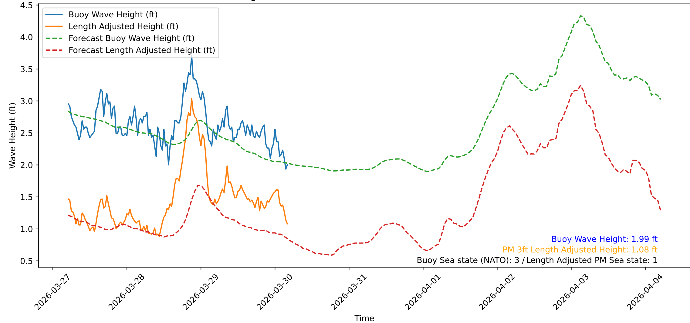
Wave Heights over Time for Green Beach at 2026-03-30 04:51:09
