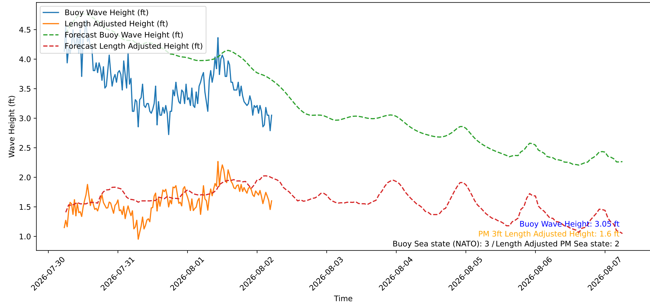
Wave Heights over Time for Oceanside Harbor at 2026-08-02 05:30:26
