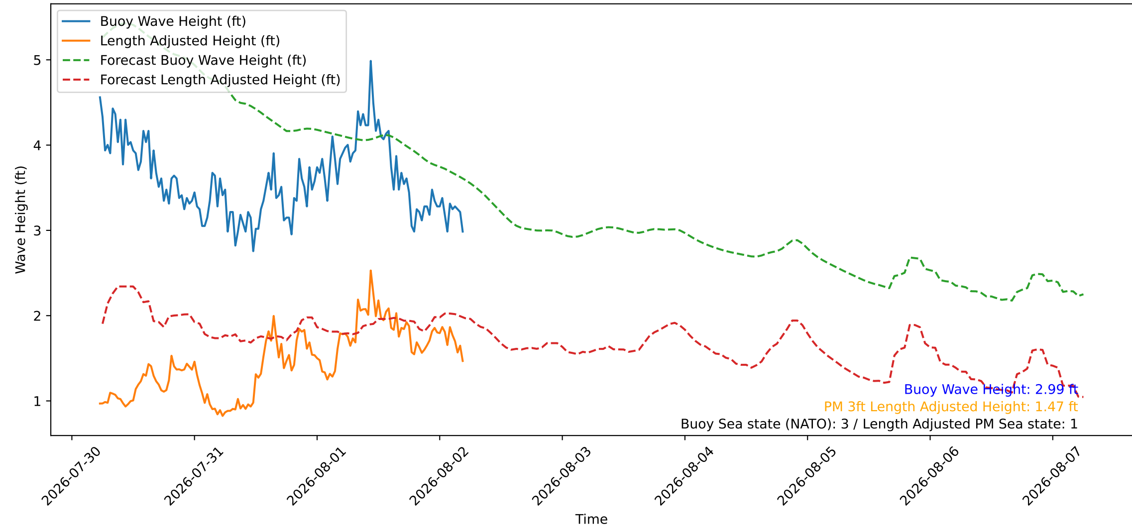
Wave Heights over Time for Green Beach at 2026-08-02 05:31:08
