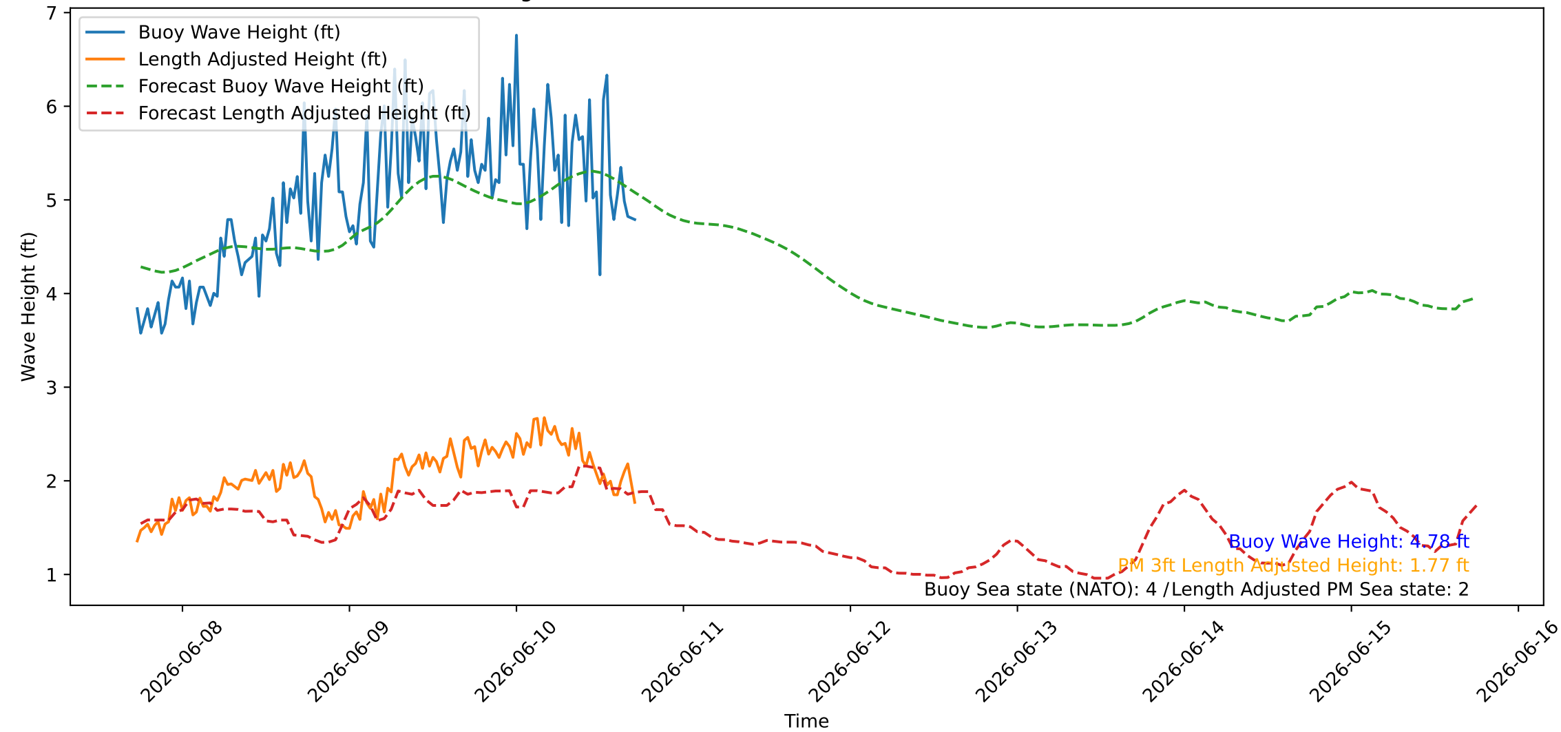
Wave Heights over Time for Oceanside Harbor at 2026-06-10 17:30:27
