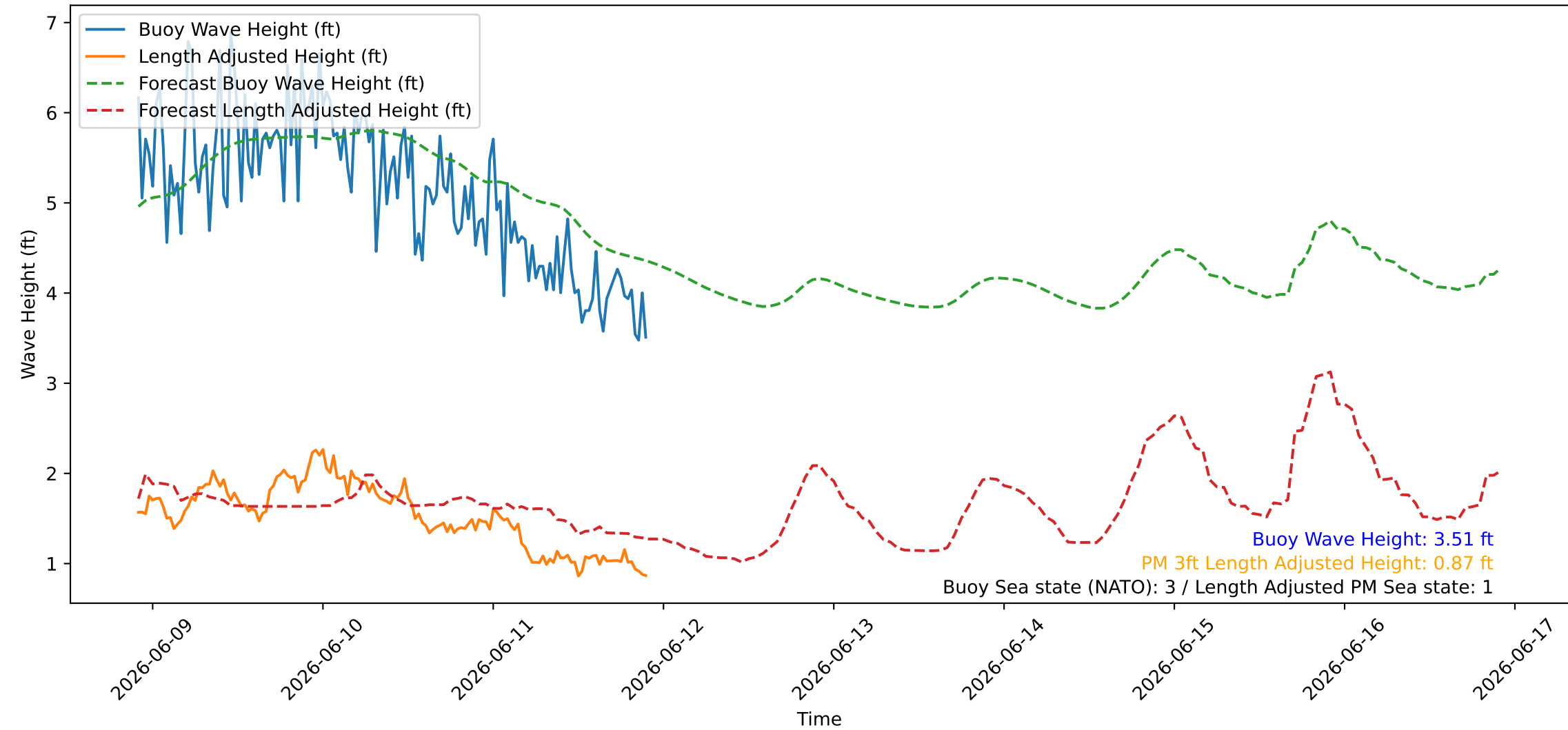
Wave Heights over Time for Green Beach at 2026-06-11 22:11:08
