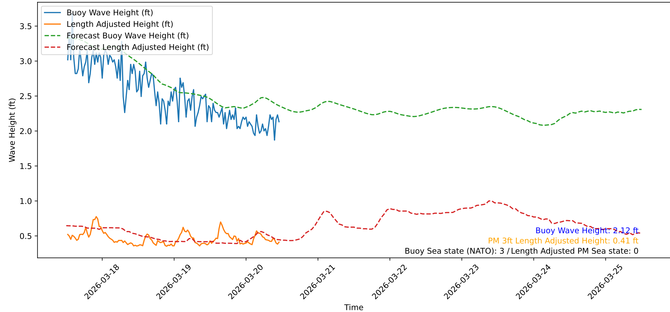
Wave Heights over Time for Red Beach at 2026-03-20 12:00:48
