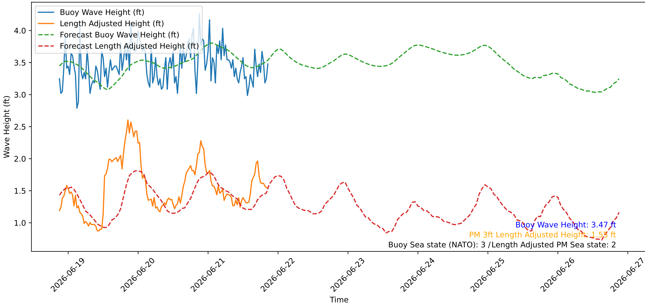
Wave Heights over Time for Oceanside Harbor at 2026-06-21 21:10:26
