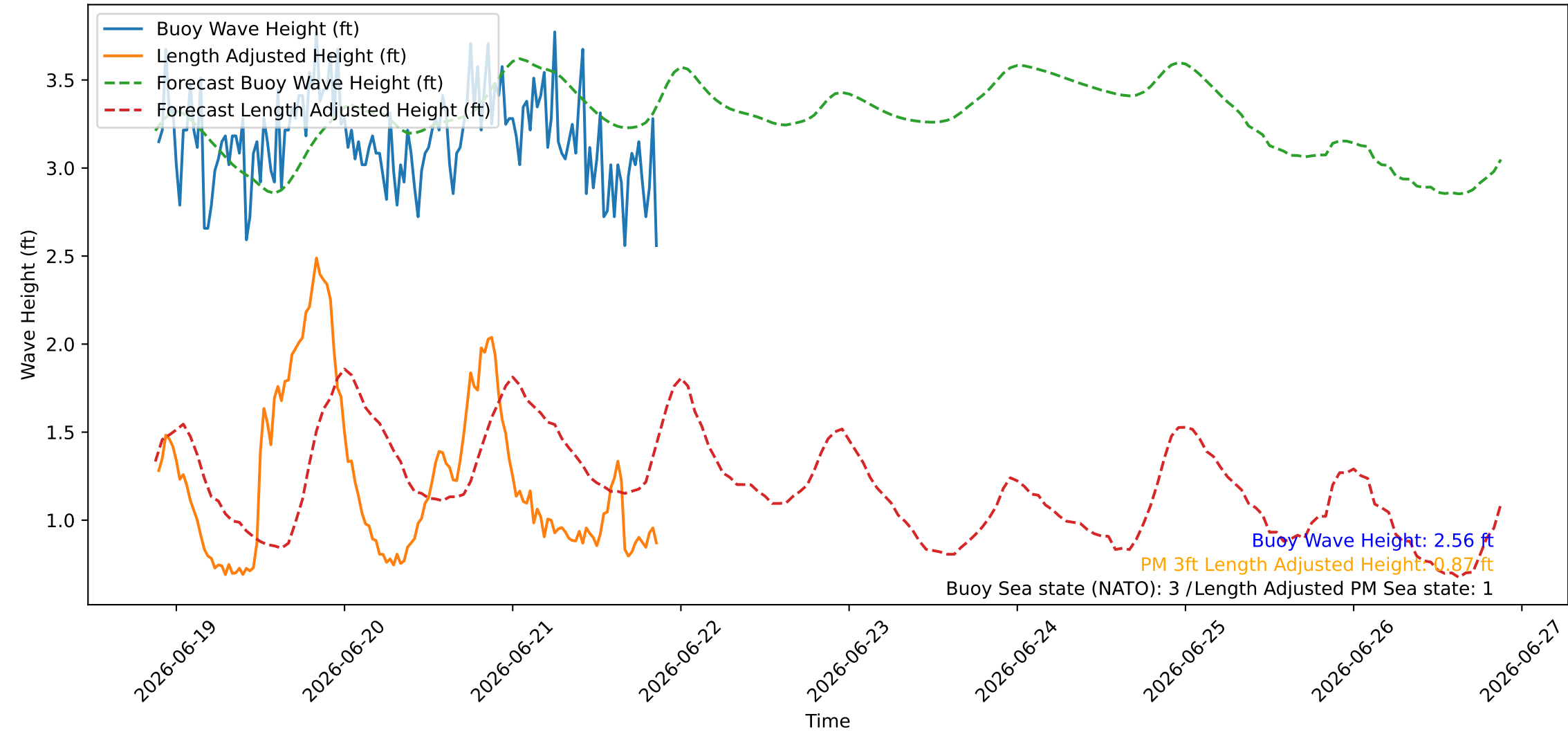
Wave Heights over Time for Red Beach at 2026-06-21 21:10:45
