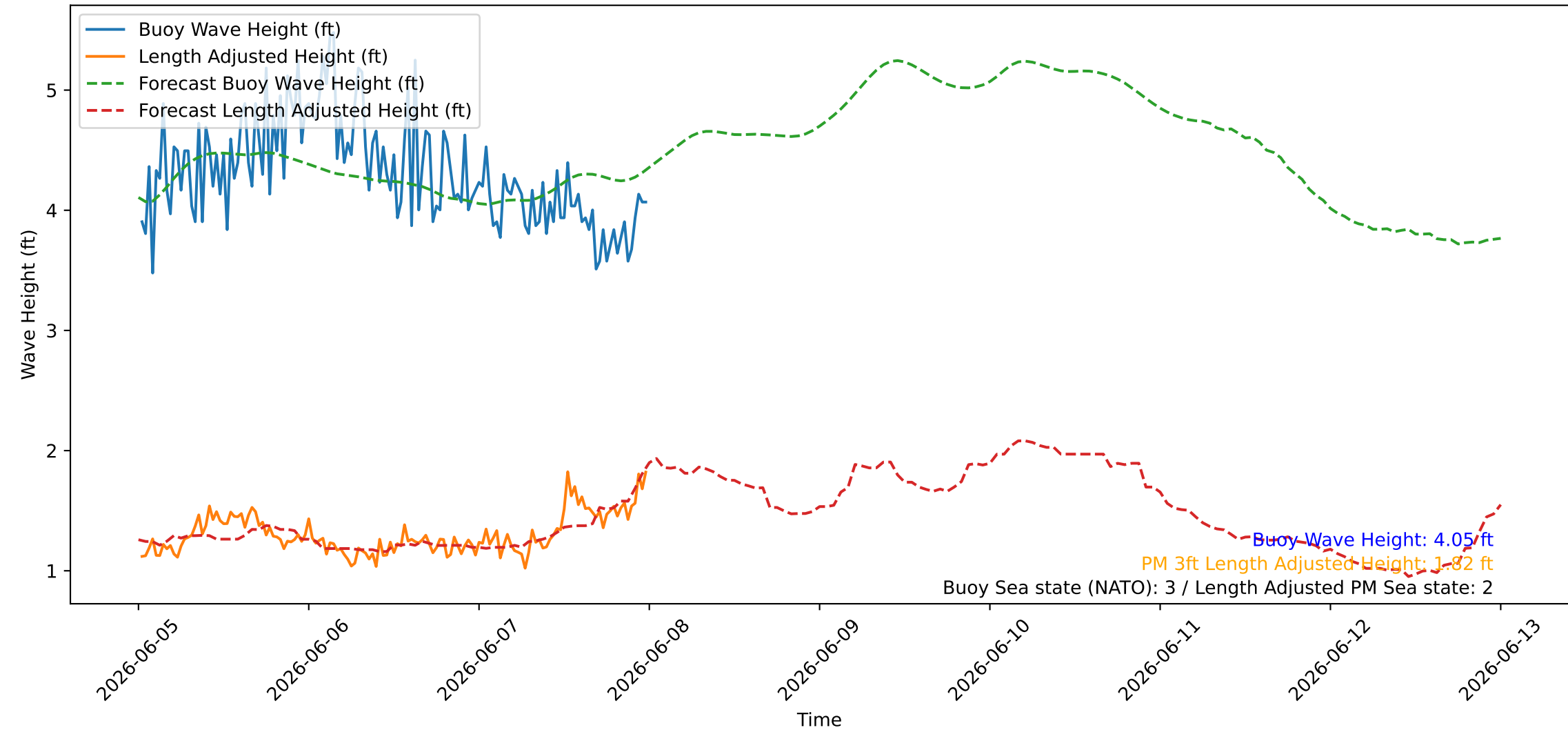
Wave Heights over Time for Oceanside Harbor at 2026-06-08 00:20:26
