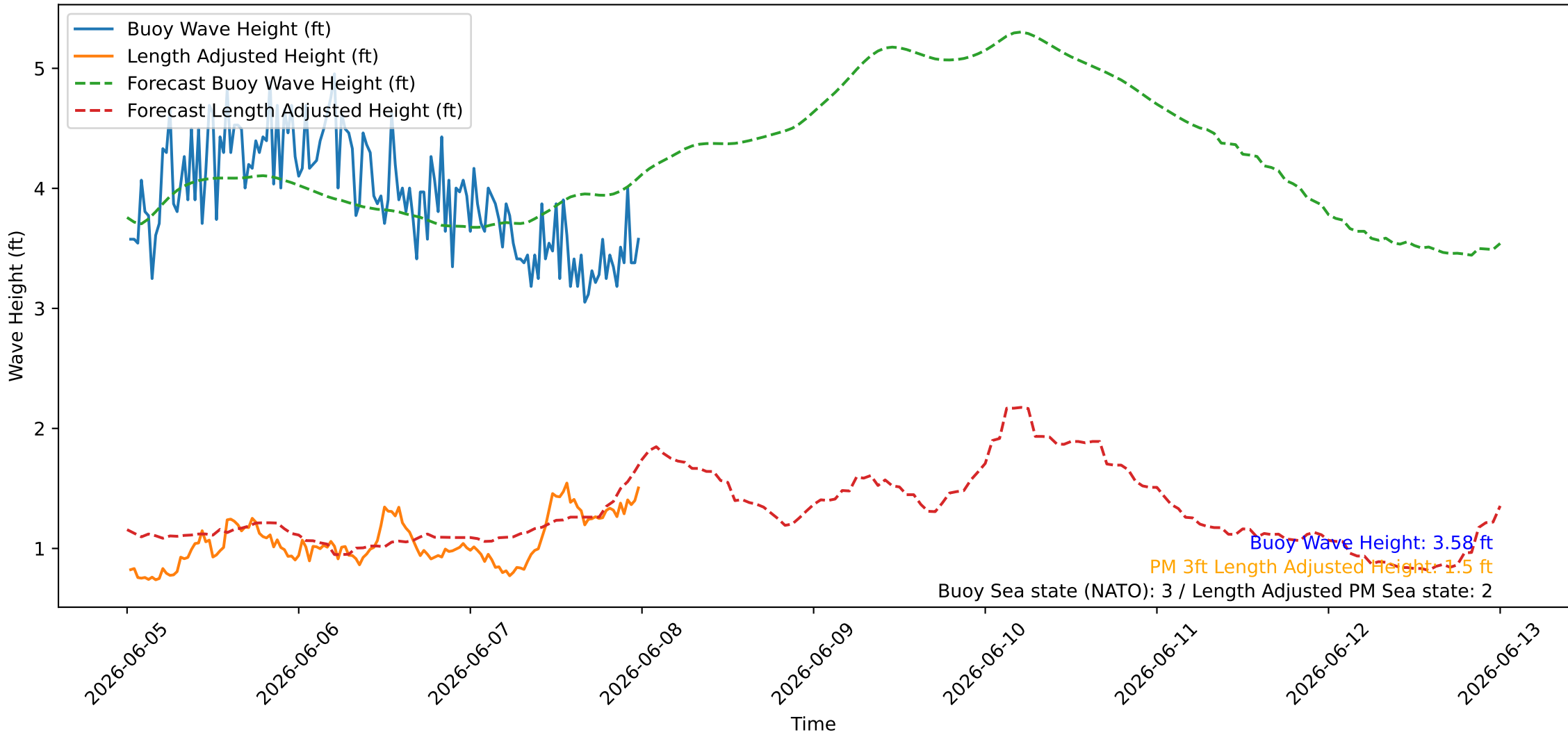
Wave Heights over Time for Red Beach at 2026-06-08 00:20:46
