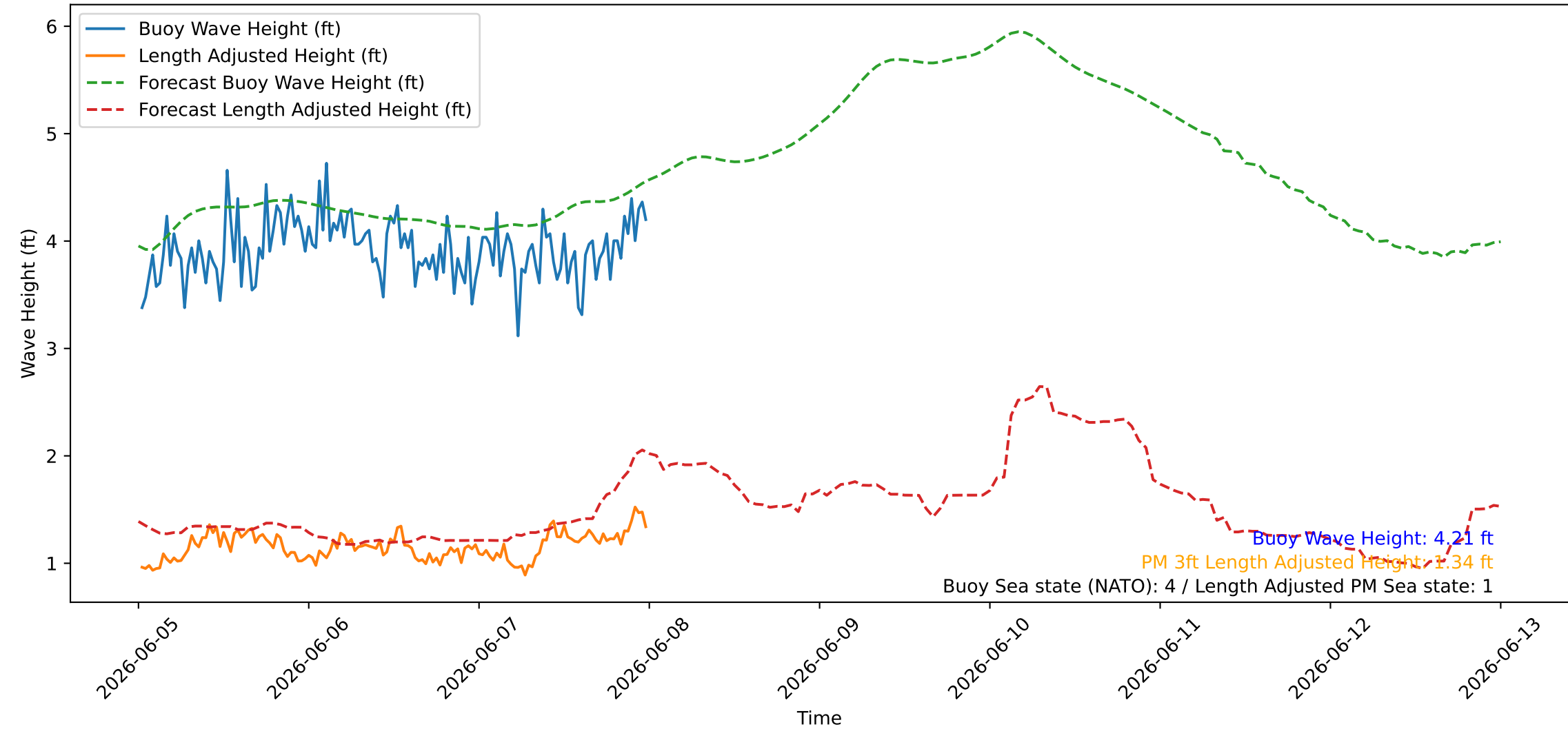
Wave Heights over Time for Green Beach at 2026-06-08 00:21:10
