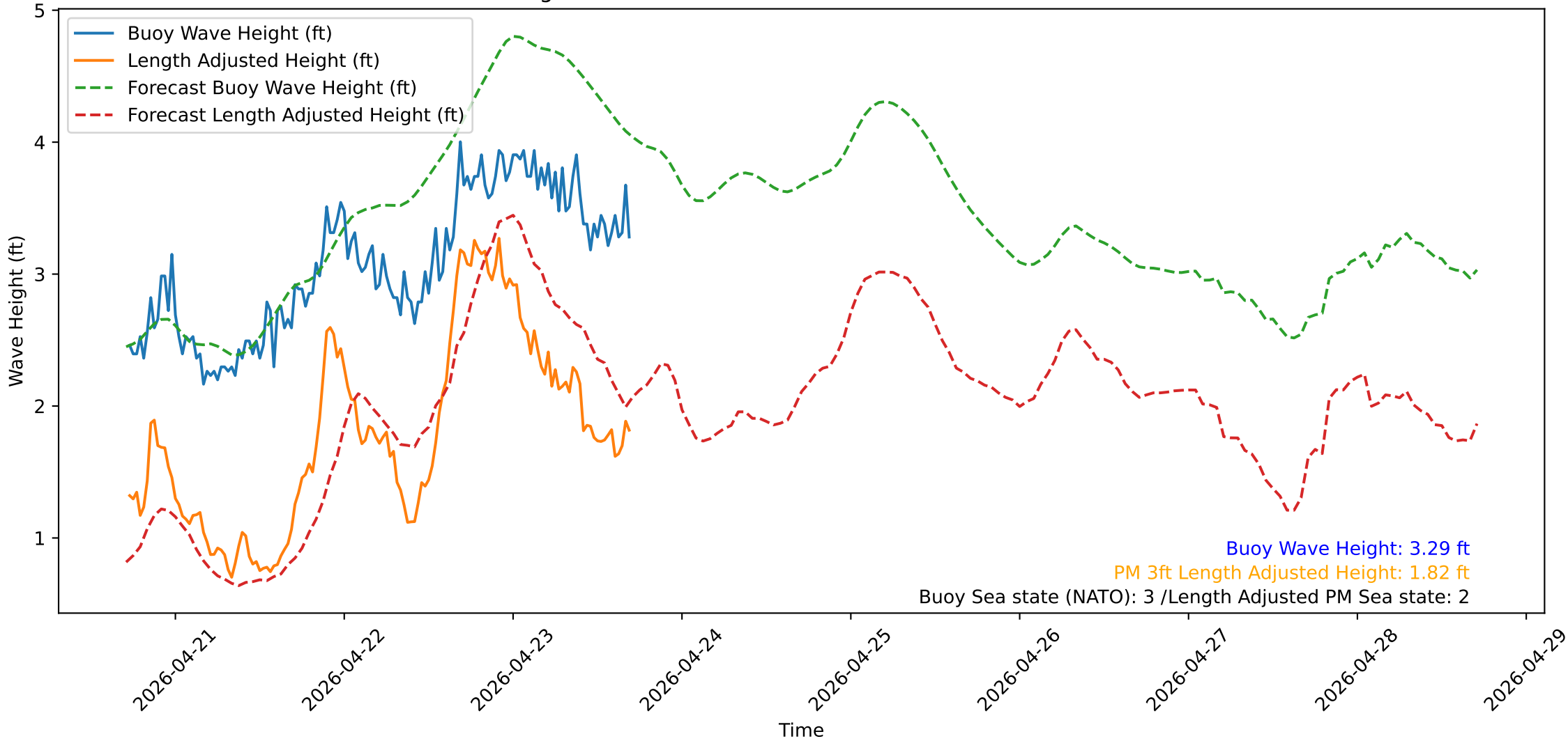
Wave Heights over Time for Green Beach at 2026-04-23 17:21:13
