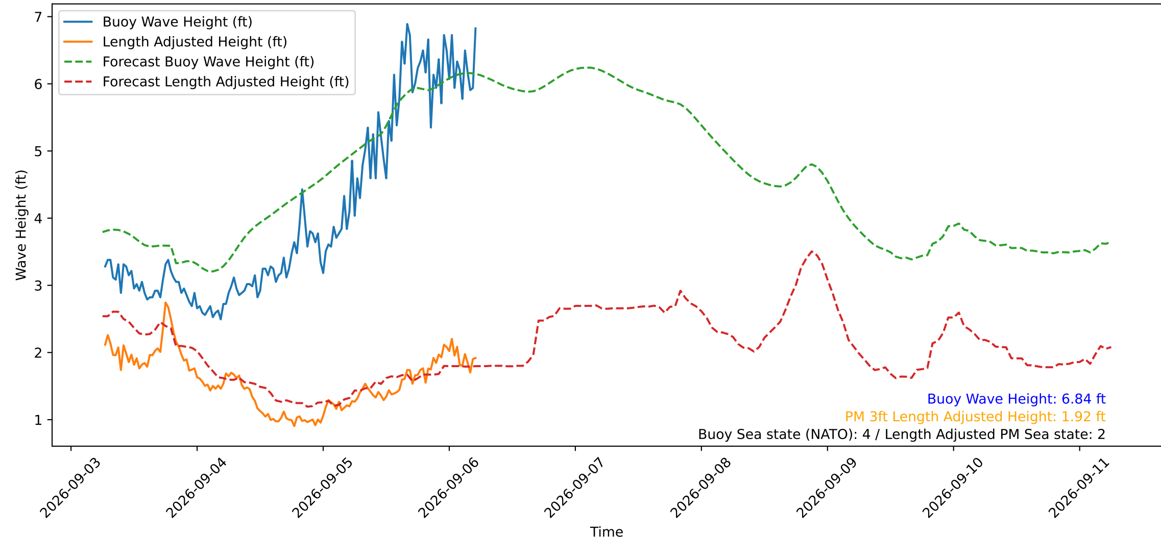
Wave Heights over Time for Green Beach at 2026-09-06 06:01:13
