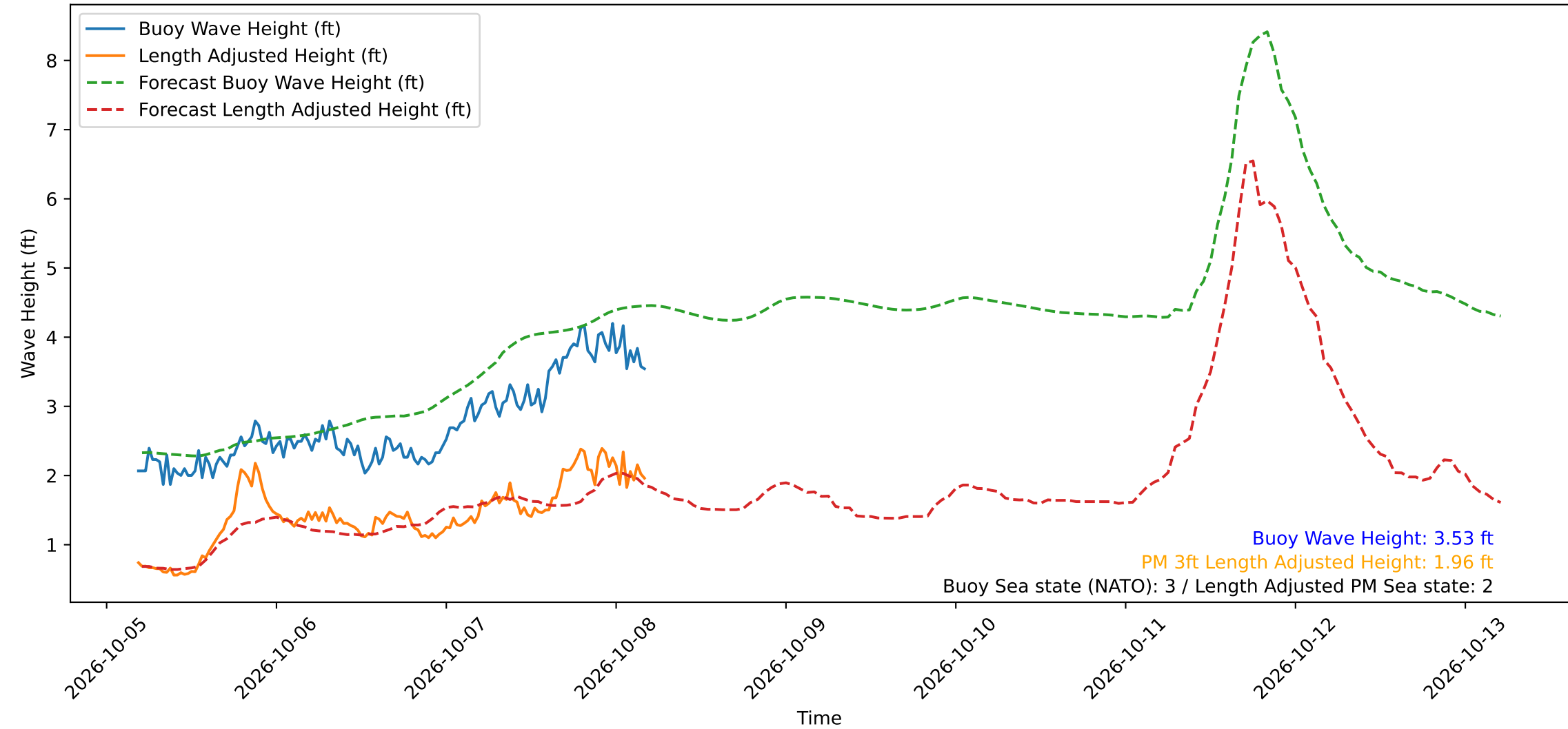
Wave Heights over Time for Oceanside Harbor at 2026-10-08 04:40:29
