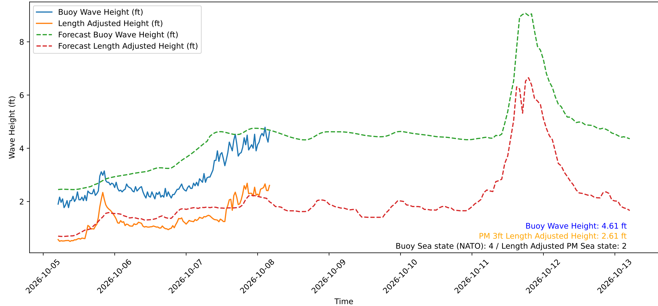
Wave Heights over Time for Green Beach at 2026-10-08 04:41:11
