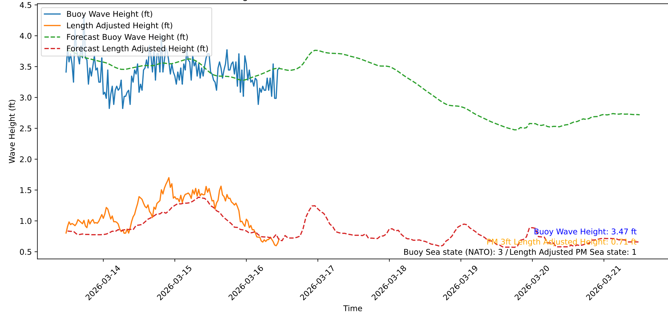
Wave Heights over Time for Green Beach at 2026-03-16 11:42:03
