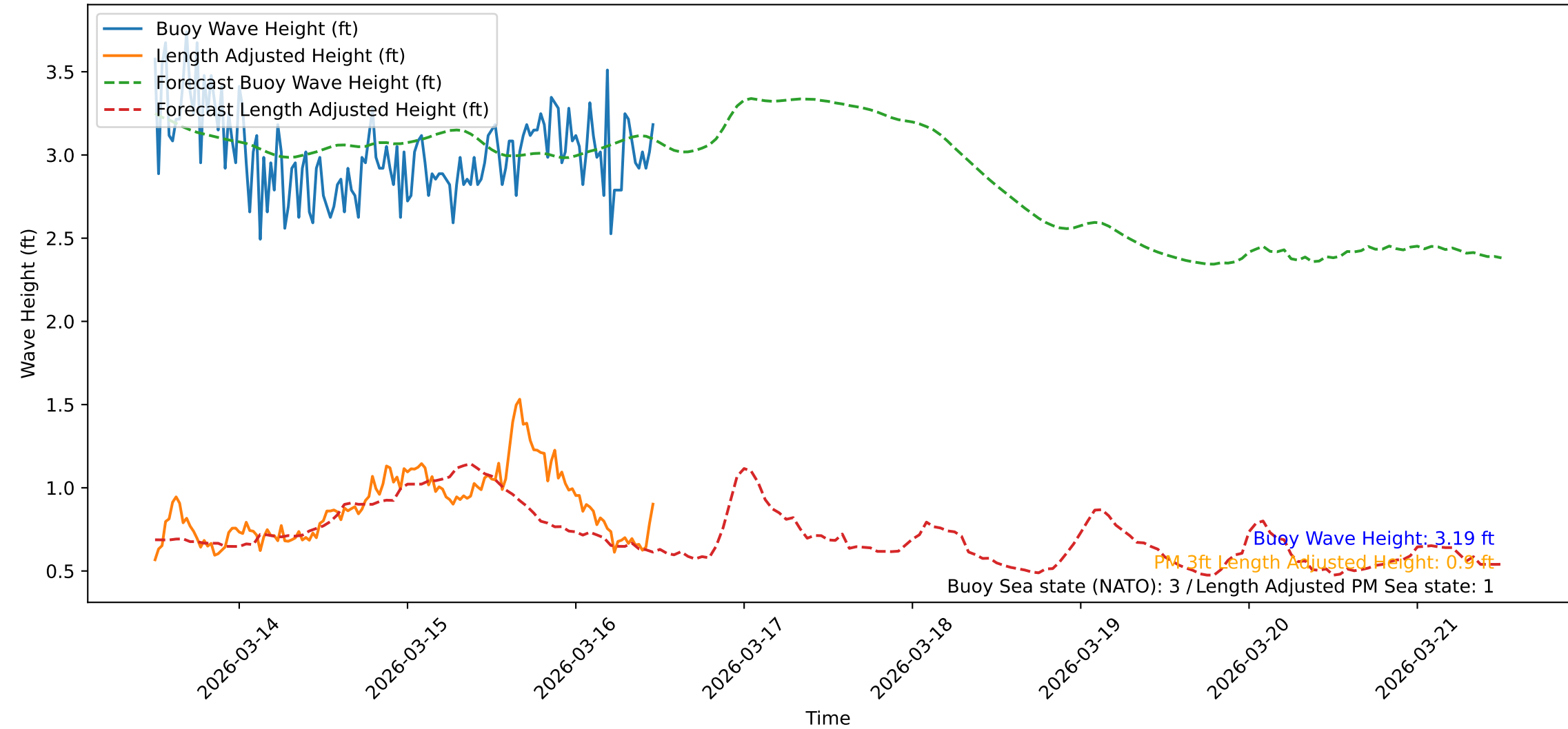
Wave Heights over Time for Red Beach at 2026-03-16 11:41:28
