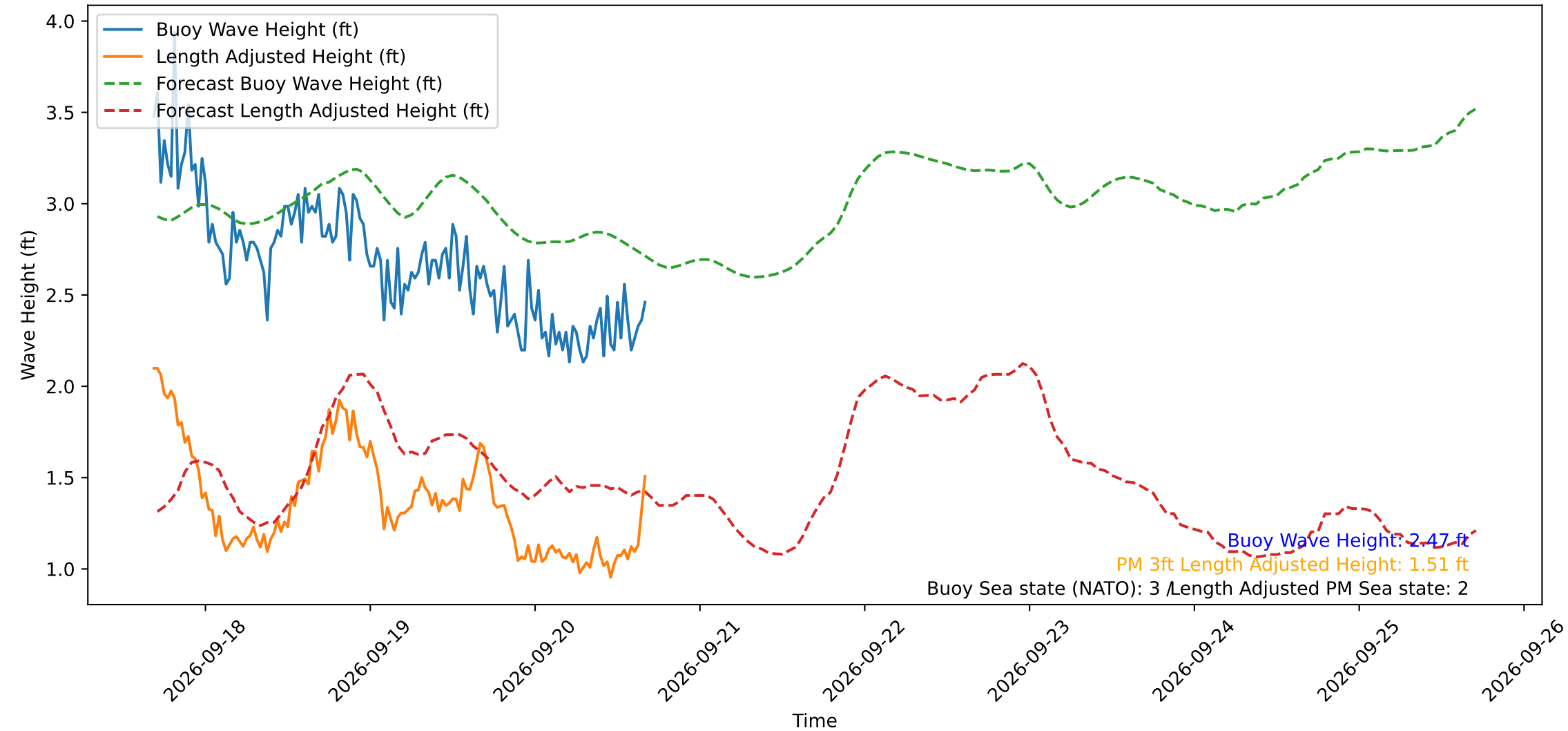
Wave Heights over Time for Oceanside Harbor at 2026-09-20 16:40:30
