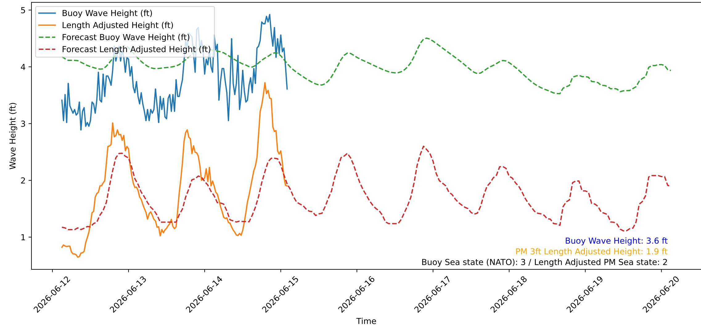
Wave Heights over Time for Green Beach at 2026-06-15 02:51:09
