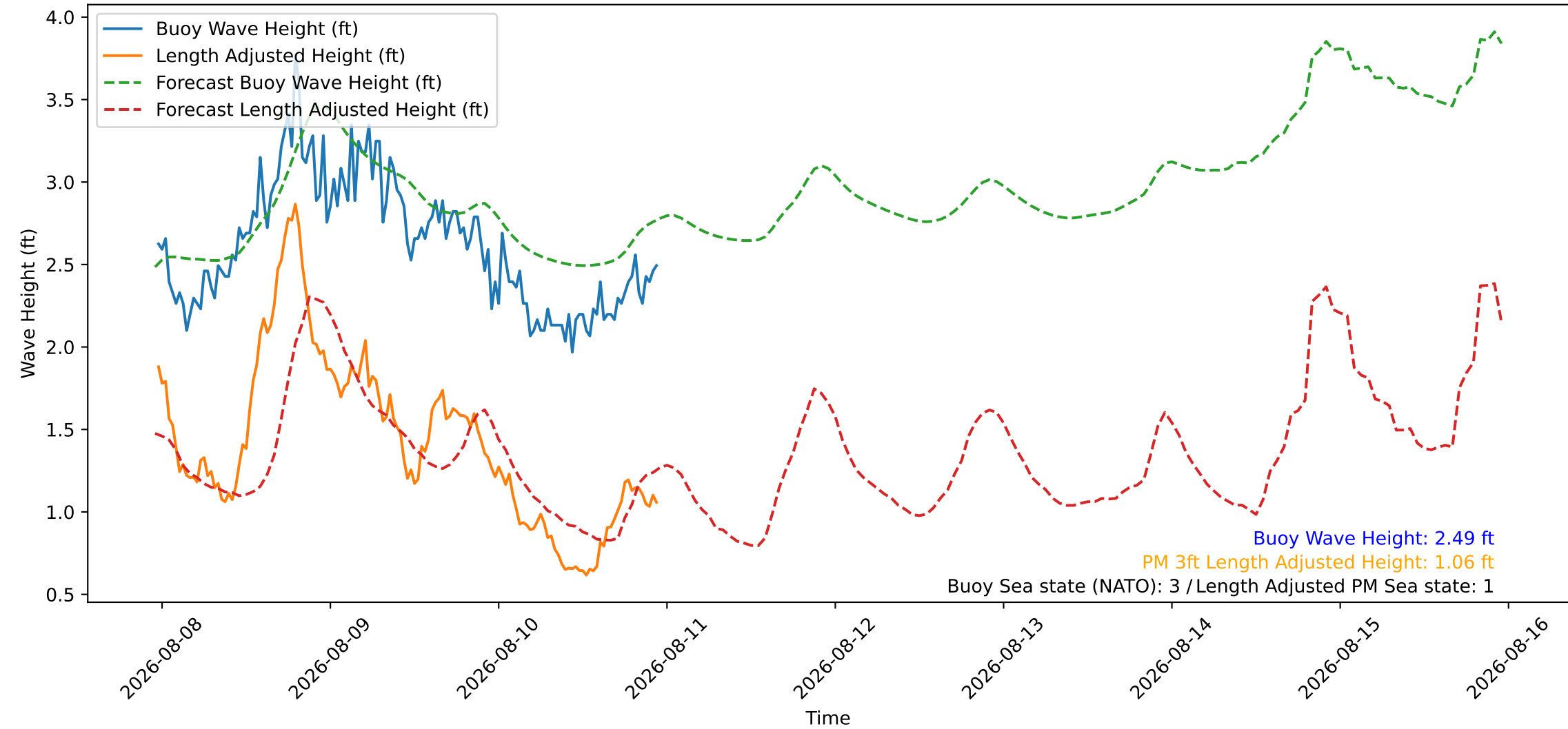
Wave Heights over Time for Green Beach at 2026-08-10 23:21:10
