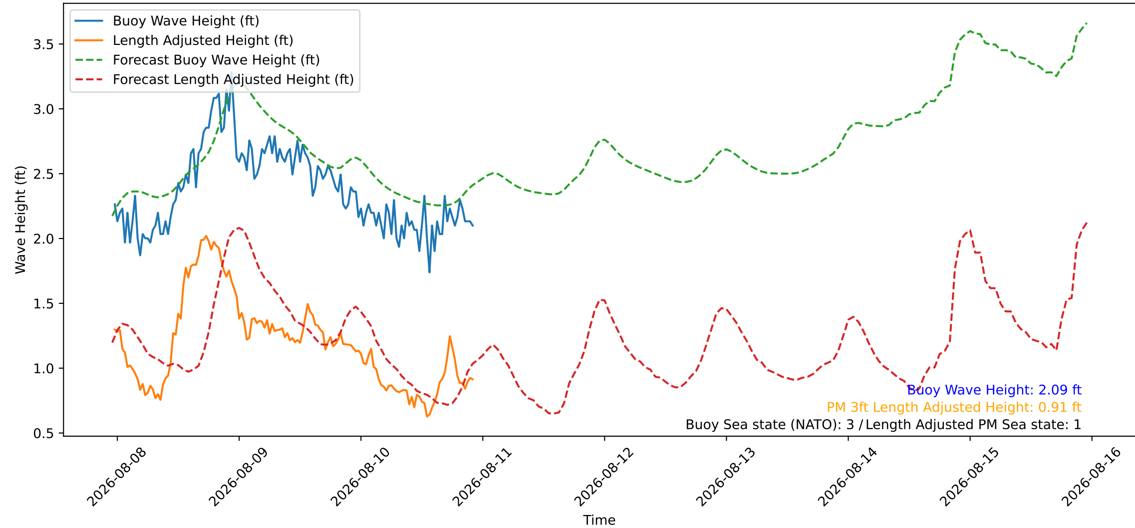
Wave Heights over Time for Red Beach at 2026-08-10 23:20:47
