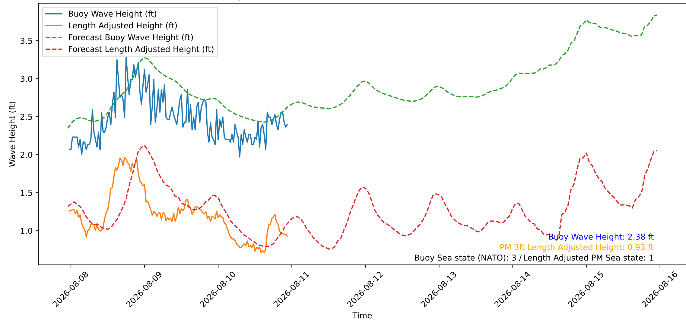
Wave Heights over Time for Oceanside Harbor at 2026-08-10 23:20:26
