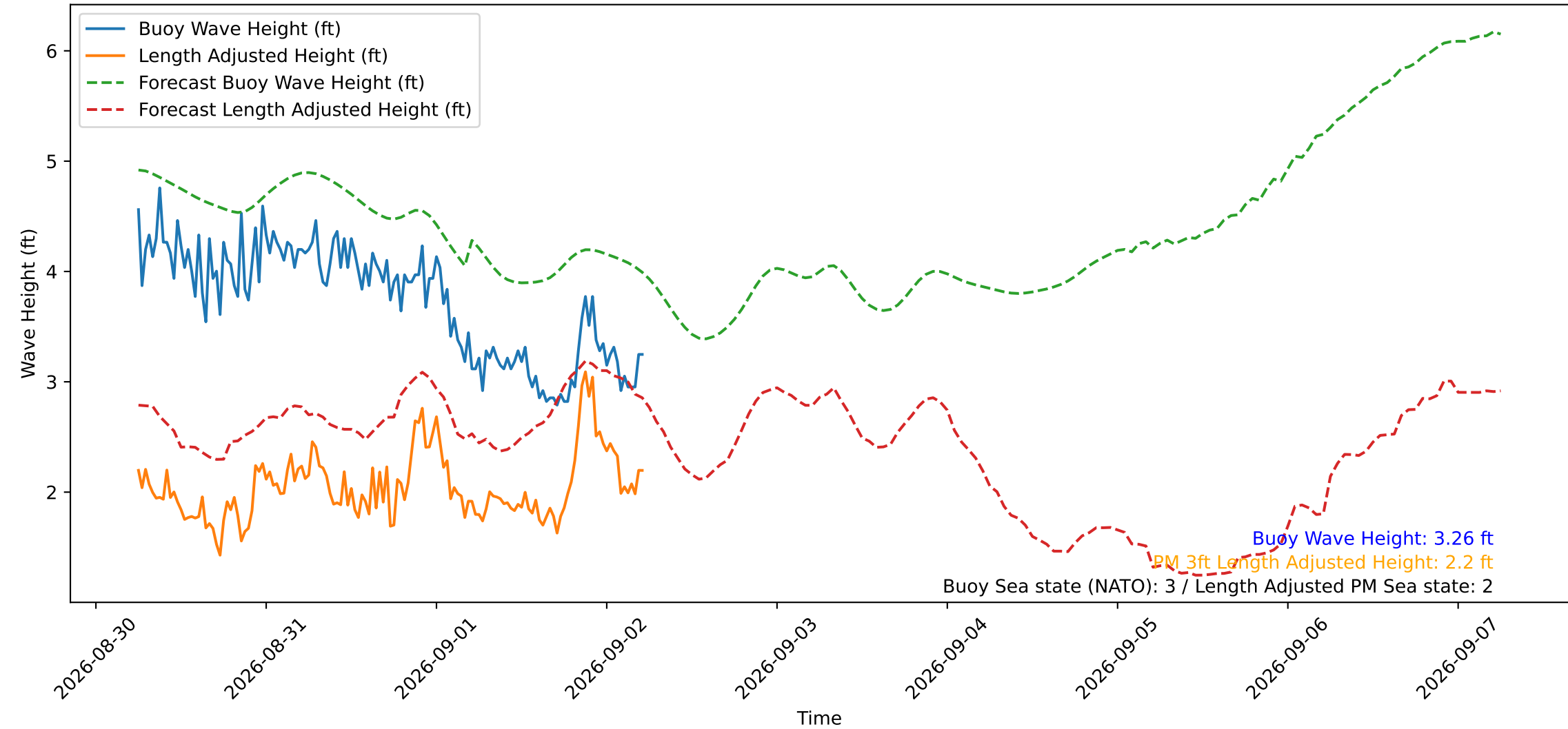
Wave Heights over Time for Green Beach at 2026-09-02 05:51:15
