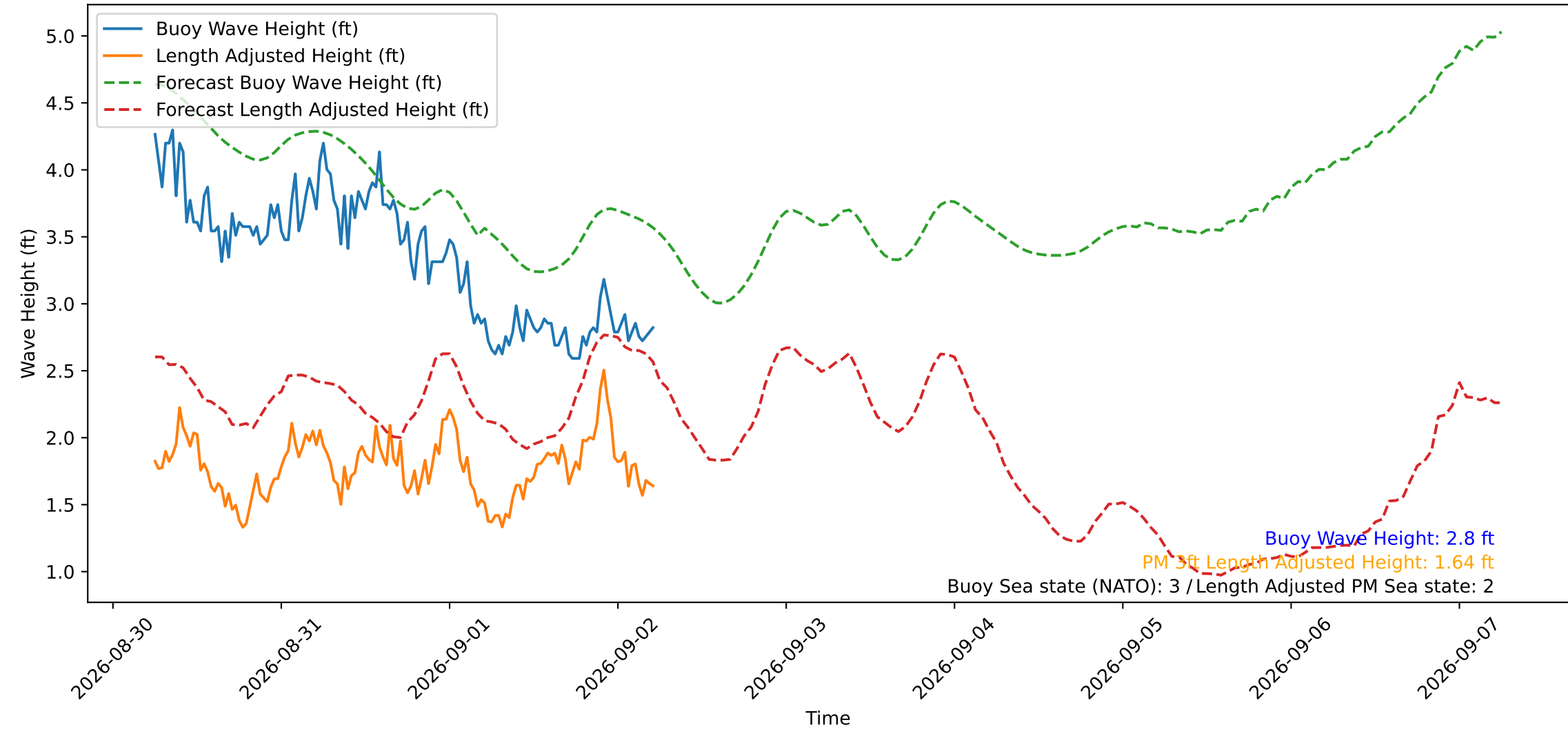
Wave Heights over Time for Red Beach at 2026-09-02 05:50:51
