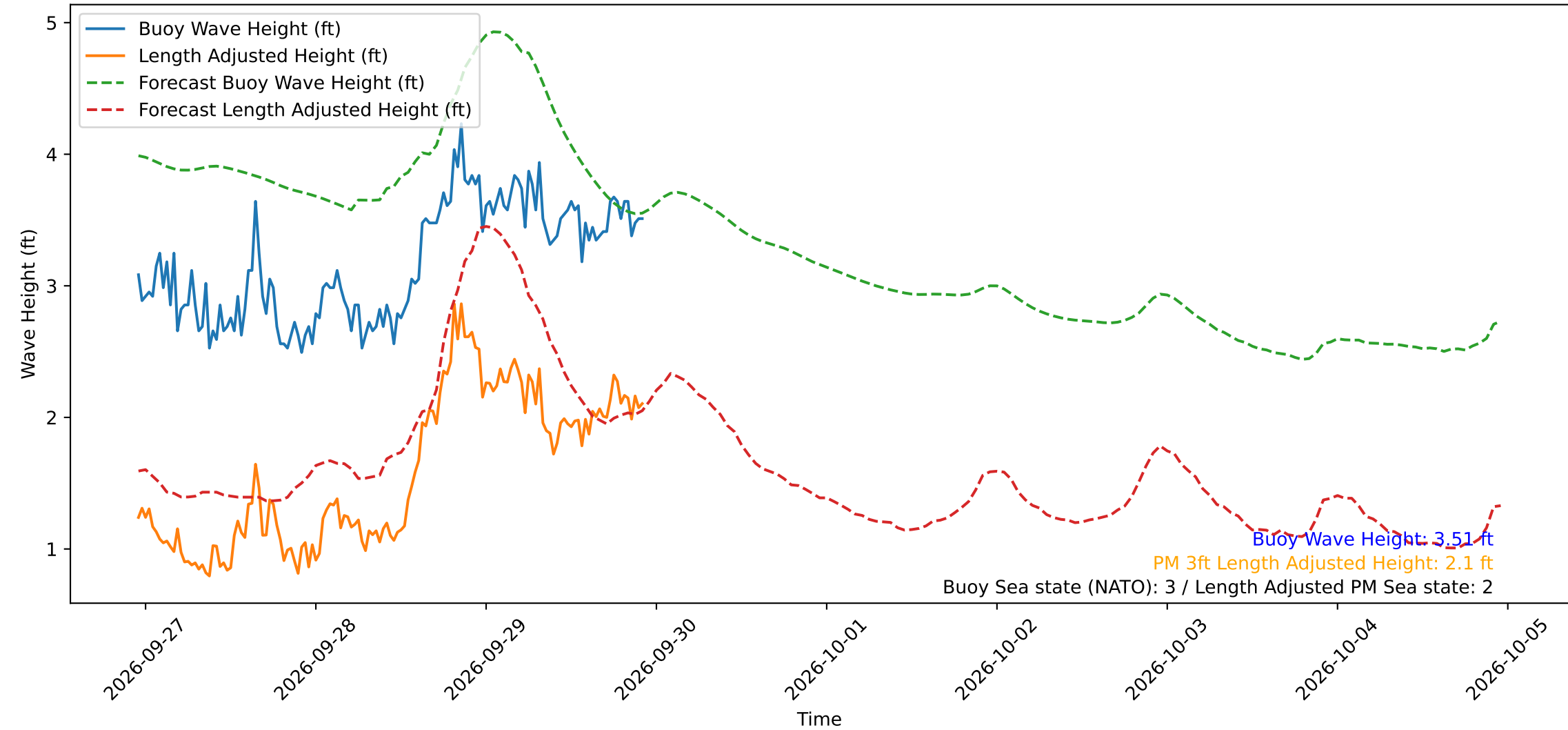
Wave Heights over Time for Oceanside Harbor at 2026-09-29 22:50:30
