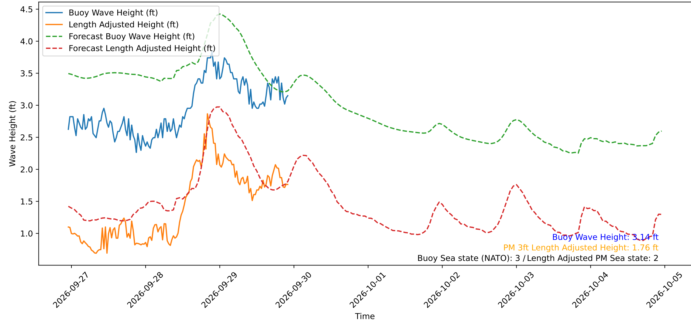
Wave Heights over Time for Red Beach at 2026-09-29 22:50:50
