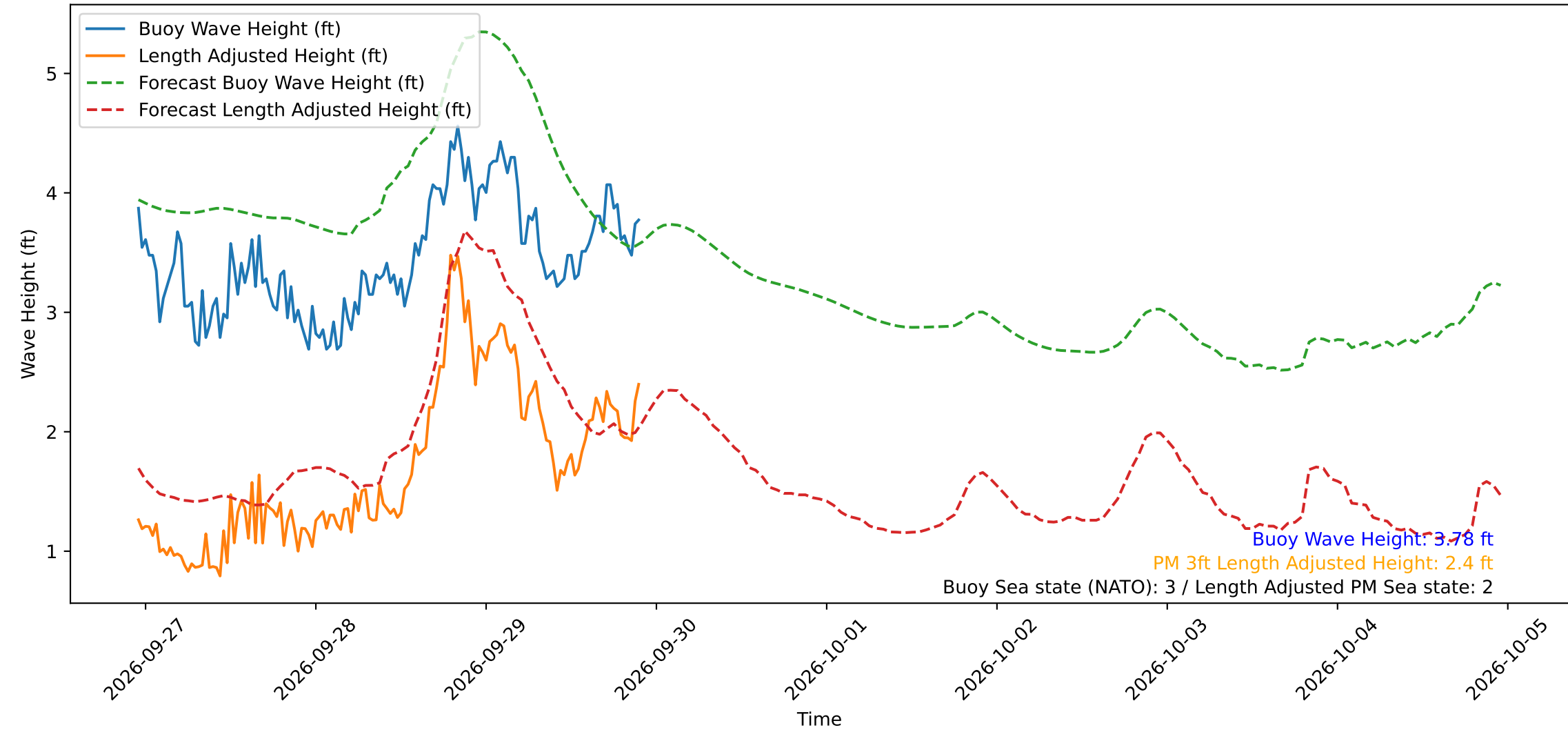
Wave Heights over Time for Green Beach at 2026-09-29 22:51:14
