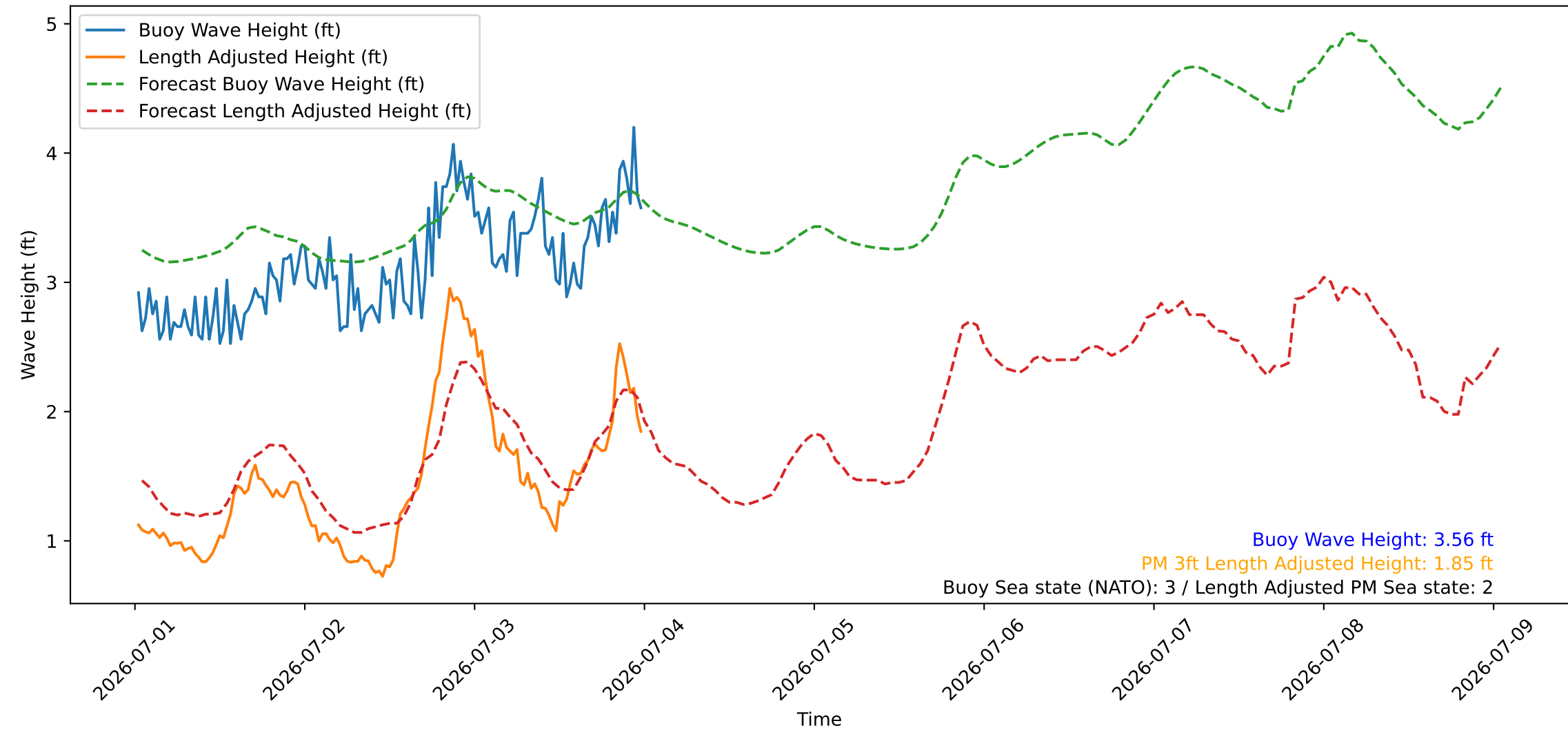
Wave Heights over Time for Green Beach at 2026-07-04 00:31:07
