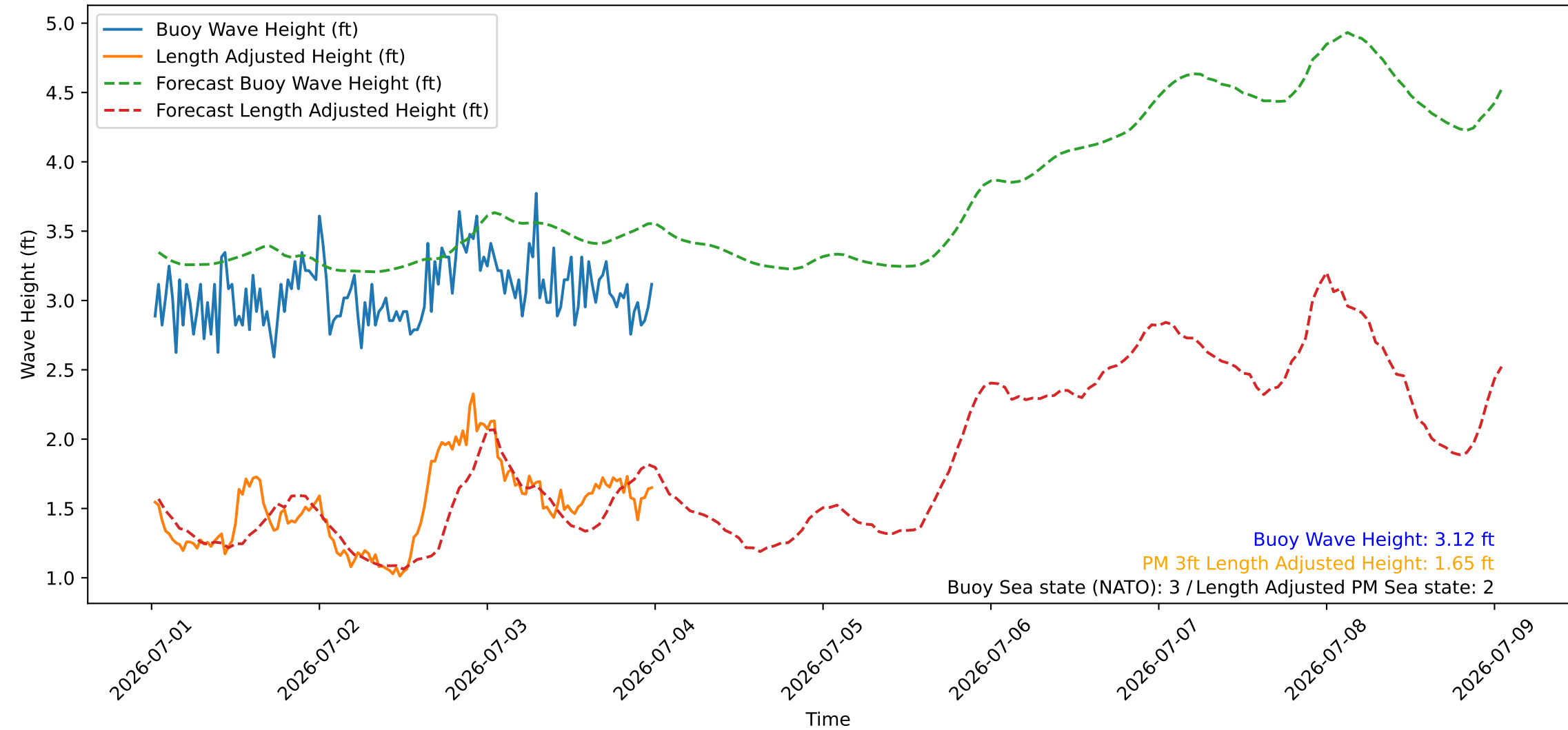
Wave Heights over Time for Oceanside Harbor at 2026-07-04 00:30:26
