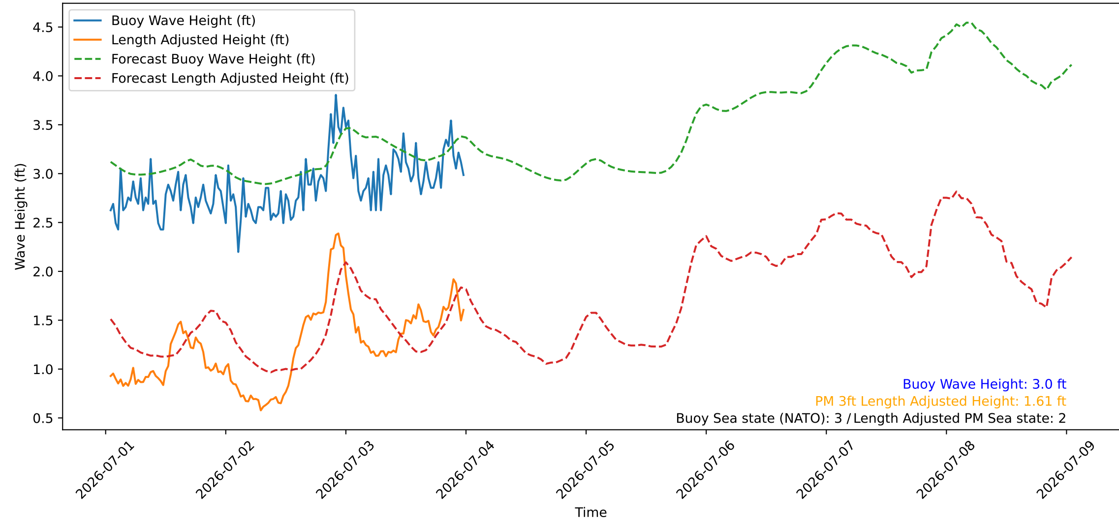
Wave Heights over Time for Red Beach at 2026-07-04 00:30:45
