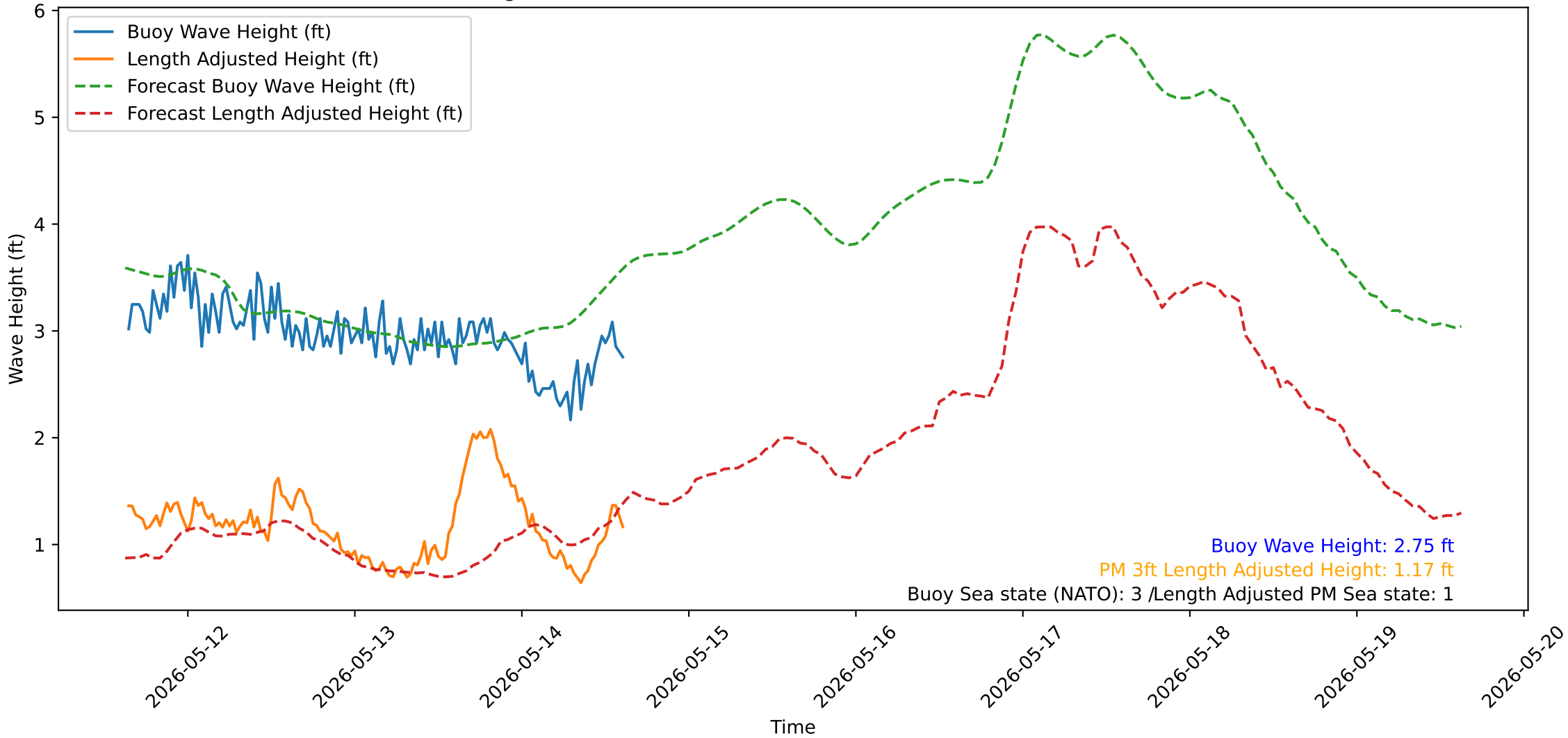
Wave Heights over Time for Oceanside Harbor at 2026-05-14 15:20:33
