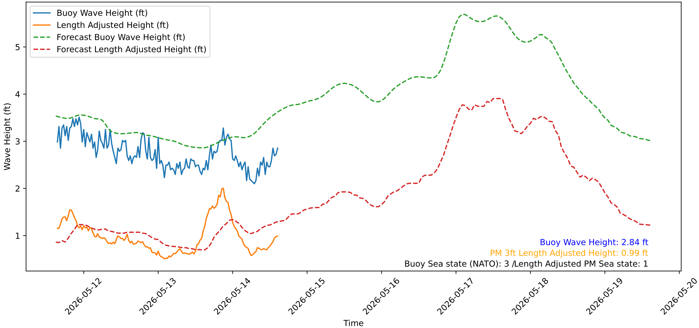
Wave Heights over Time for Green Beach at 2026-05-14 15:21:17
