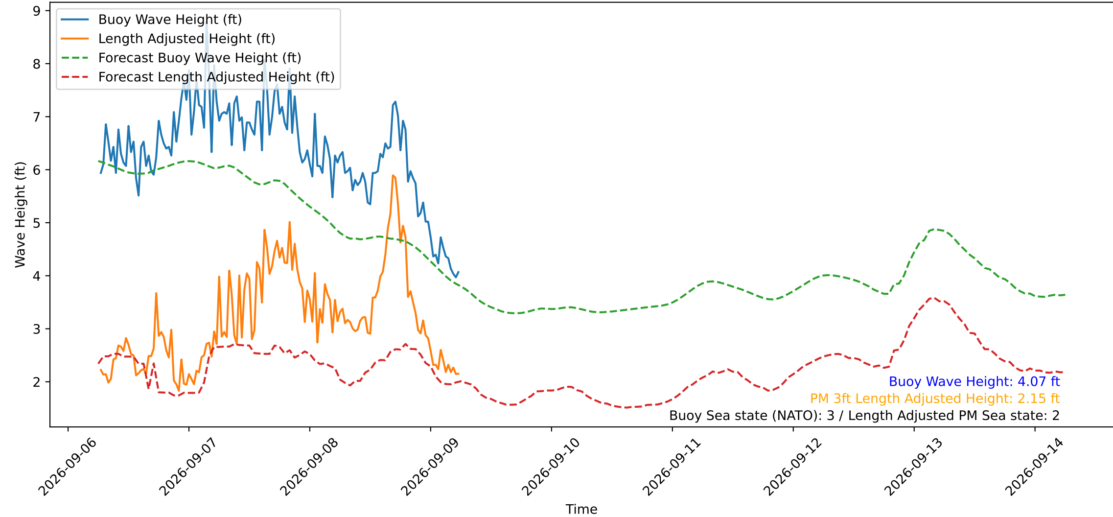
Wave Heights over Time for Green Beach at 2026-09-09 06:21:14
