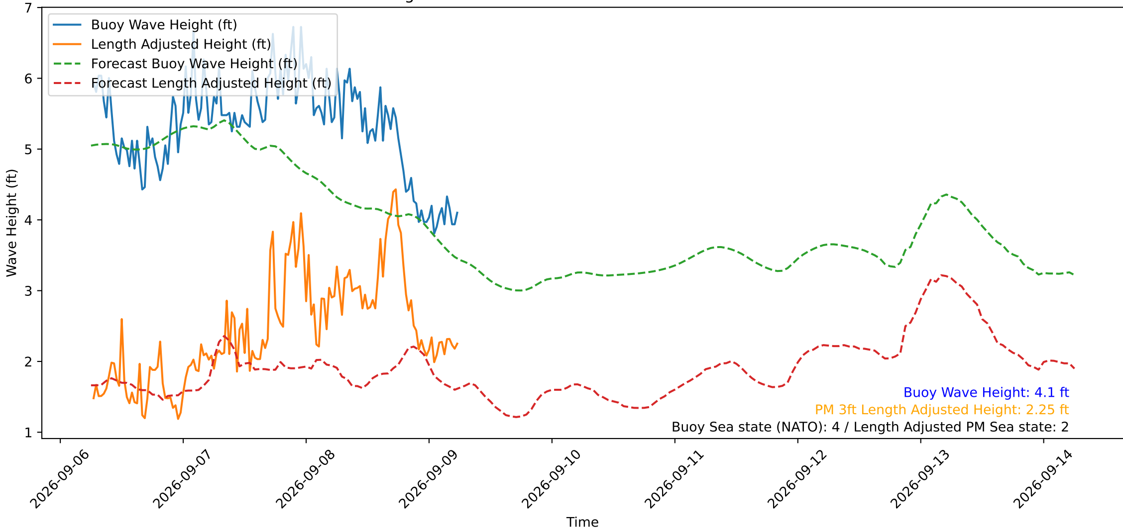
Wave Heights over Time for Red Beach at 2026-09-09 06:20:50
