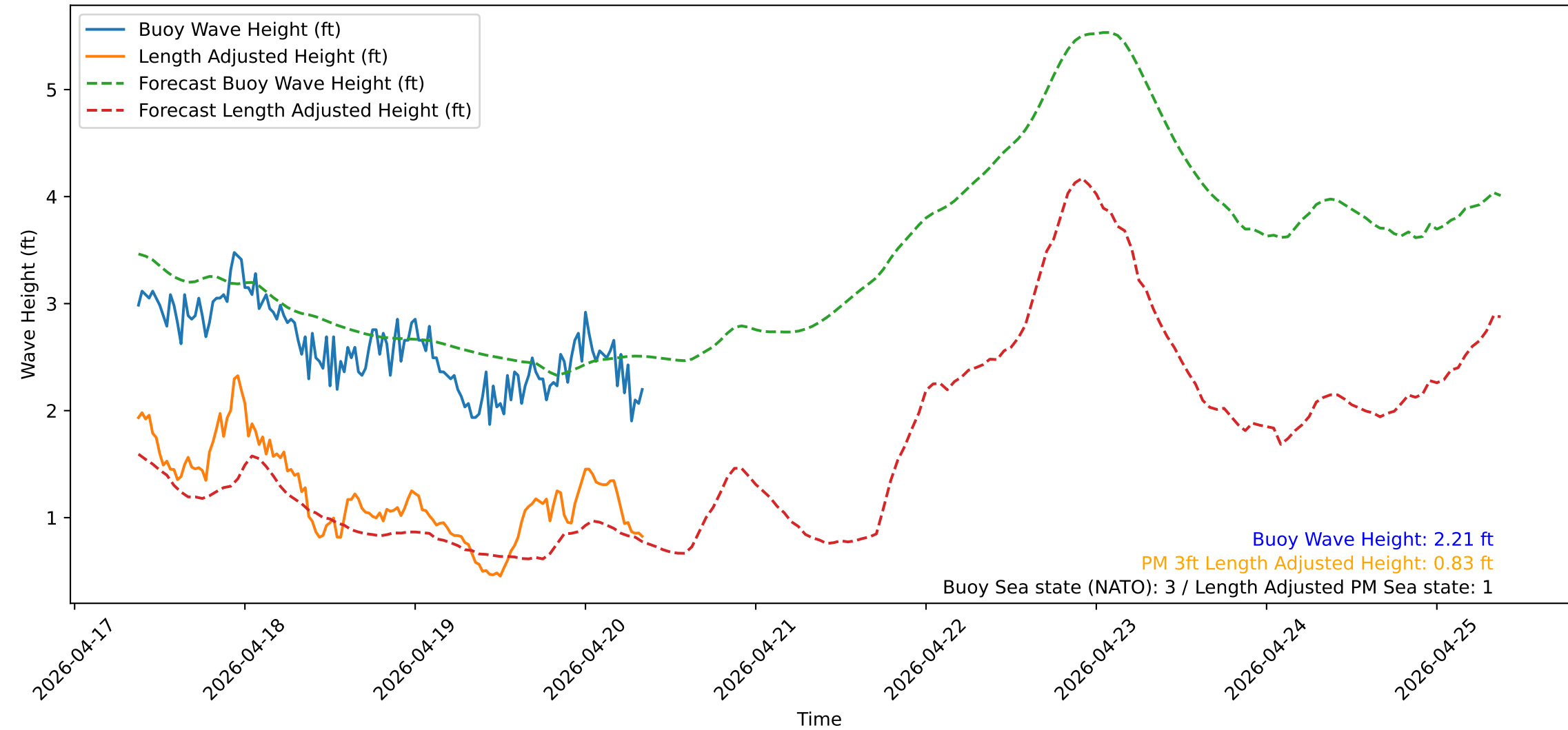
Wave Heights over Time for Green Beach at 2026-04-20 08:51:13
