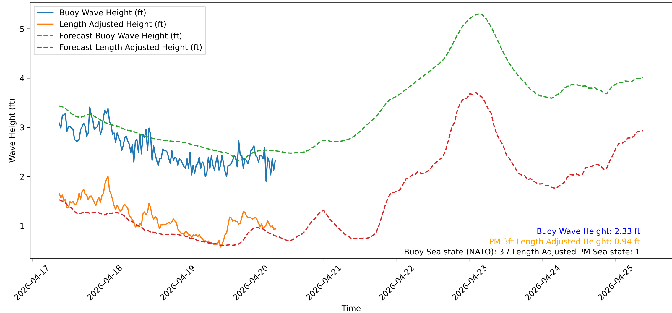
Wave Heights over Time for Oceanside Harbor at 2026-04-20 08:50:31
