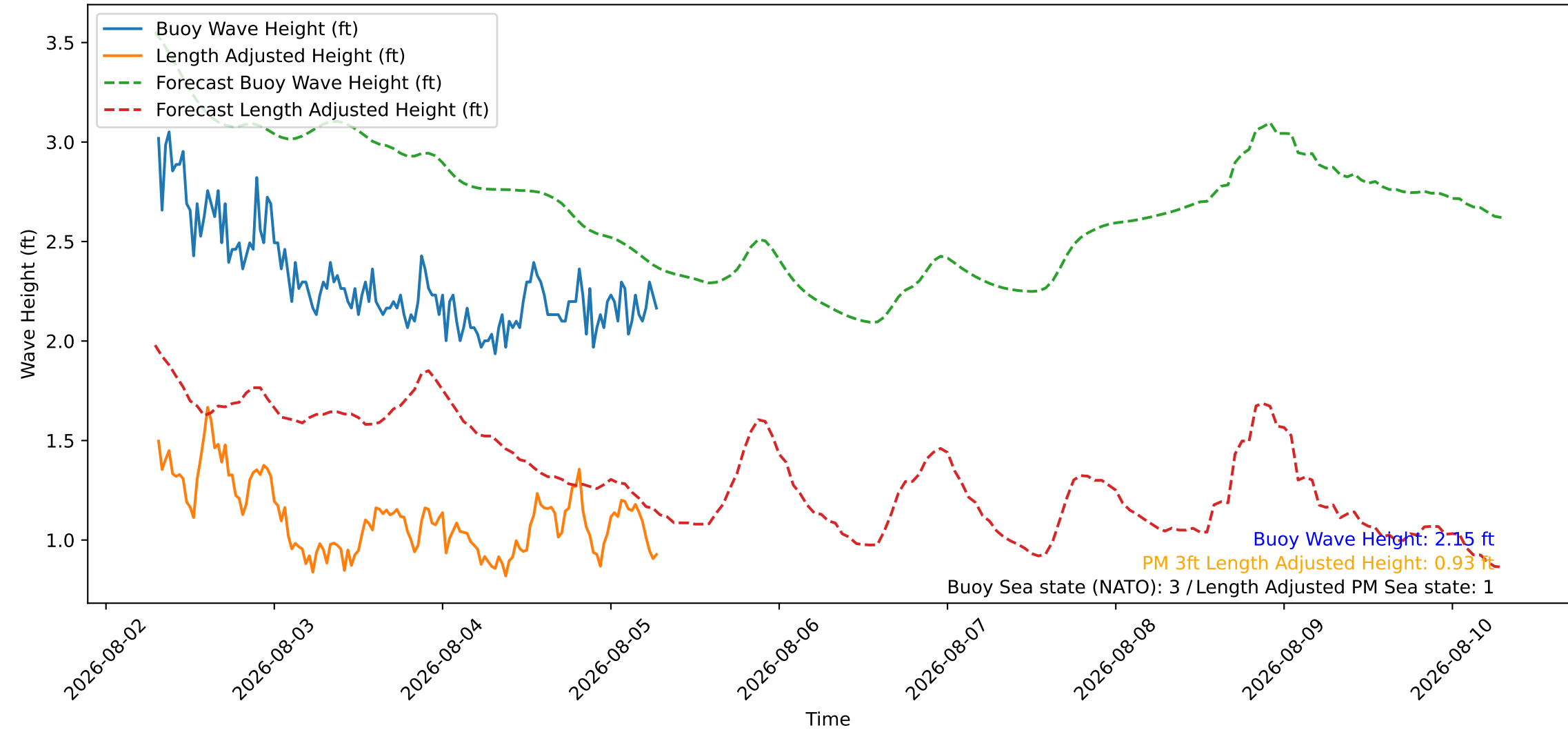
Wave Heights over Time for Green Beach at 2026-08-05 07:21:10
