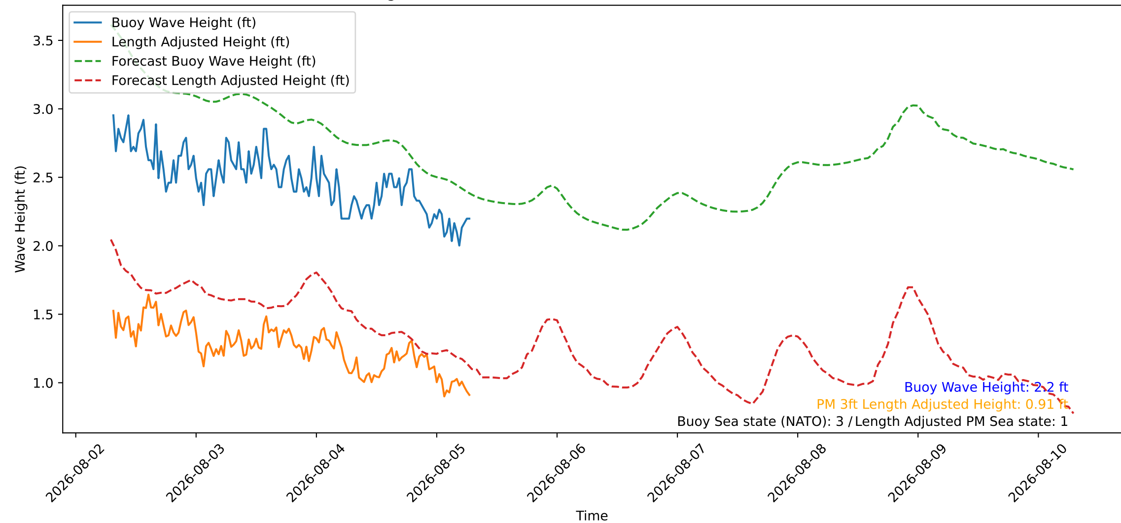
Wave Heights over Time for Oceanside Harbor at 2026-08-05 07:20:26
