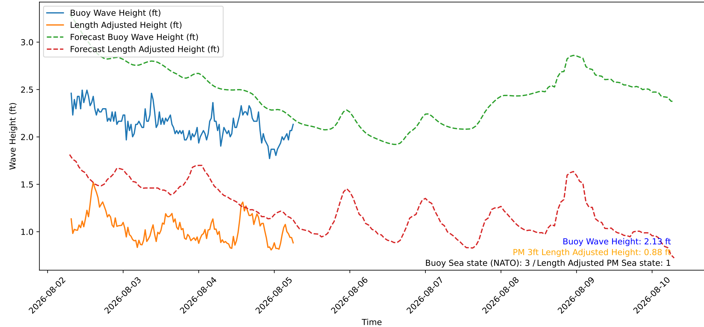
Wave Heights over Time for Red Beach at 2026-08-05 07:20:47
