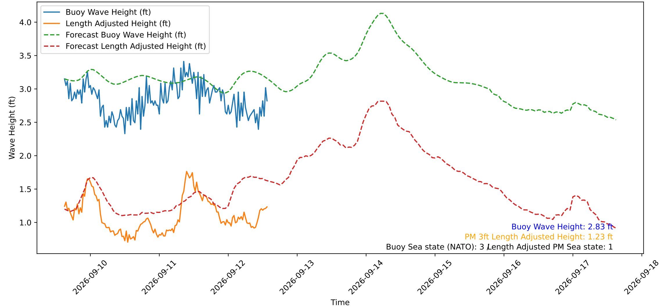
Wave Heights over Time for Red Beach at 2026-09-12 14:40:49
