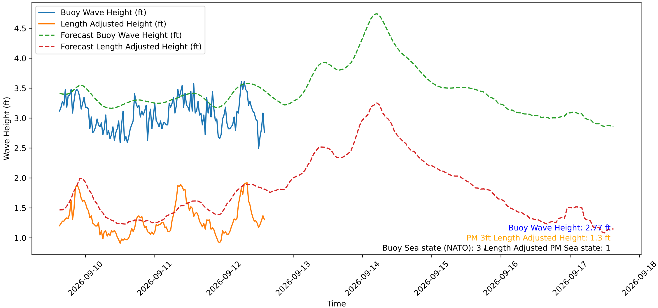
Wave Heights over Time for Green Beach at 2026-09-12 14:41:12
