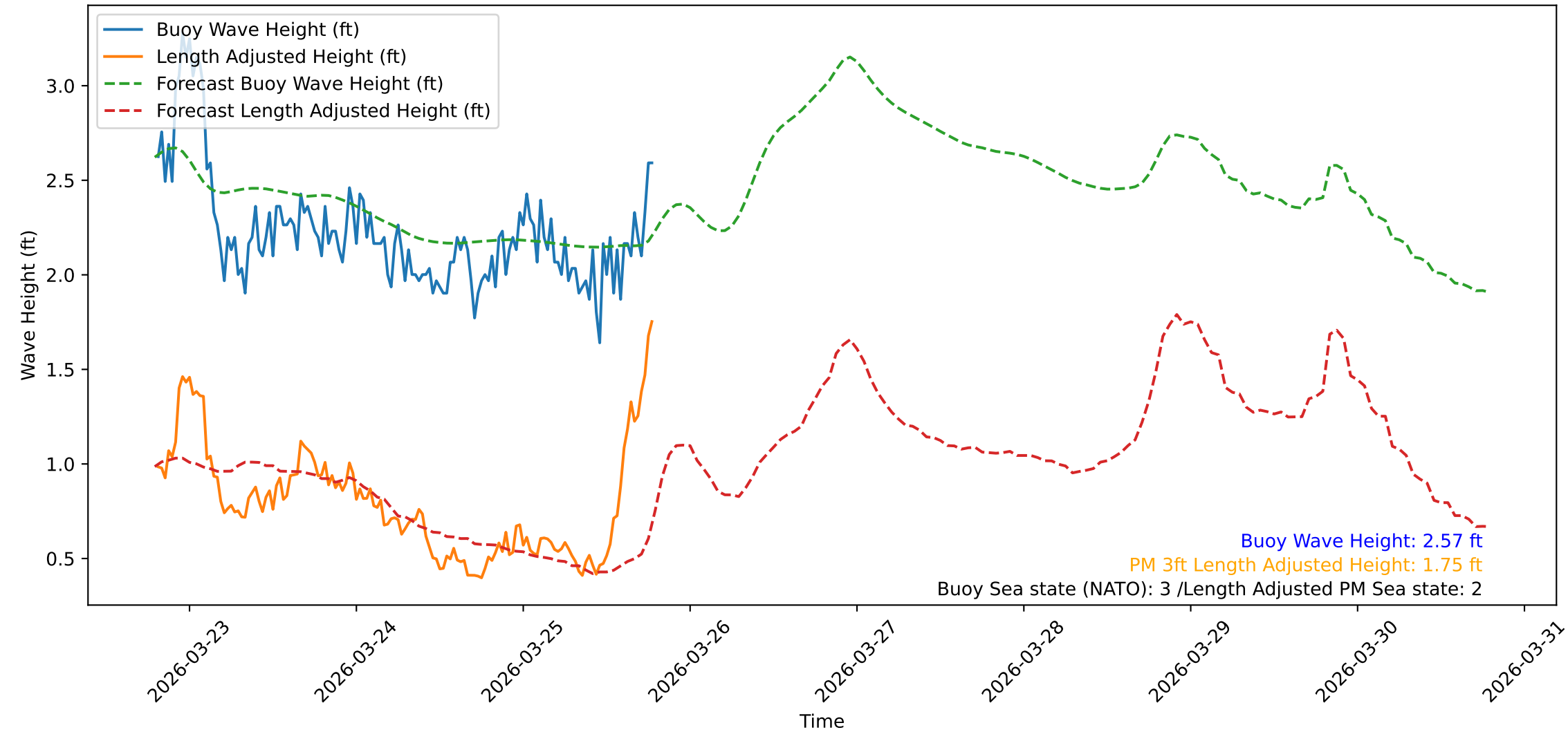
Wave Heights over Time for Green Beach at 2026-03-25 19:21:08
