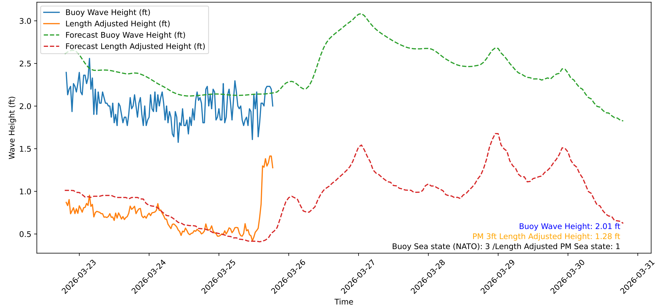
Wave Heights over Time for Oceanside Harbor at 2026-03-25 19:20:31
