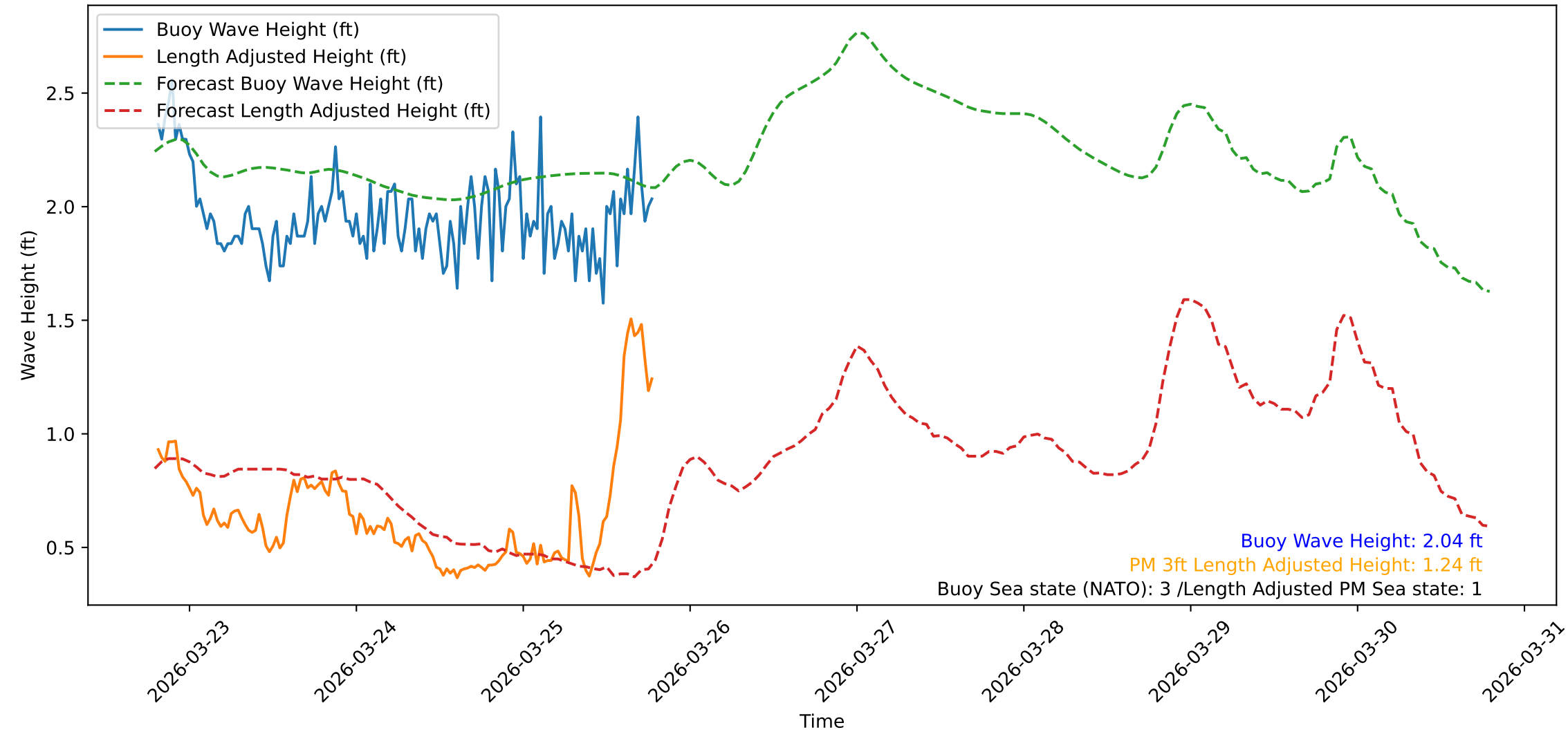
Wave Heights over Time for Red Beach at 2026-03-25 19:20:47
