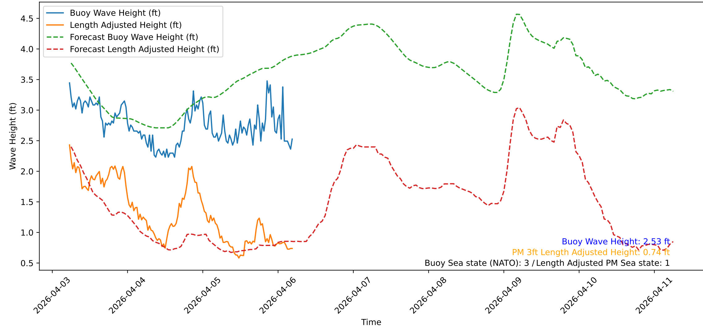
Wave Heights over Time for Green Beach at 2026-04-06 05:31:10
