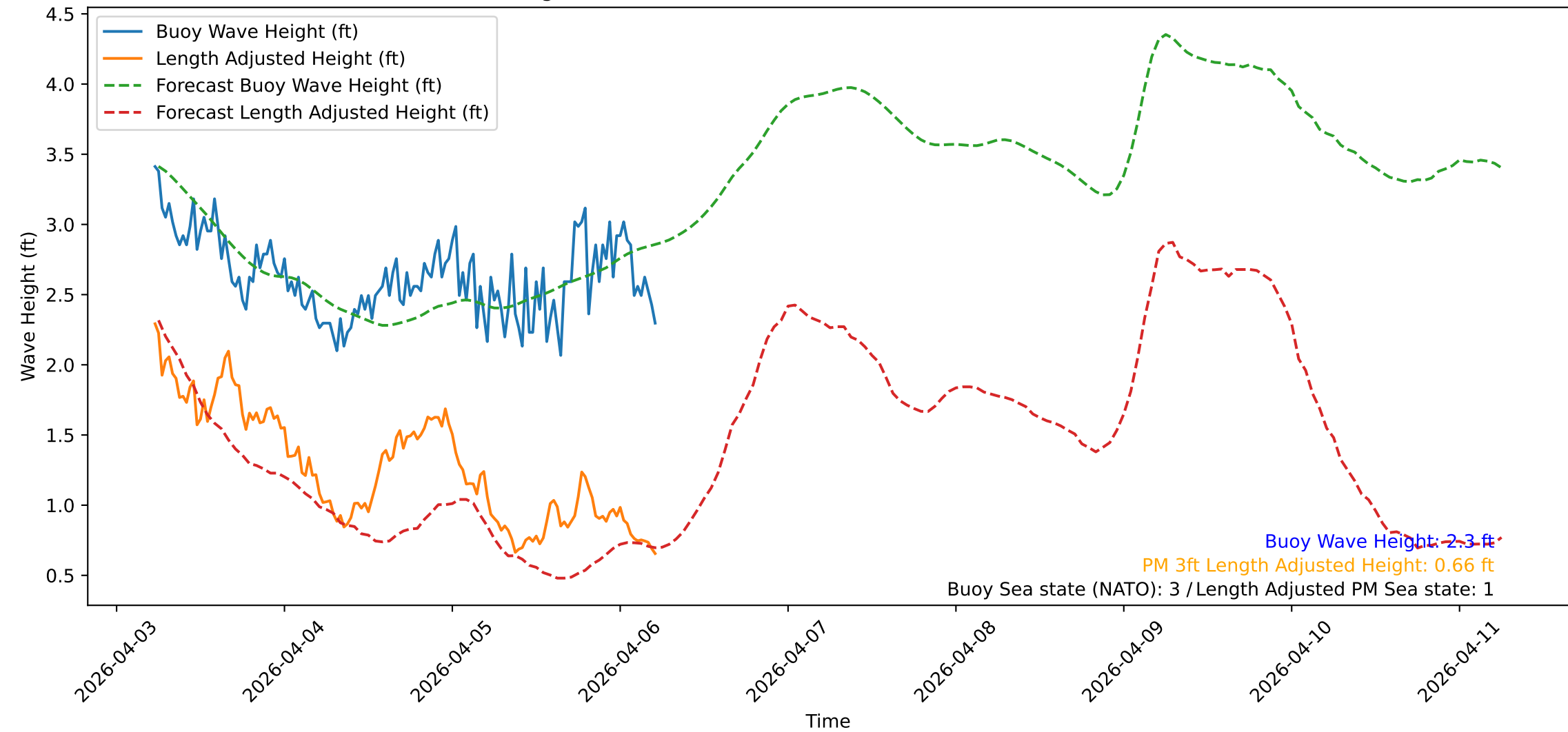
Wave Heights over Time for Oceanside Harbor at 2026-04-06 05:30:31
