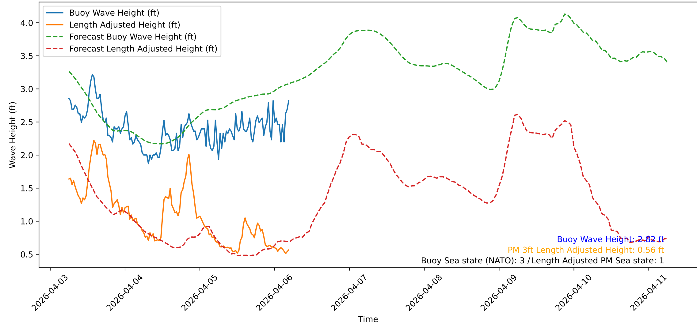
Wave Heights over Time for Red Beach at 2026-04-06 05:30:47
