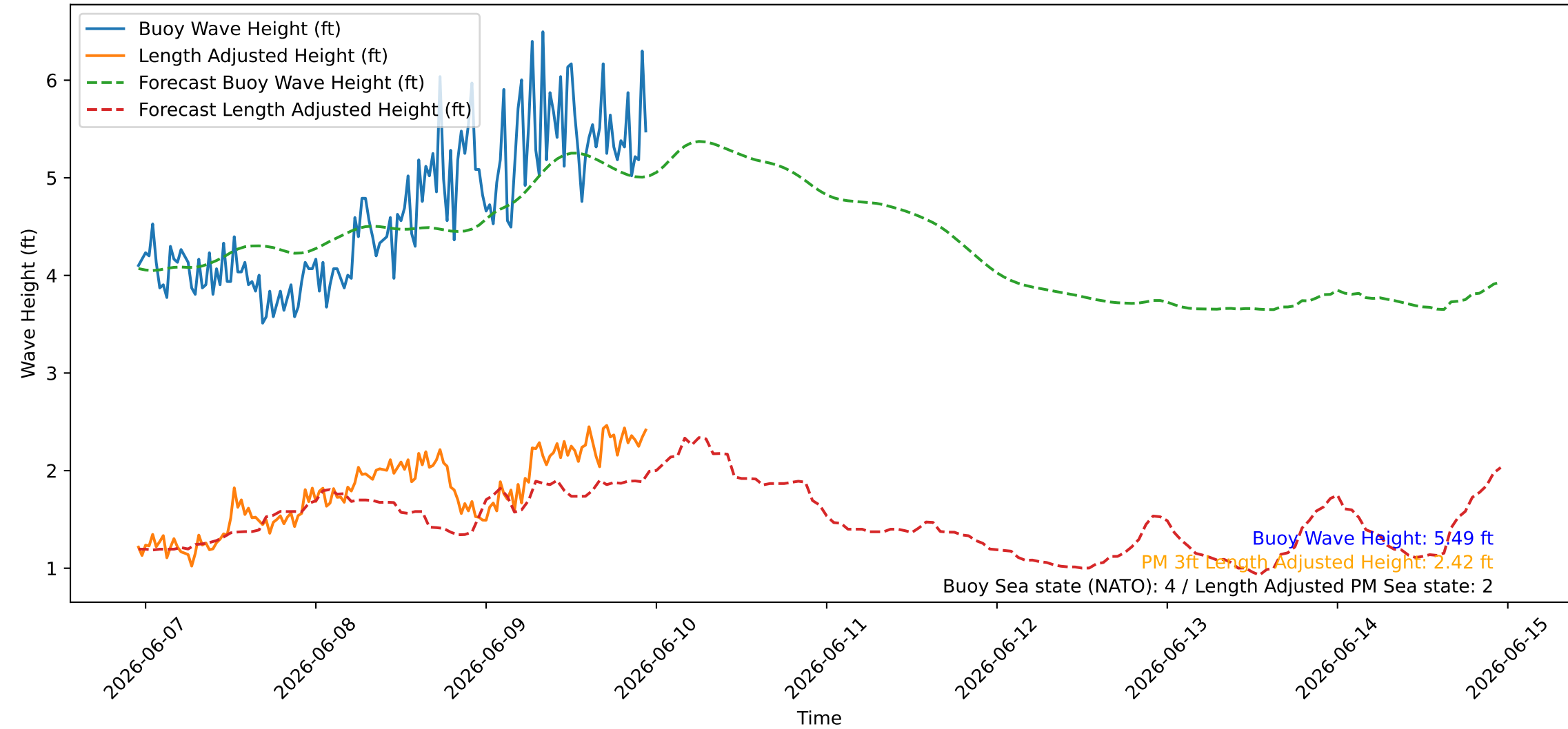
Wave Heights over Time for Oceanside Harbor at 2026-06-09 23:00:26
