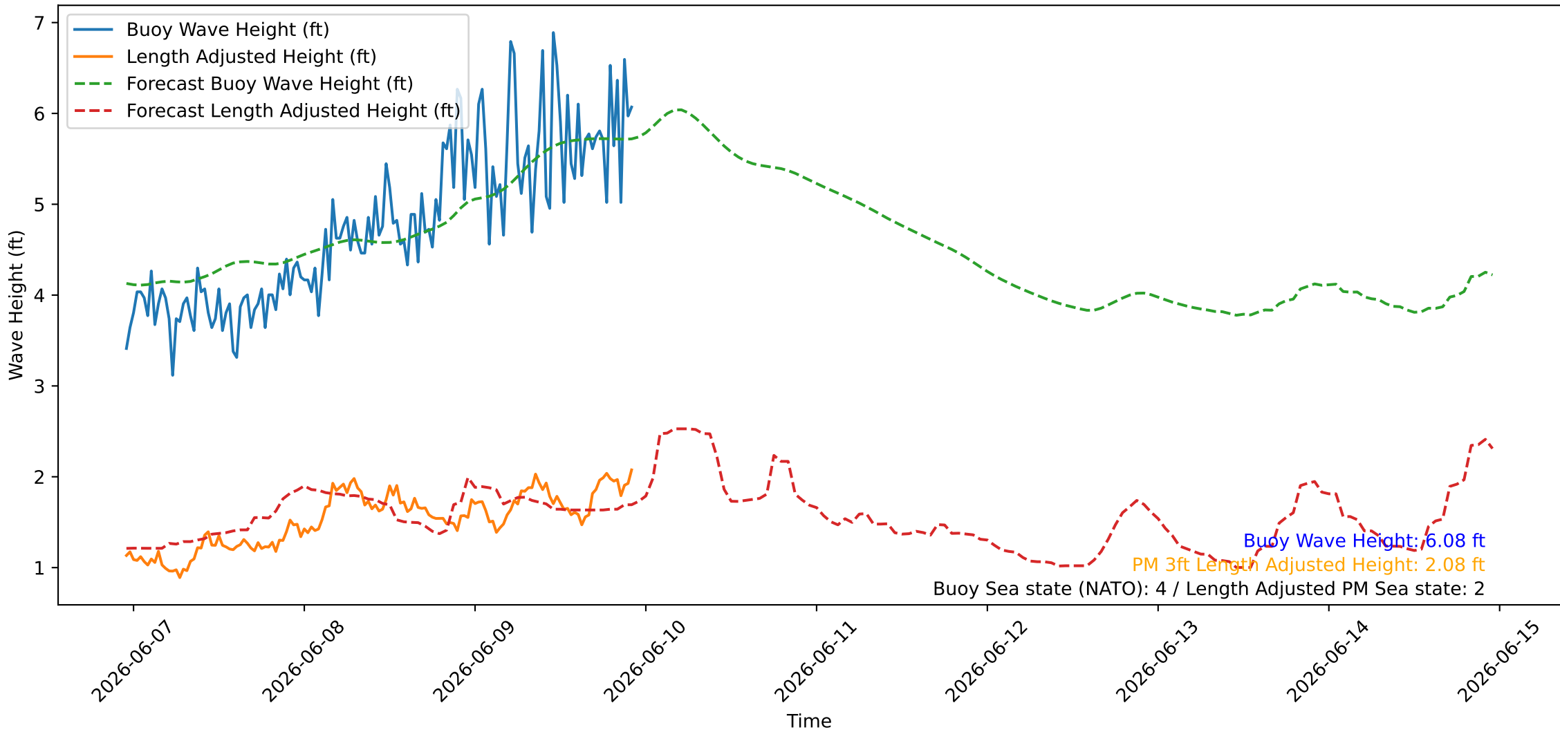
Wave Heights over Time for Green Beach at 2026-06-09 23:01:10
