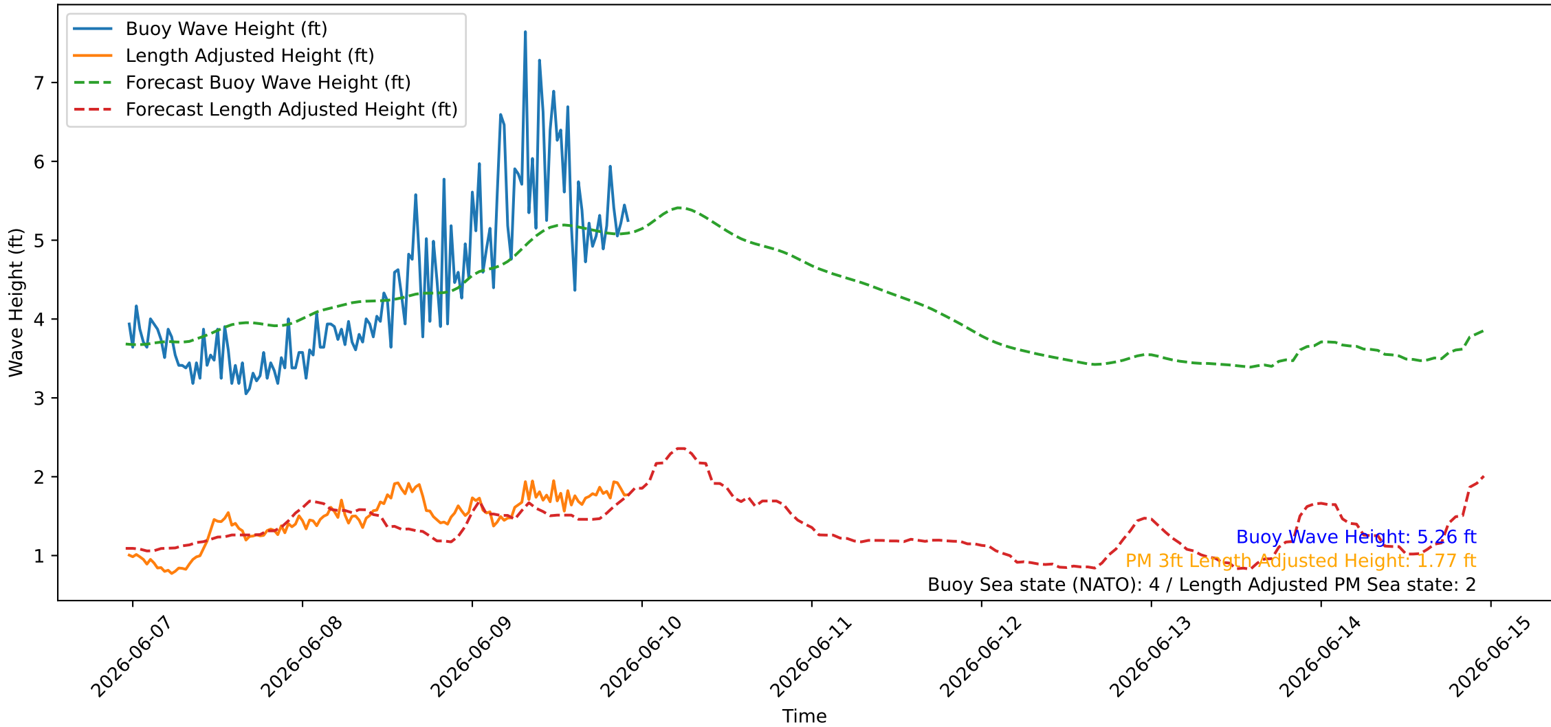
Wave Heights over Time for Red Beach at 2026-06-09 23:00:46
