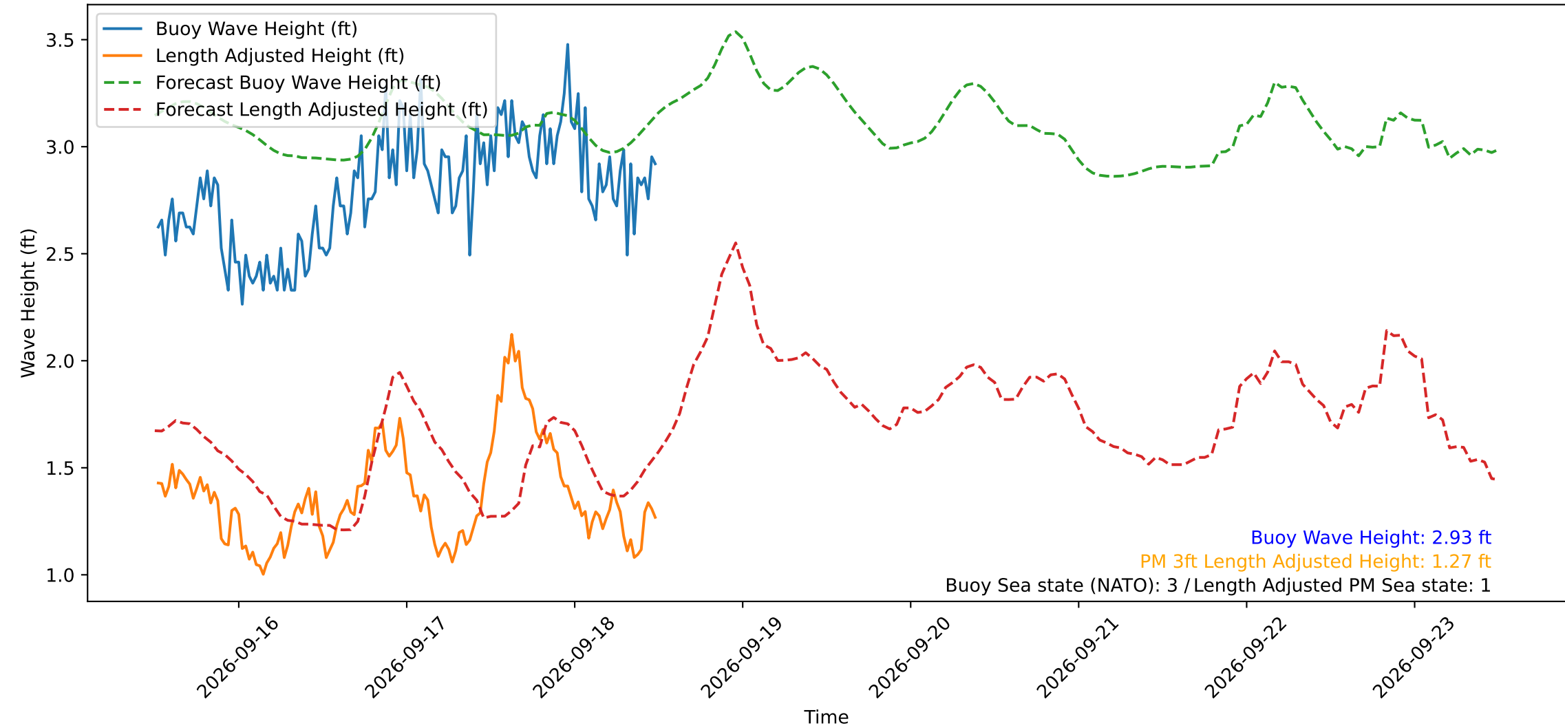
Wave Heights over Time for Green Beach at 2026-09-18 12:11:17
