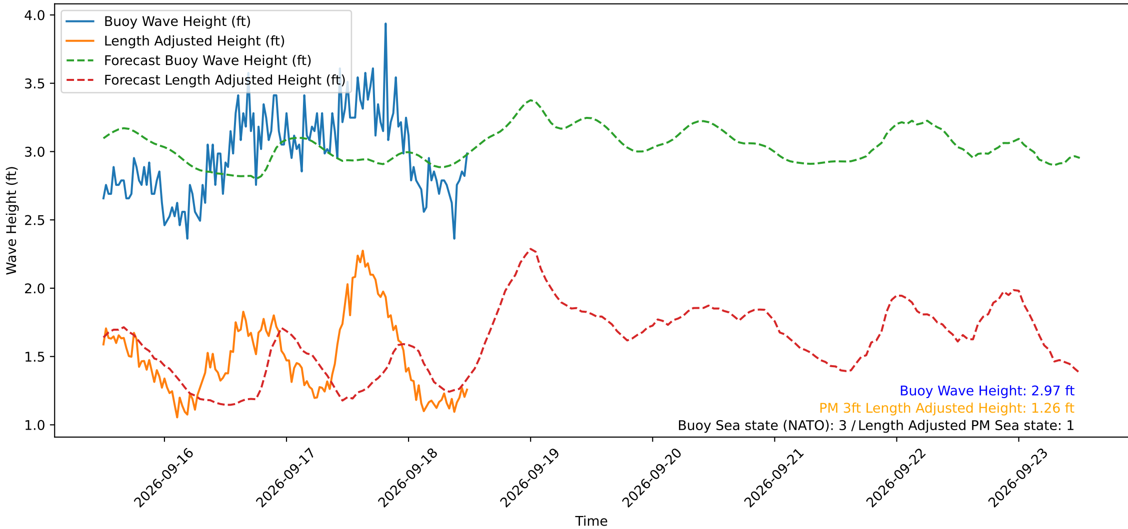
Wave Heights over Time for Oceanside Harbor at 2026-09-18 12:10:31
