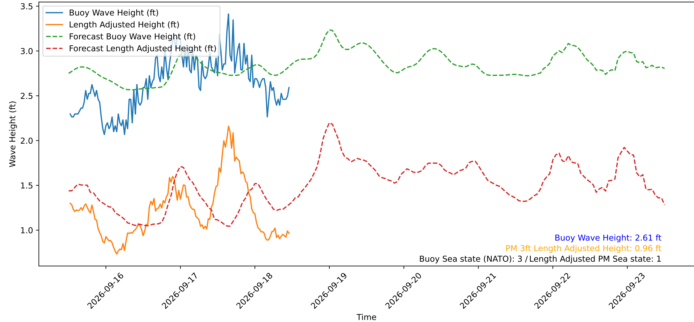
Wave Heights over Time for Red Beach at 2026-09-18 12:10:53
