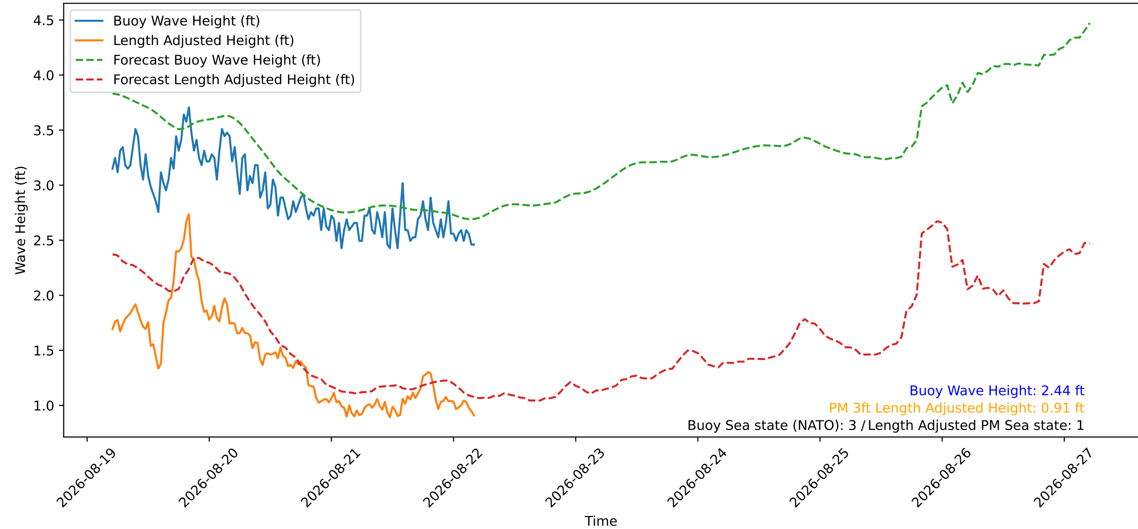
Wave Heights over Time for Green Beach at 2026-08-22 04:41:11
