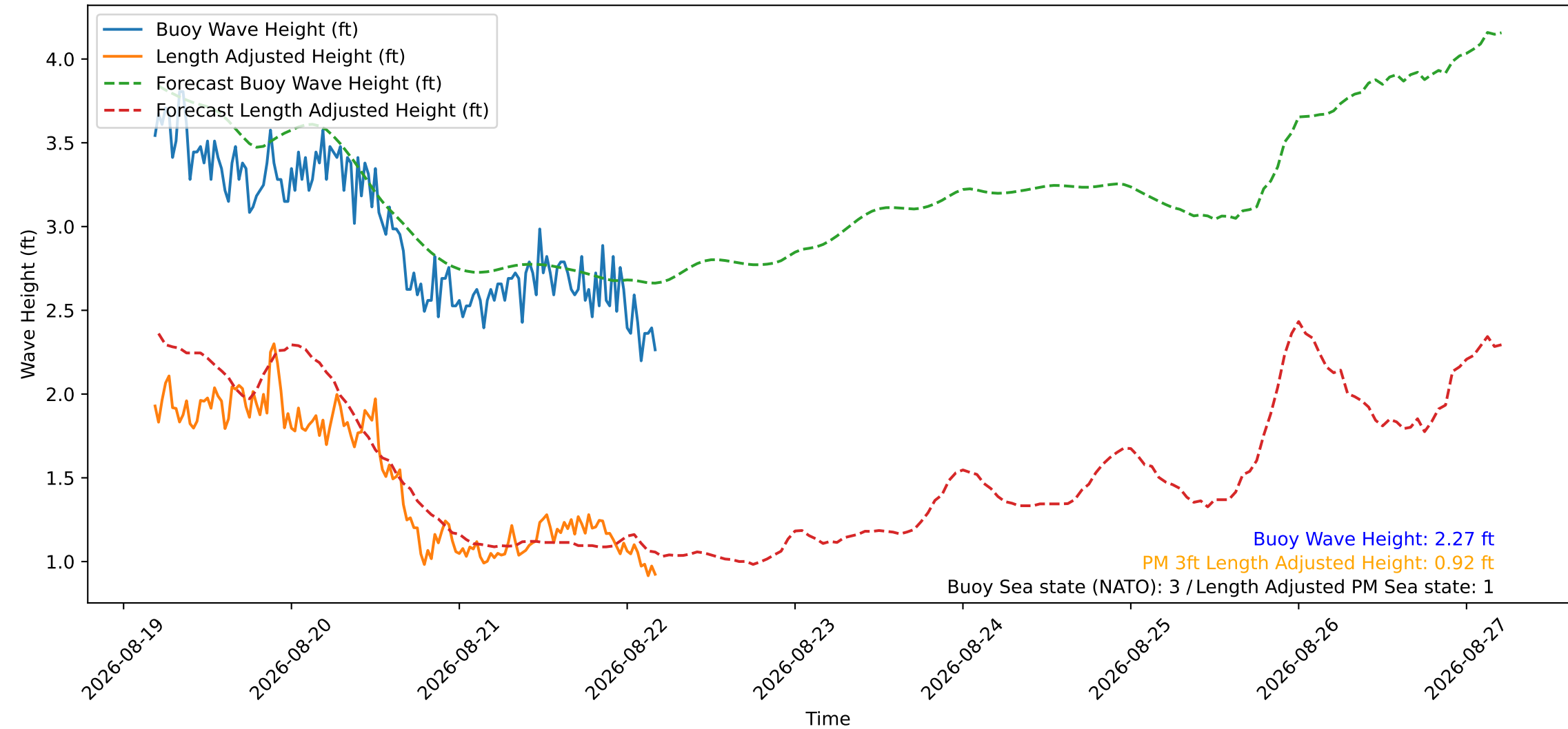
Wave Heights over Time for Oceanside Harbor at 2026-08-22 04:40:29
