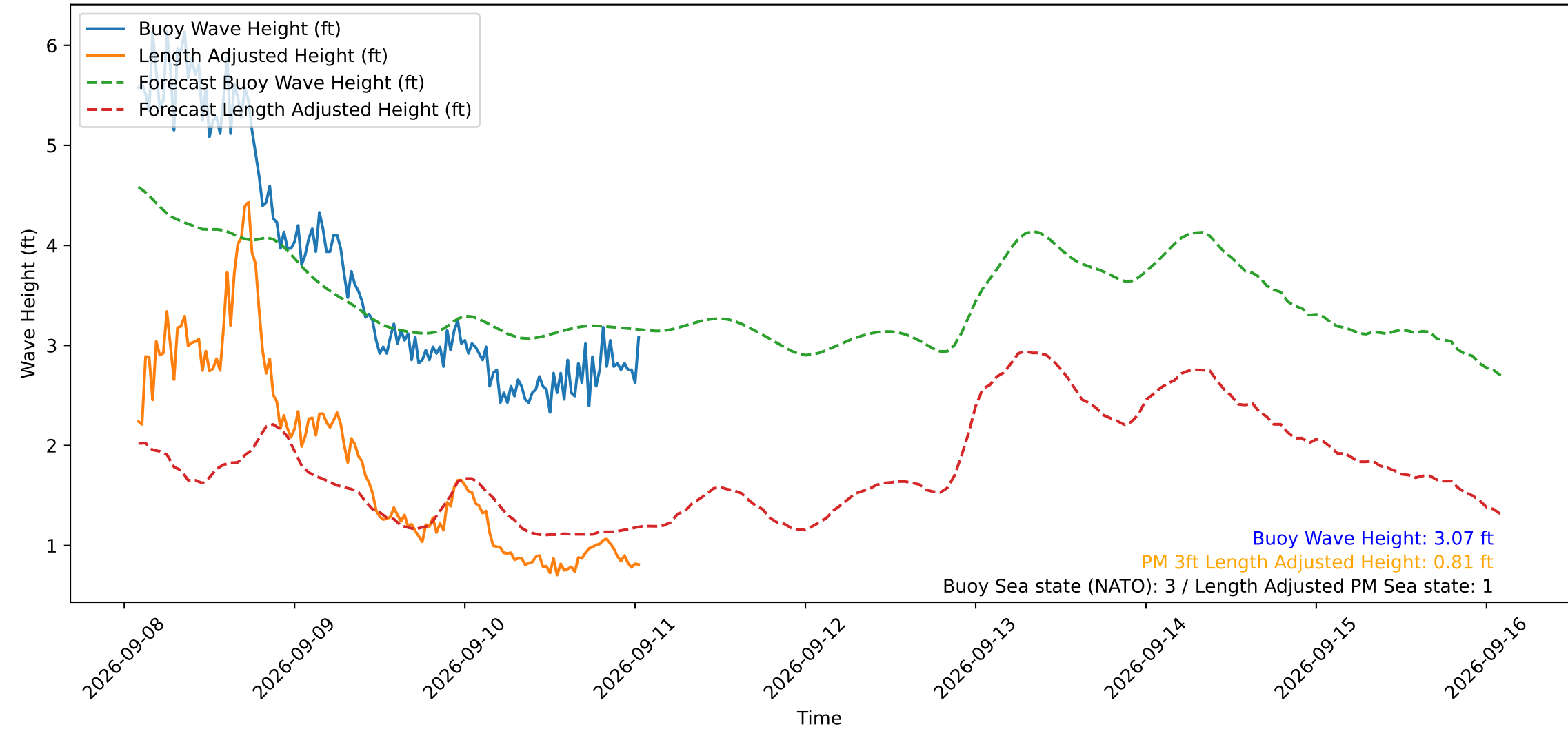
Wave Heights over Time for Red Beach at 2026-09-11 01:30:50
