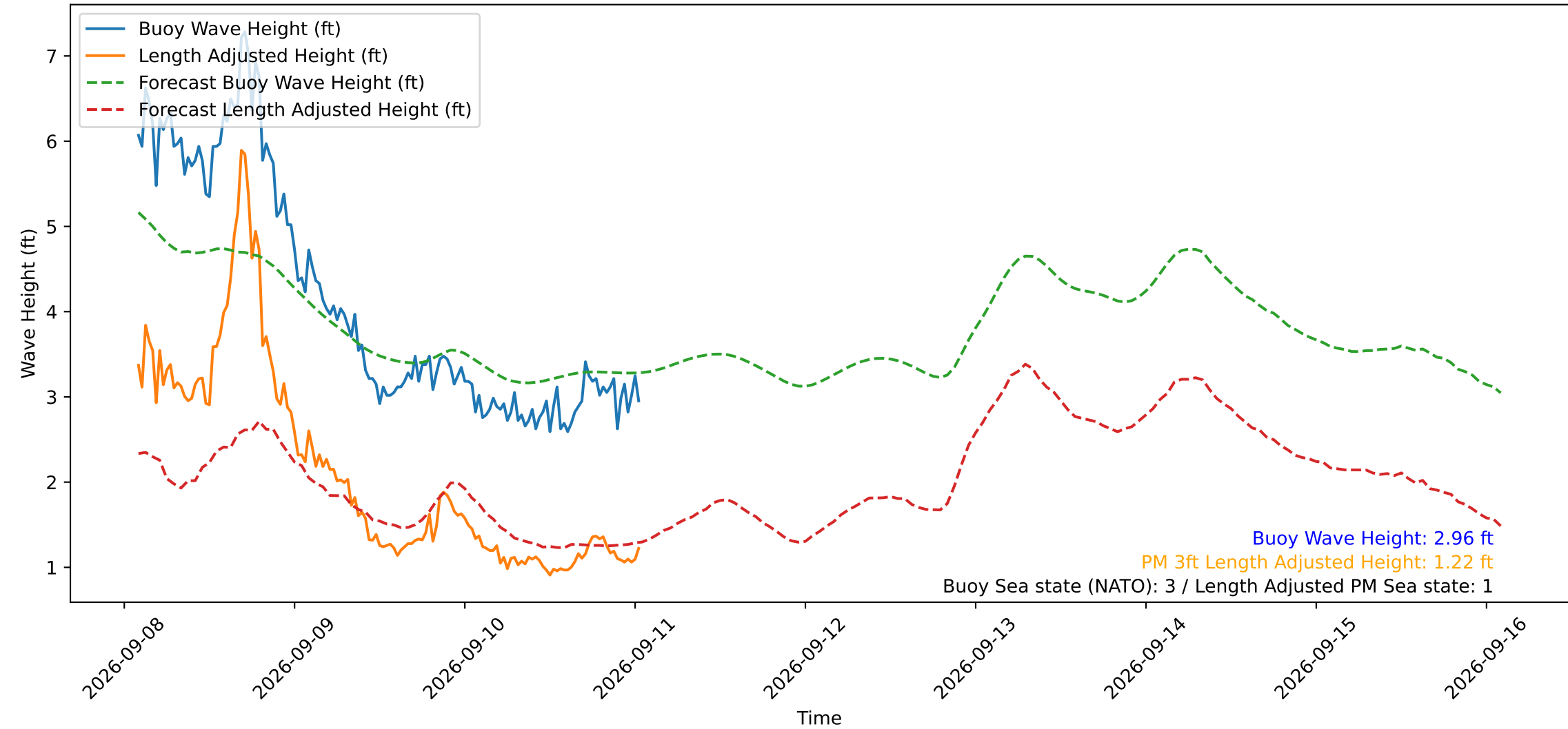
Wave Heights over Time for Green Beach at 2026-09-11 01:31:12
