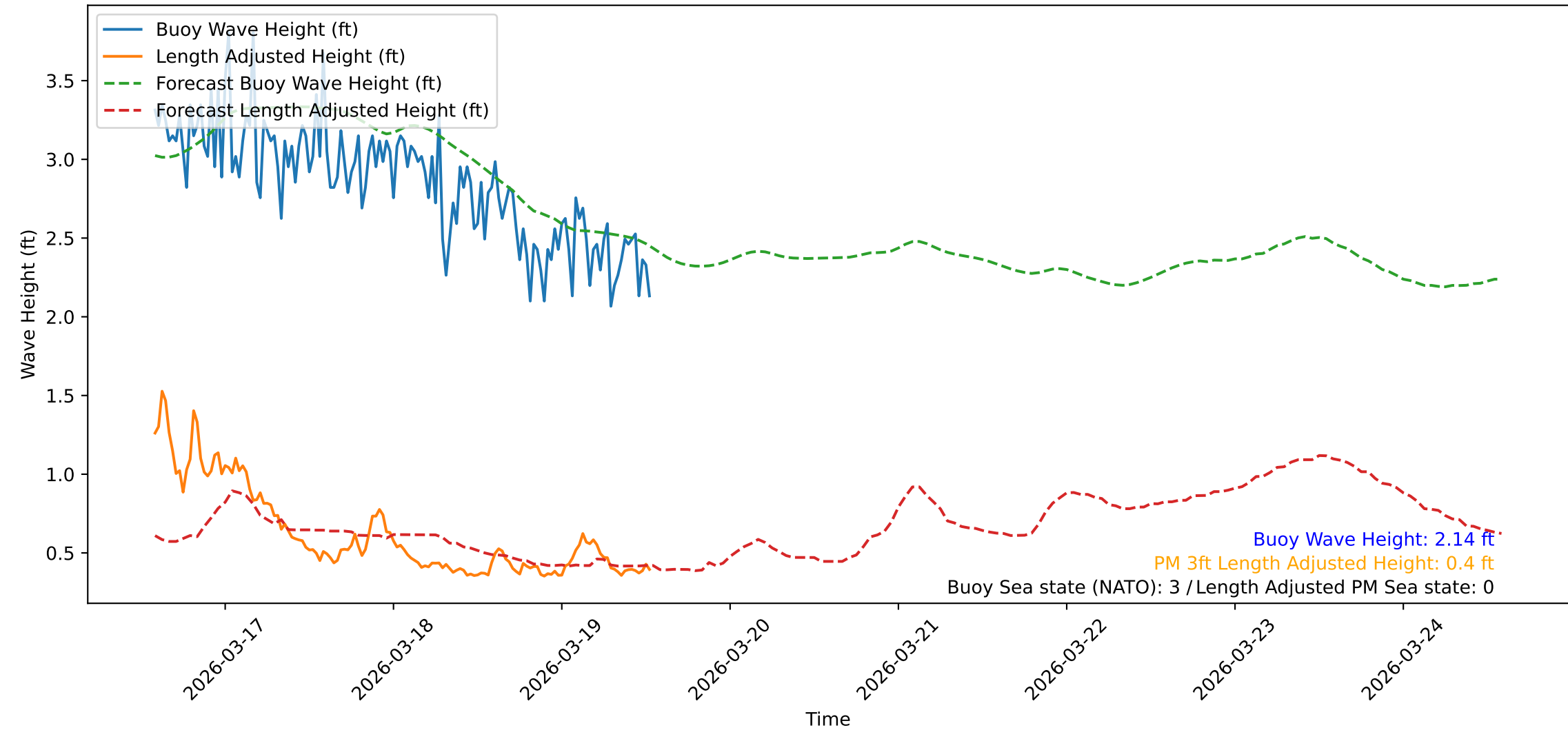
Wave Heights over Time for Red Beach at 2026-03-19 13:30:48
