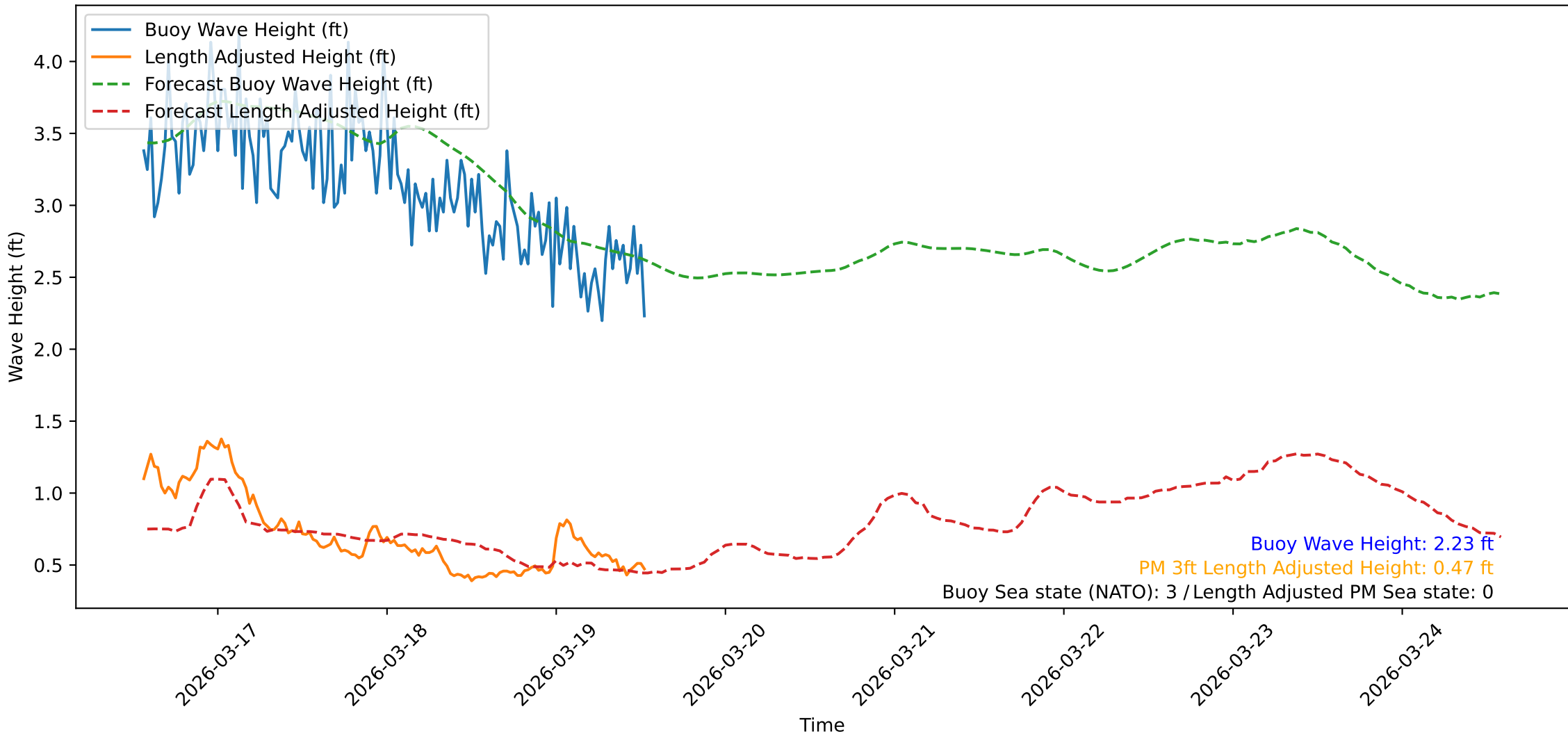
Wave Heights over Time for Green Beach at 2026-03-19 13:31:10
