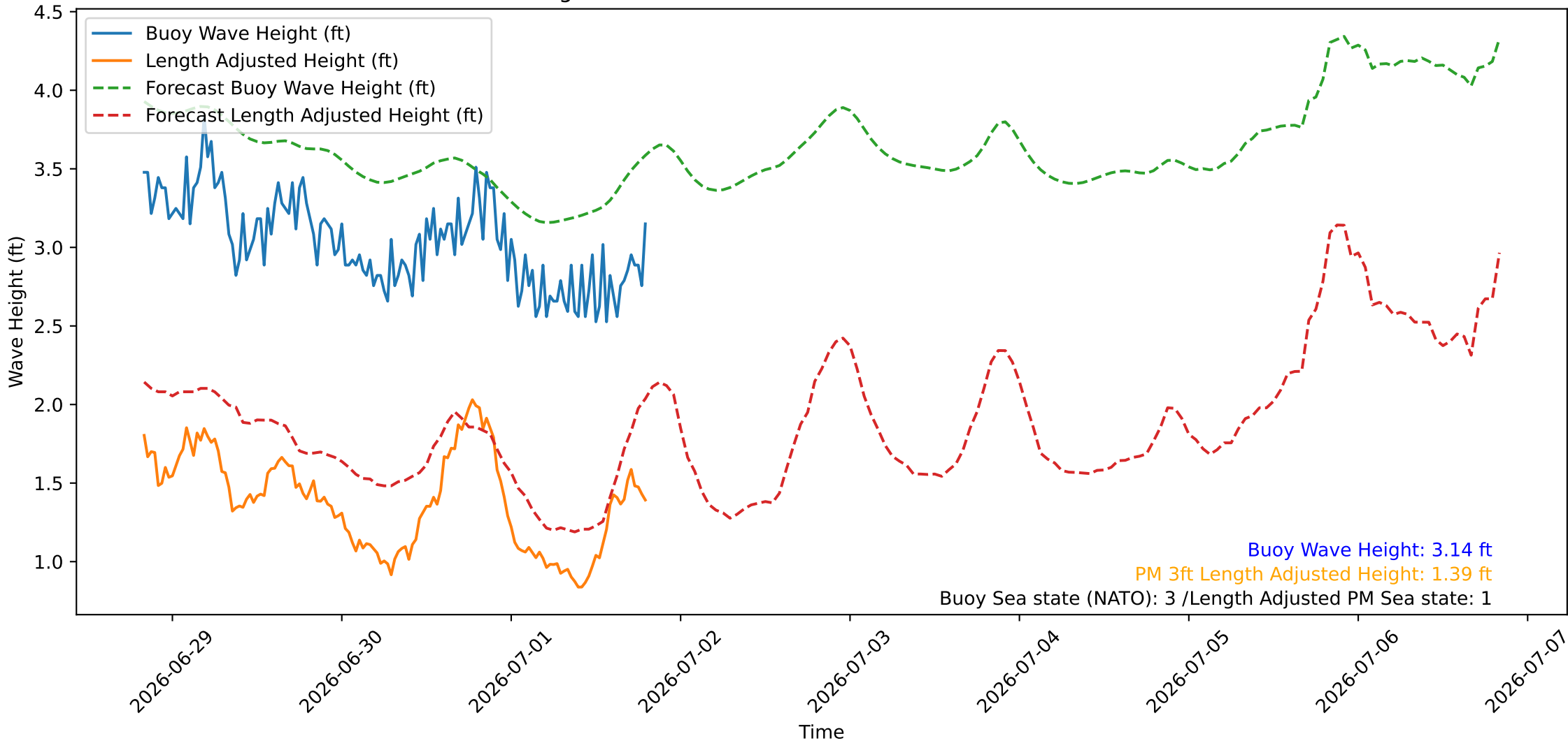
Wave Heights over Time for Green Beach at 2026-07-01 19:51:09
