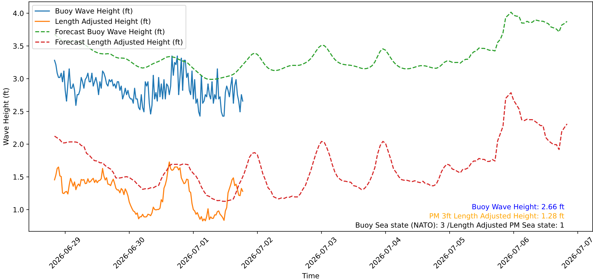
Wave Heights over Time for Red Beach at 2026-07-01 19:50:47
