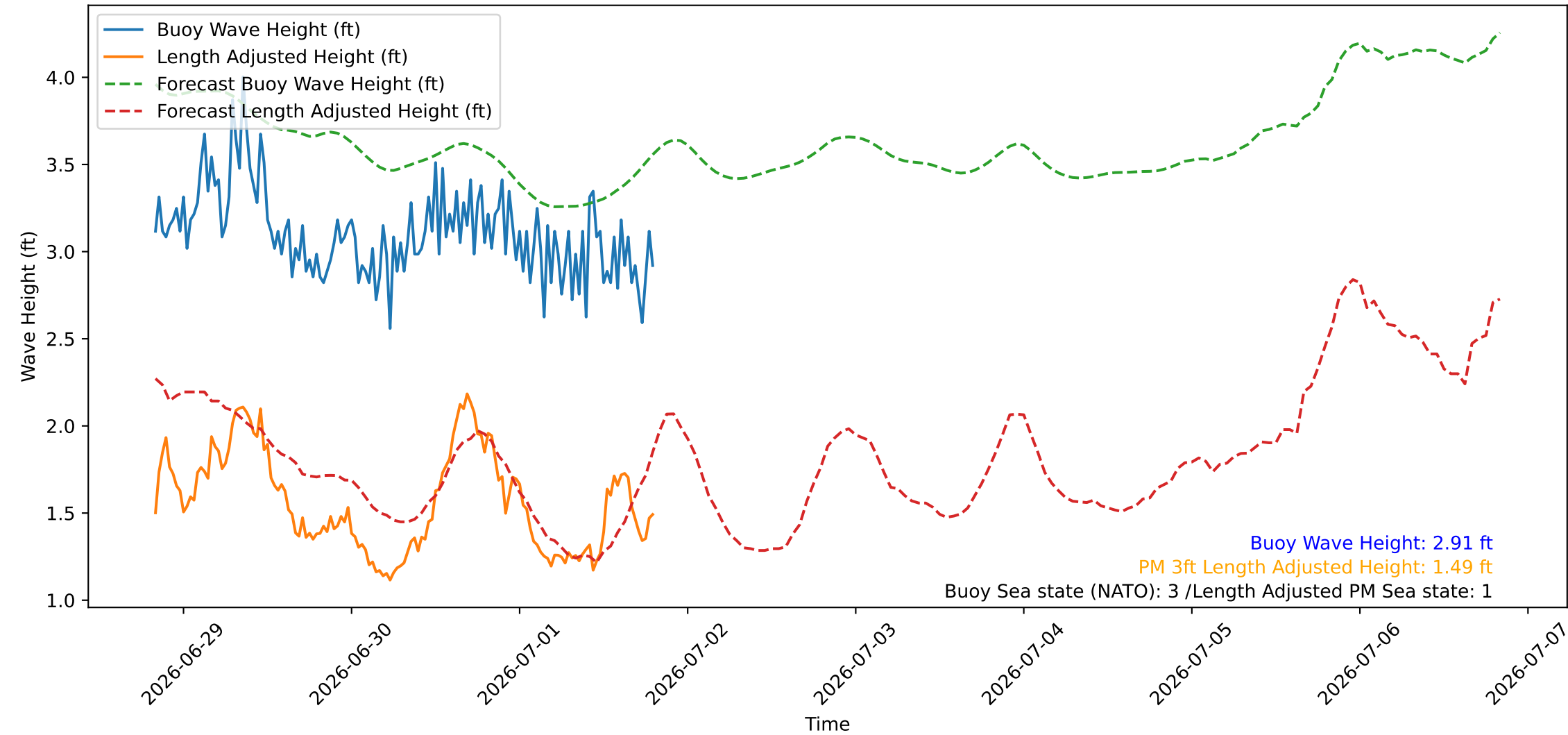
Wave Heights over Time for Oceanside Harbor at 2026-07-01 19:50:26
