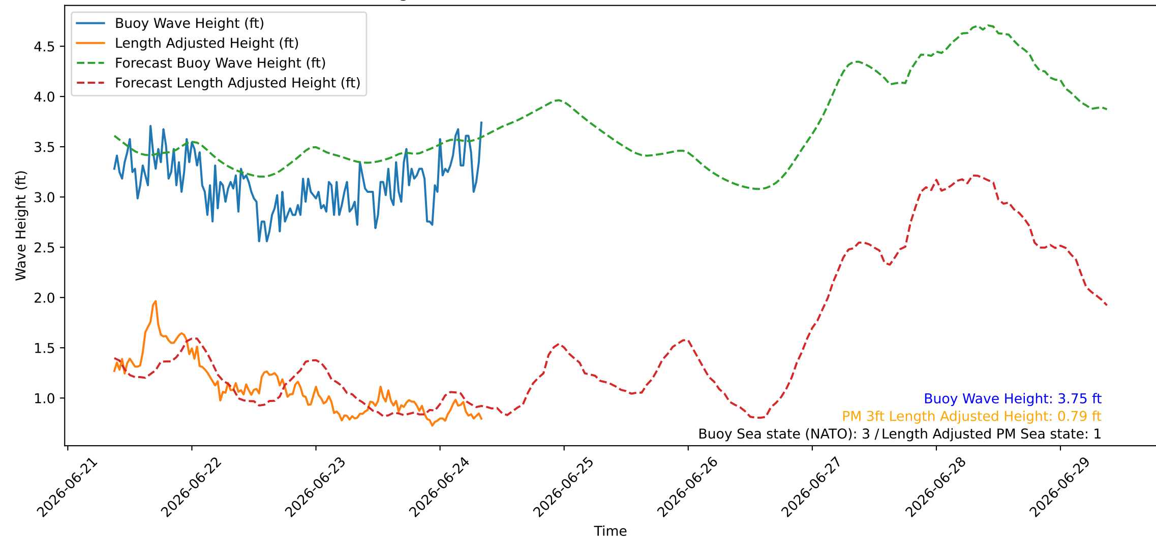
Wave Heights over Time for Oceanside Harbor at 2026-06-24 08:50:26
