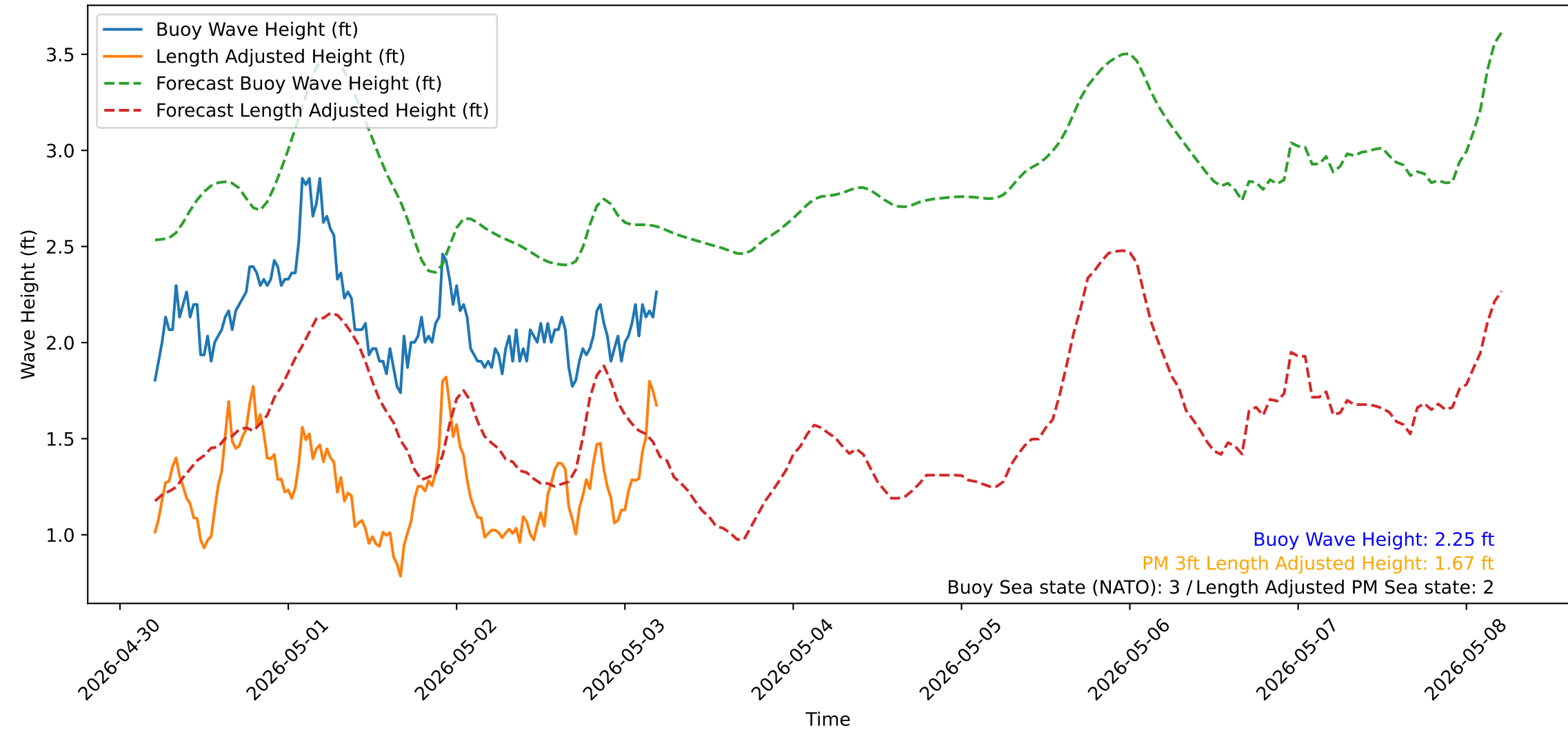
Wave Heights over Time for Green Beach at 2026-05-03 05:11:12
