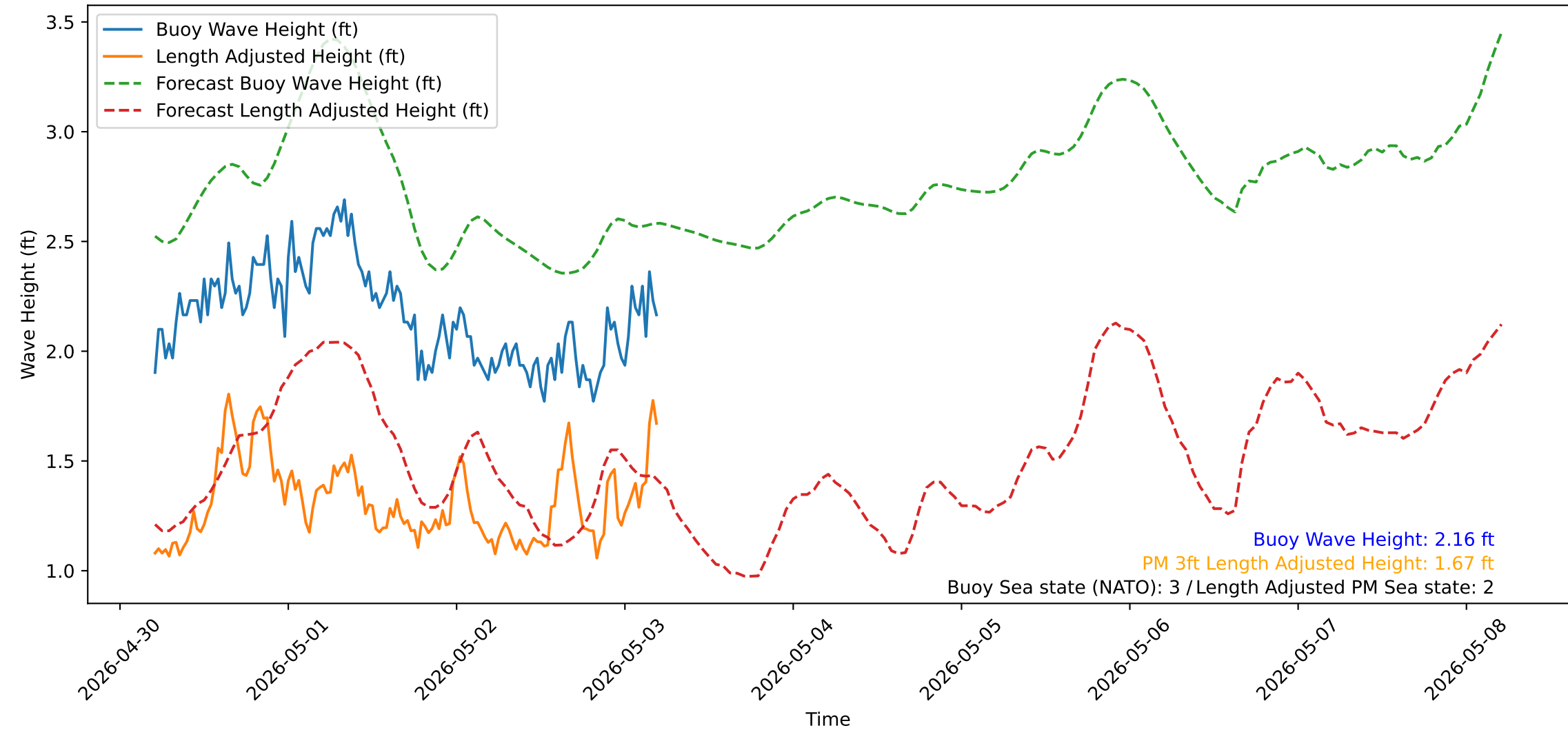
Wave Heights over Time for Oceanside Harbor at 2026-05-03 05:10:31
