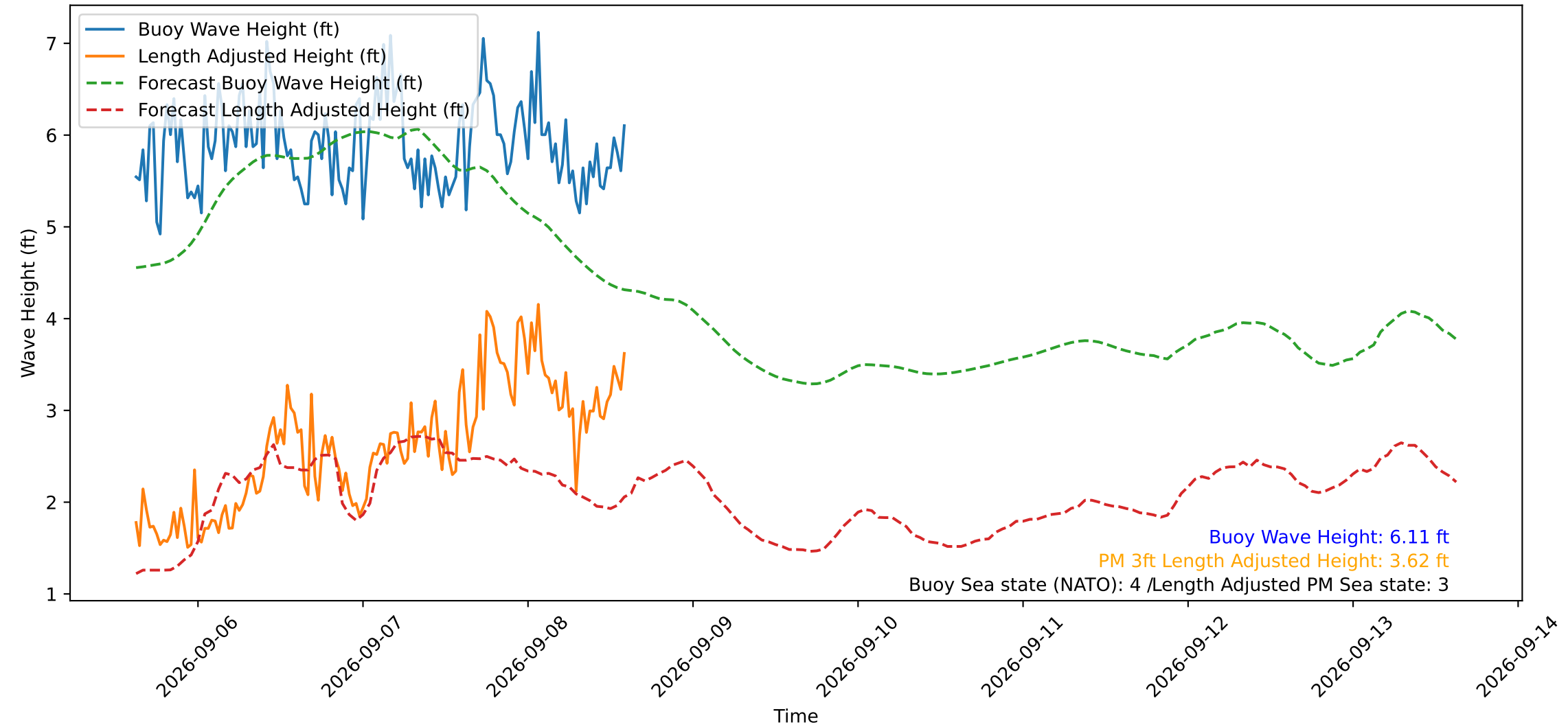
Wave Heights over Time for Oceanside Harbor at 2026-09-08 14:50:30
