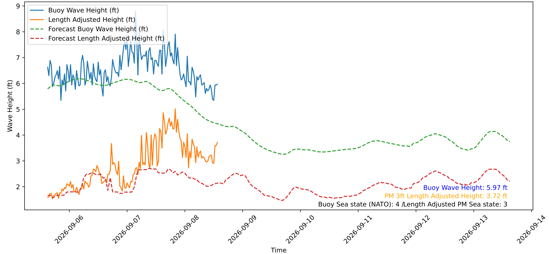
Wave Heights over Time for Green Beach at 2026-09-08 14:51:14
