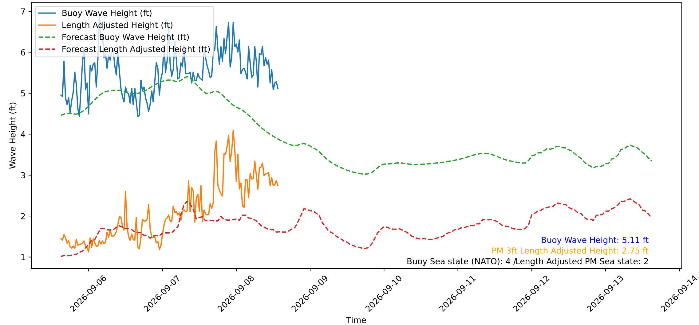
Wave Heights over Time for Red Beach at 2026-09-08 14:50:50
