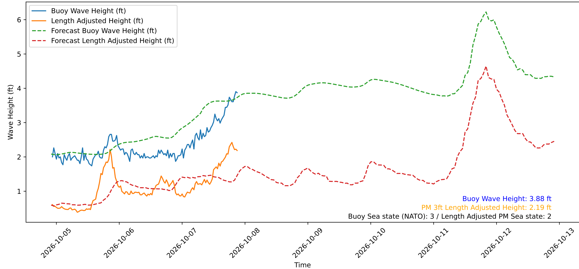
Wave Heights over Time for Red Beach at 2026-10-07 22:00:50
