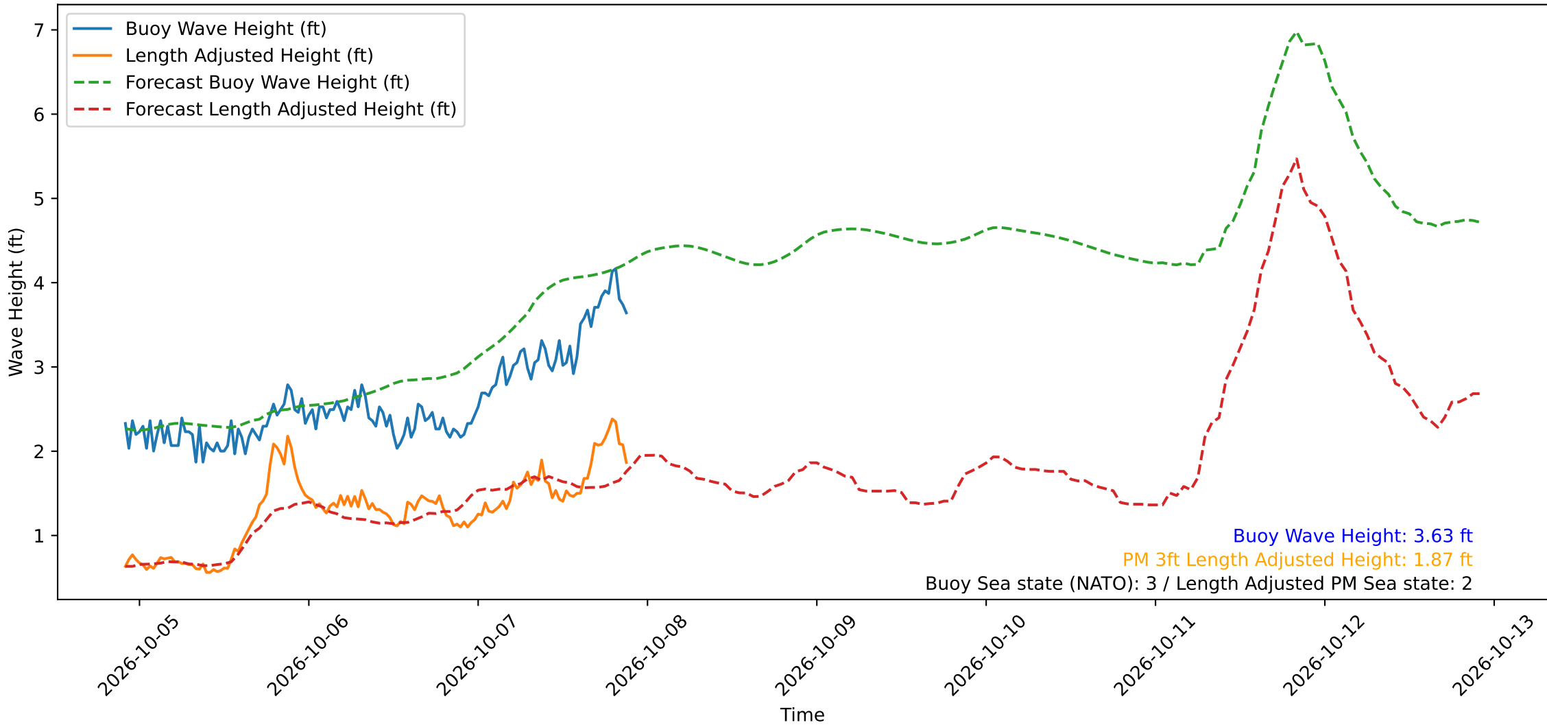
Wave Heights over Time for Oceanside Harbor at 2026-10-07 22:00:30
