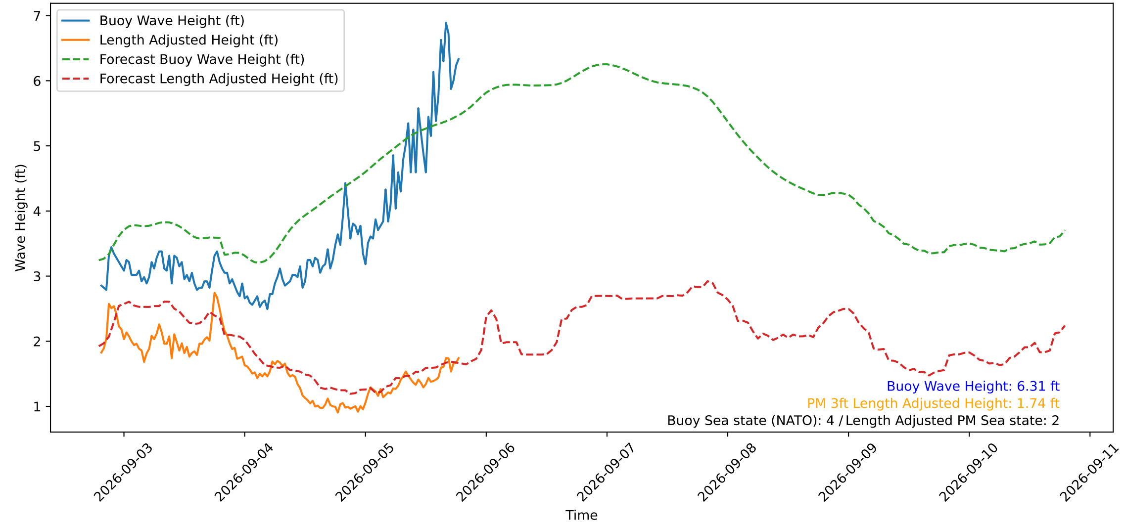
Wave Heights over Time for Green Beach at 2026-09-05 19:11:12
