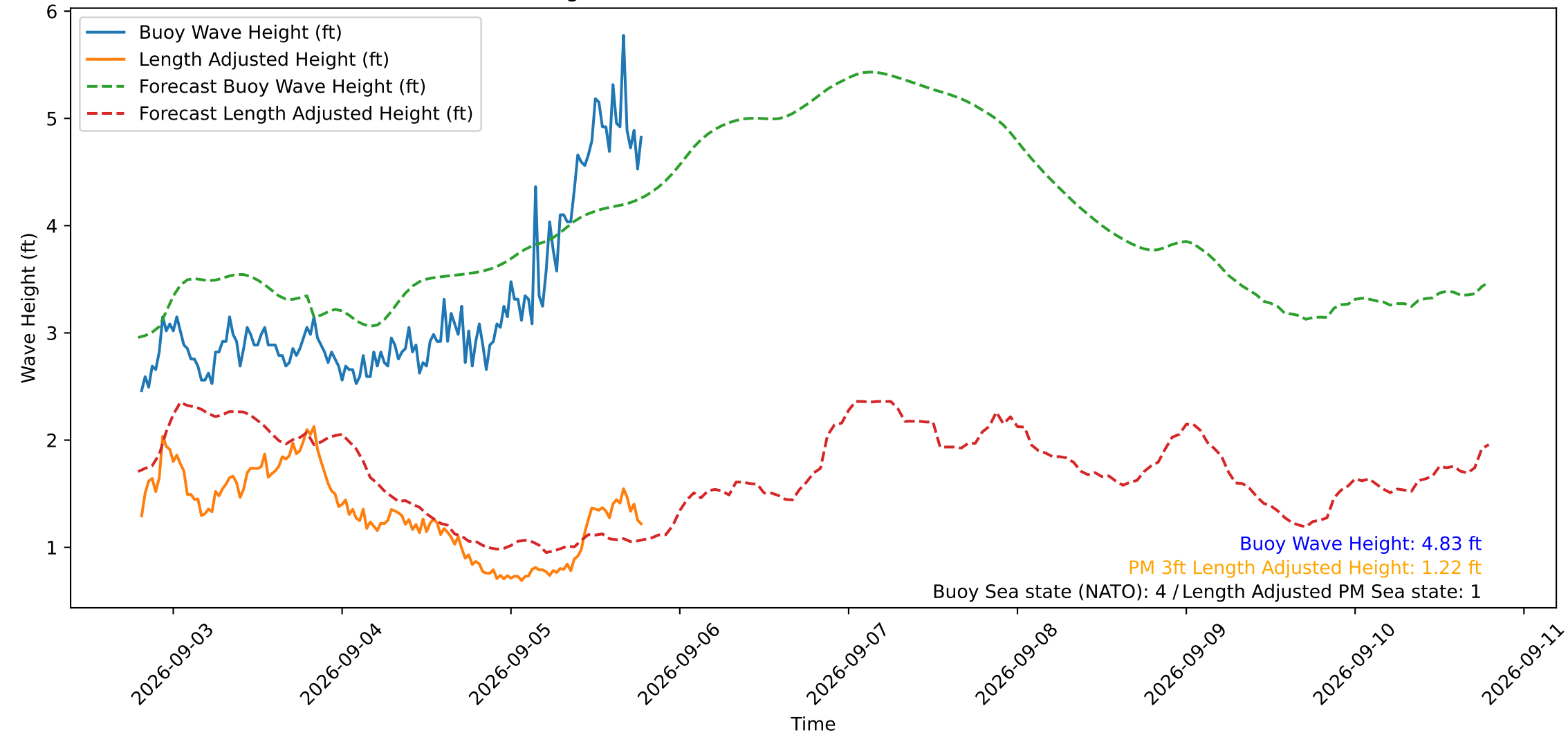
Wave Heights over Time for Red Beach at 2026-09-05 19:10:49
