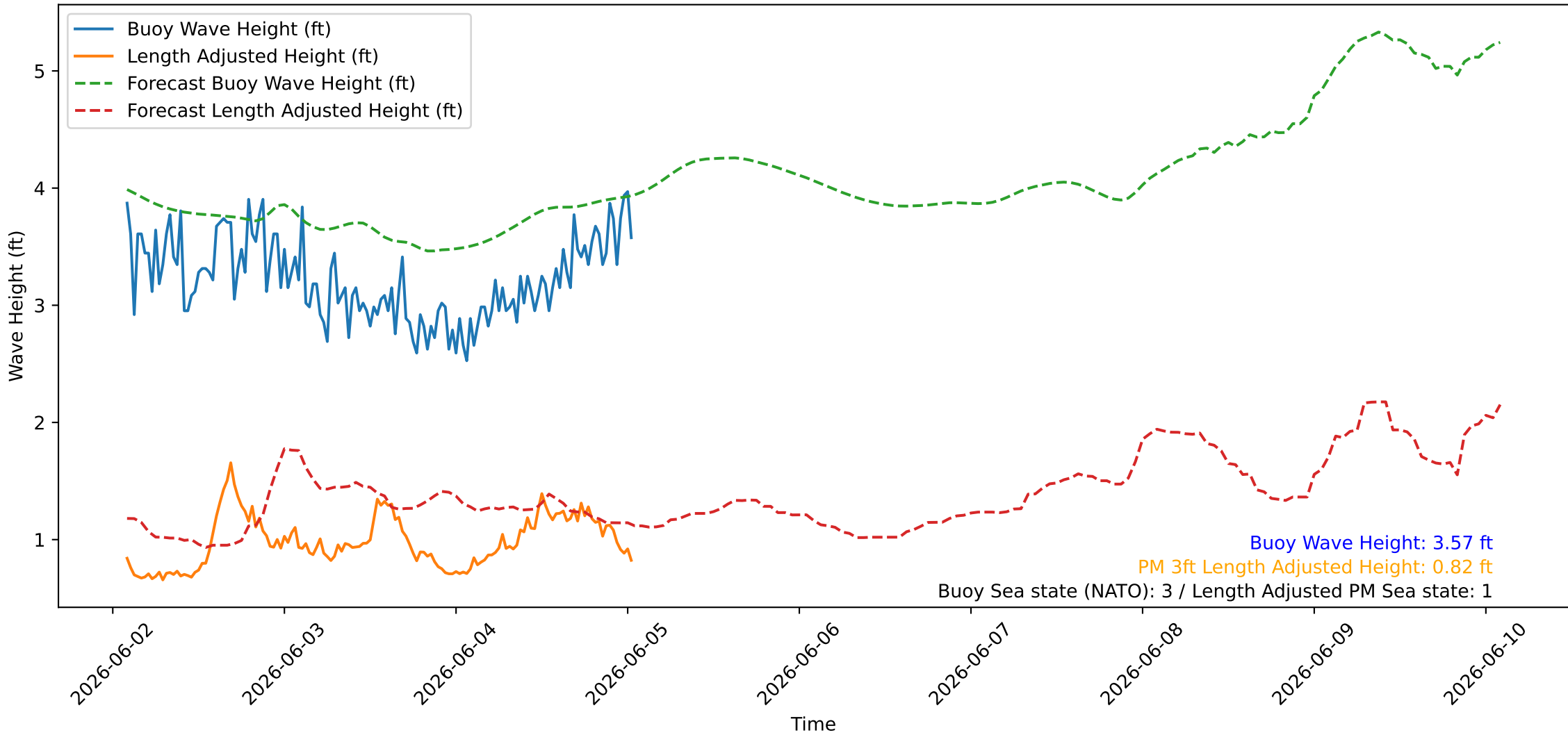
Wave Heights over Time for Red Beach at 2026-06-05 01:30:45
