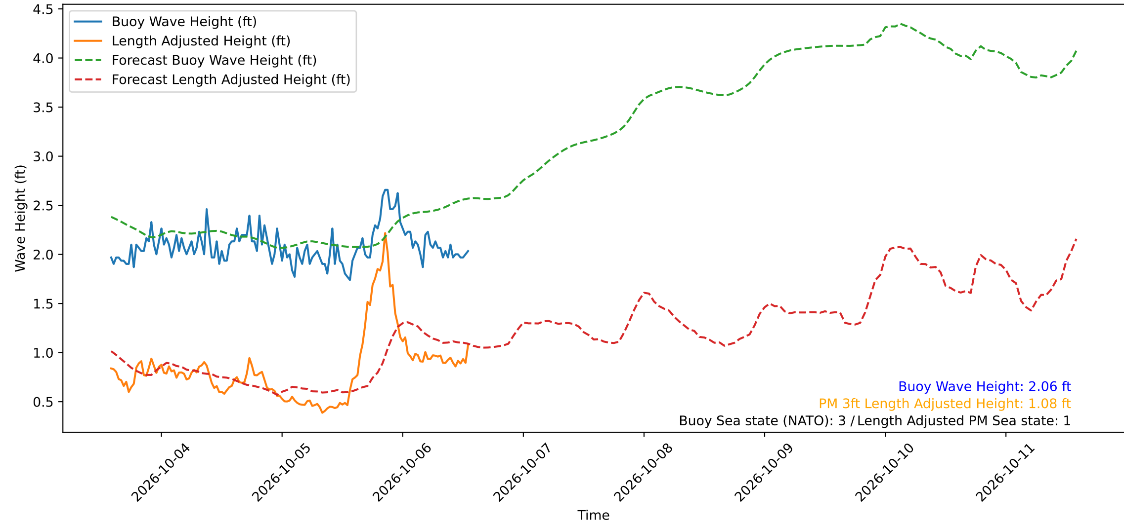
Wave Heights over Time for Red Beach at 2026-10-06 13:50:51
