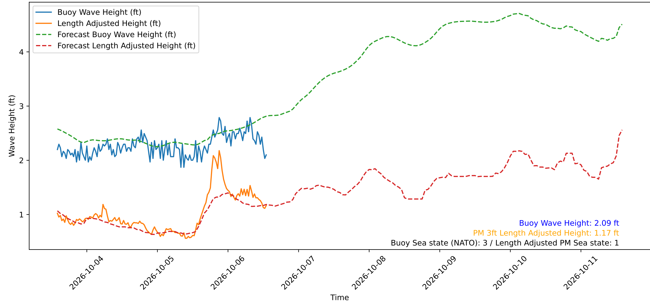
Wave Heights over Time for Oceanside Harbor at 2026-10-06 13:50:31
