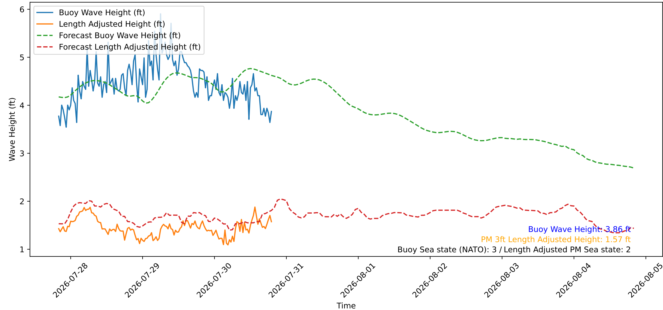
Wave Heights over Time for Oceanside Harbor at 2026-07-30 19:50:26
