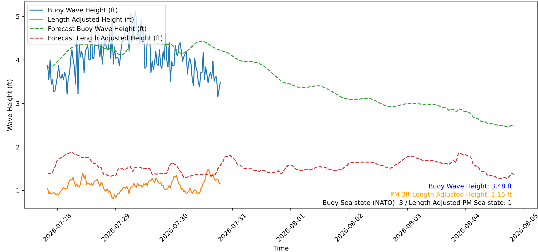
Wave Heights over Time for Red Beach at 2026-07-30 19:50:46
