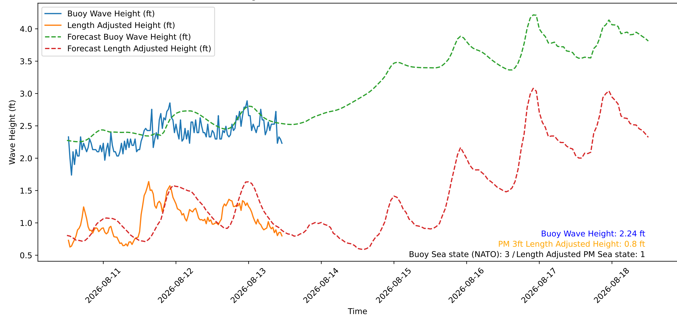
Wave Heights over Time for Red Beach at 2026-08-13 12:10:45
