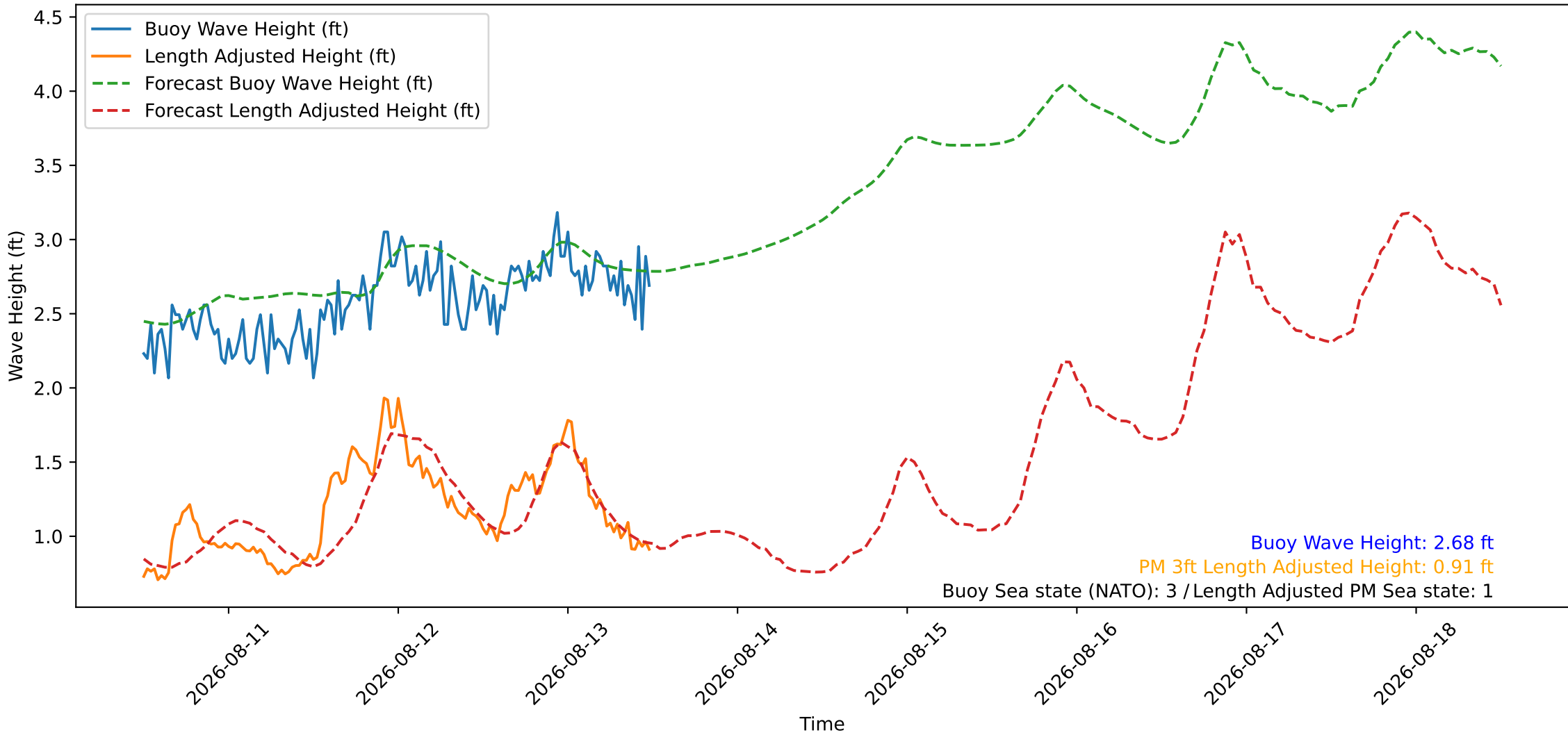
Wave Heights over Time for Oceanside Harbor at 2026-08-13 12:10:26
