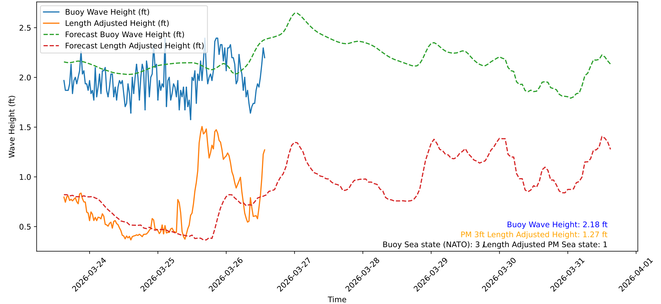
Wave Heights over Time for Red Beach at 2026-03-26 14:30:48
