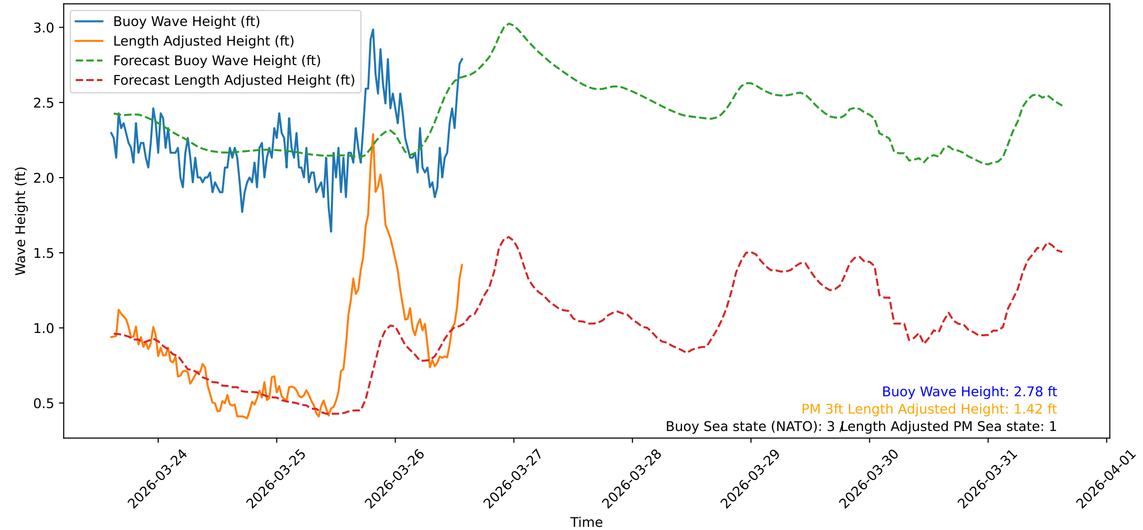
Wave Heights over Time for Green Beach at 2026-03-26 14:31:09
