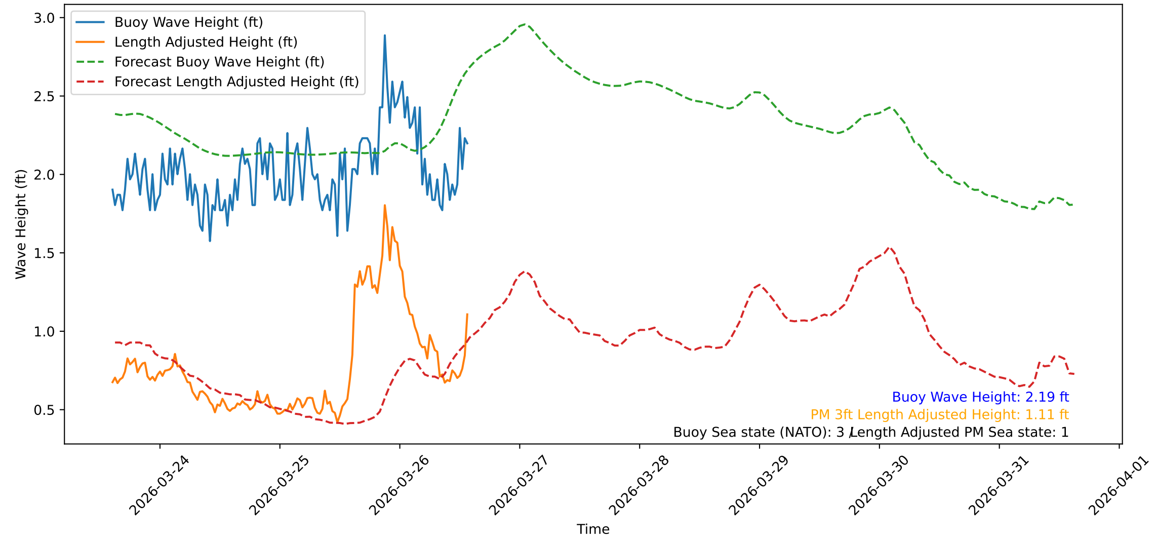
Wave Heights over Time for Oceanside Harbor at 2026-03-26 14:30:31
