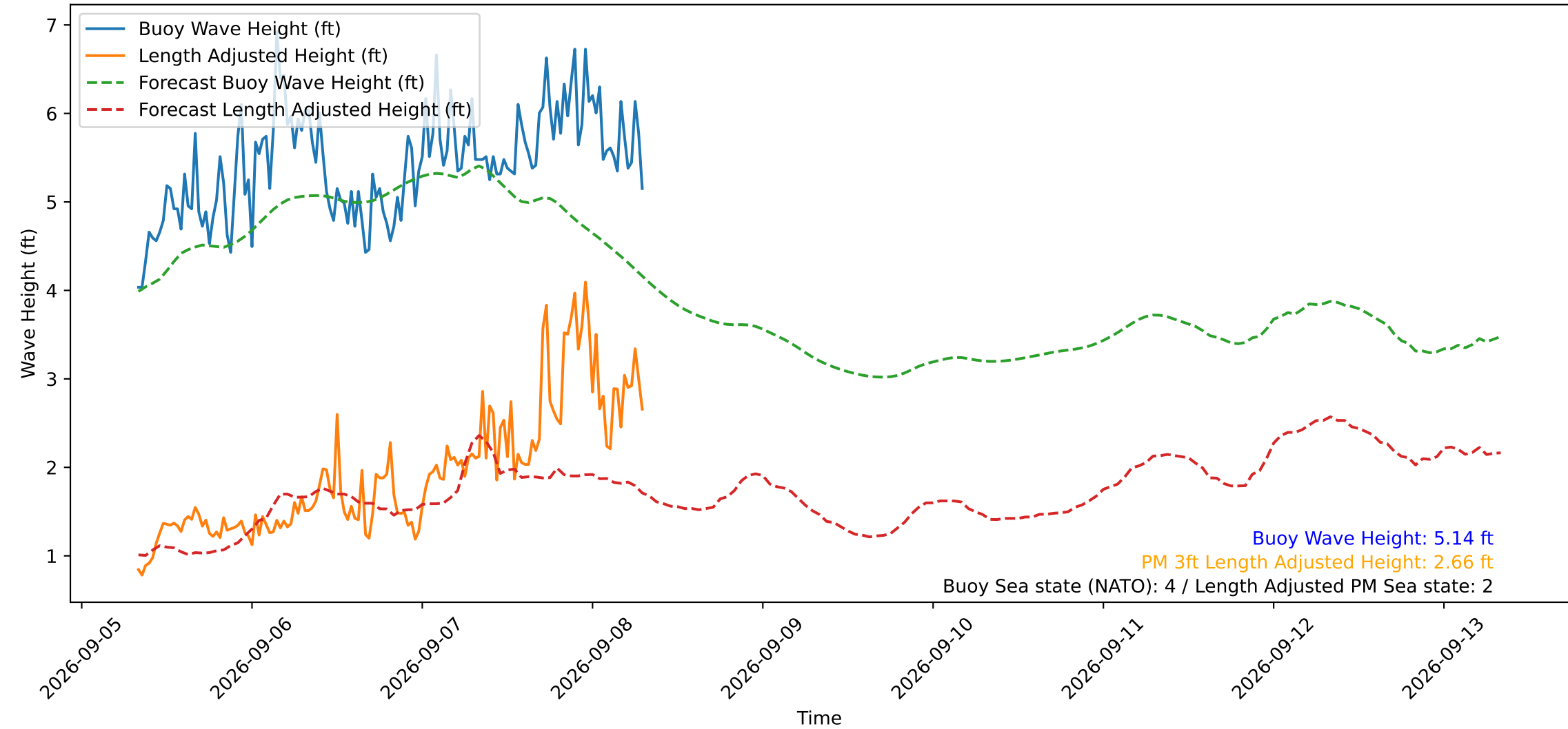
Wave Heights over Time for Red Beach at 2026-09-08 07:50:51
