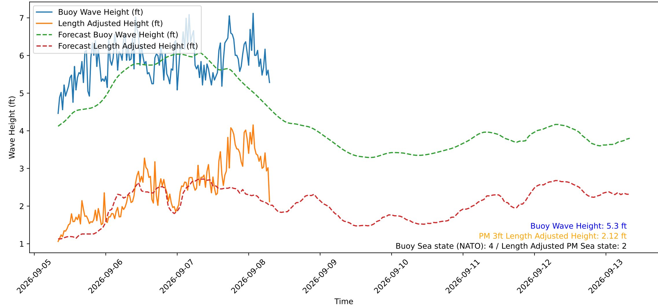
Wave Heights over Time for Oceanside Harbor at 2026-09-08 07:50:30
