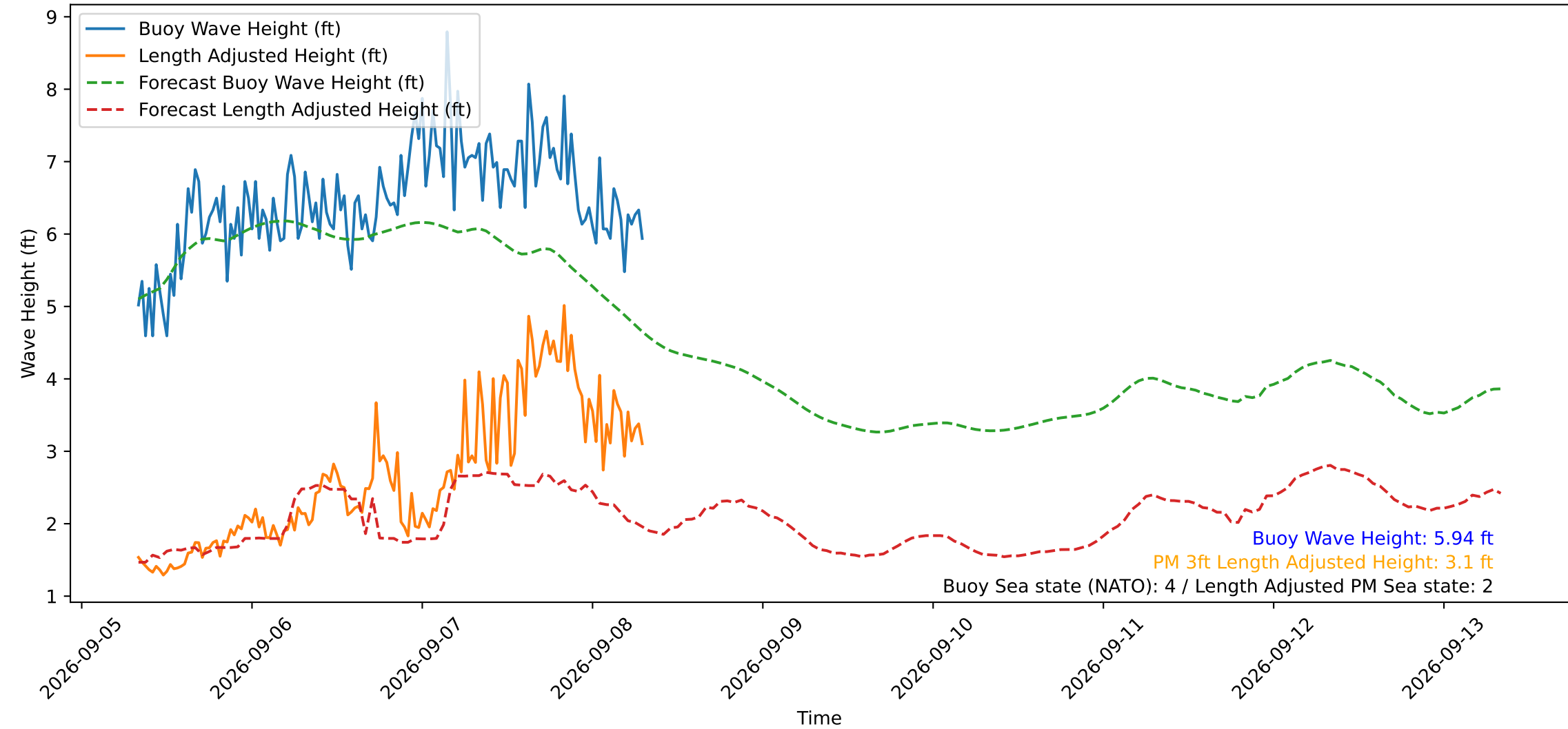
Wave Heights over Time for Green Beach at 2026-09-08 07:51:15
