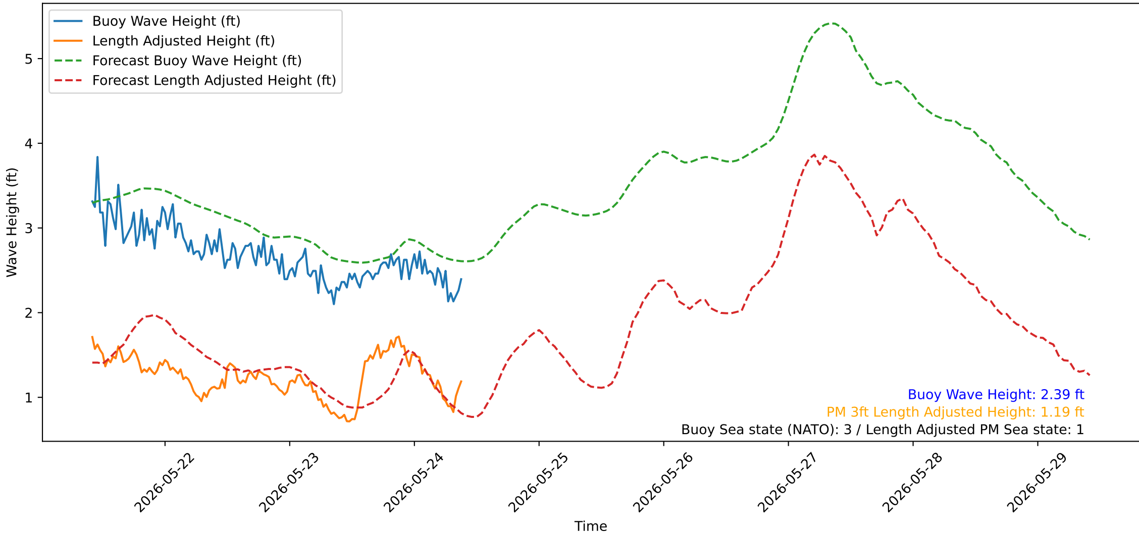
Wave Heights over Time for Oceanside Harbor at 2026-05-24 09:50:32
