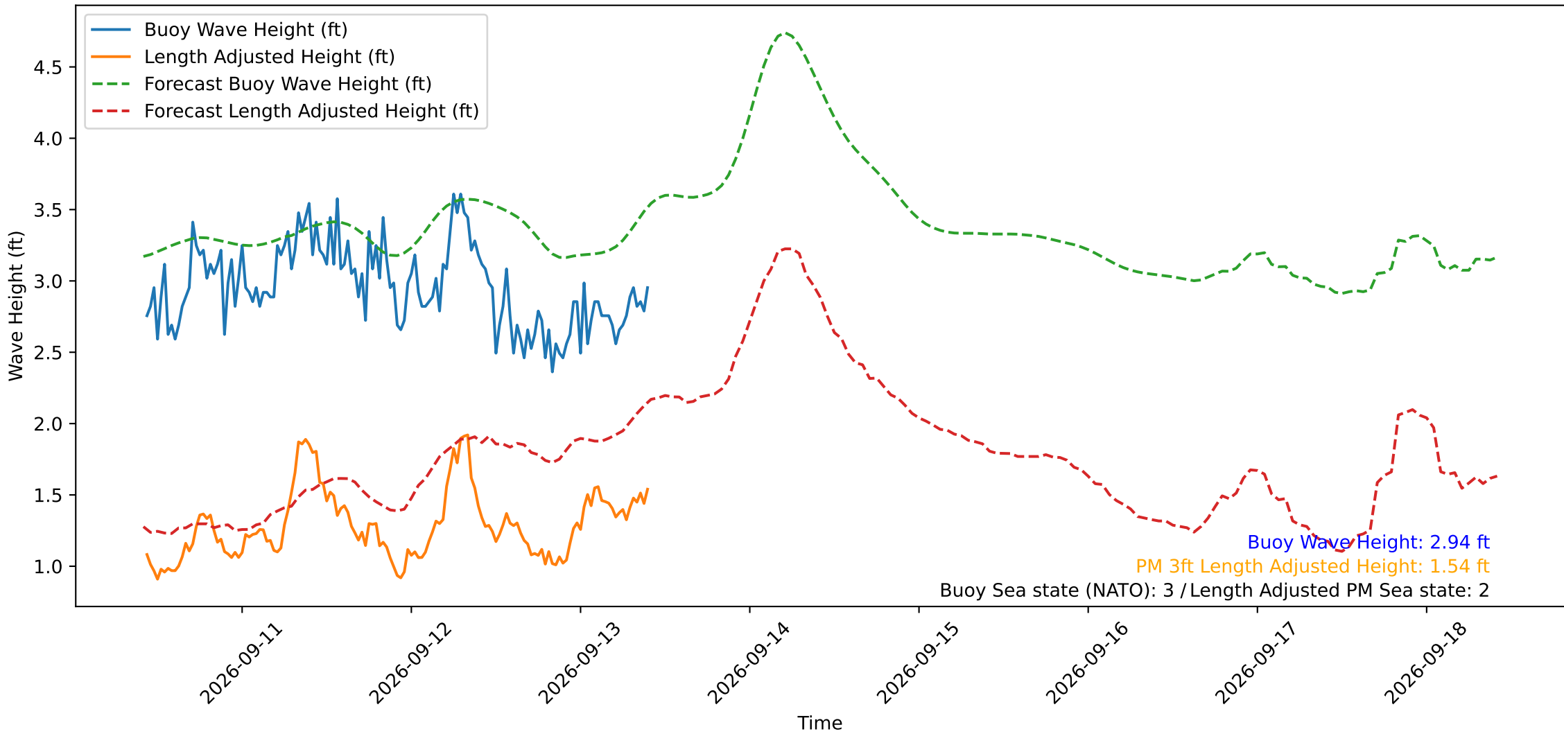
Wave Heights over Time for Green Beach at 2026-09-13 10:21:15
