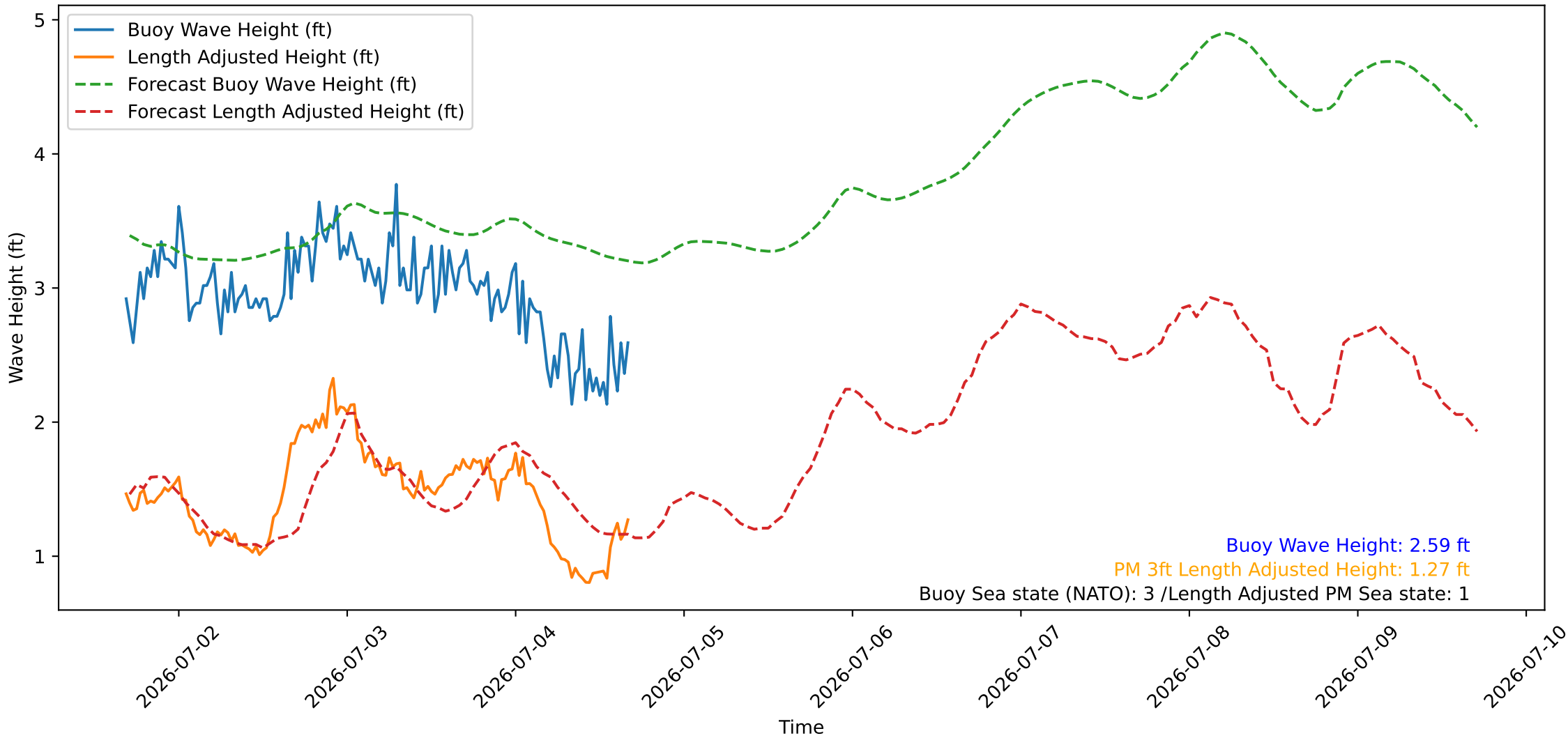
Wave Heights over Time for Oceanside Harbor at 2026-07-04 16:30:27
