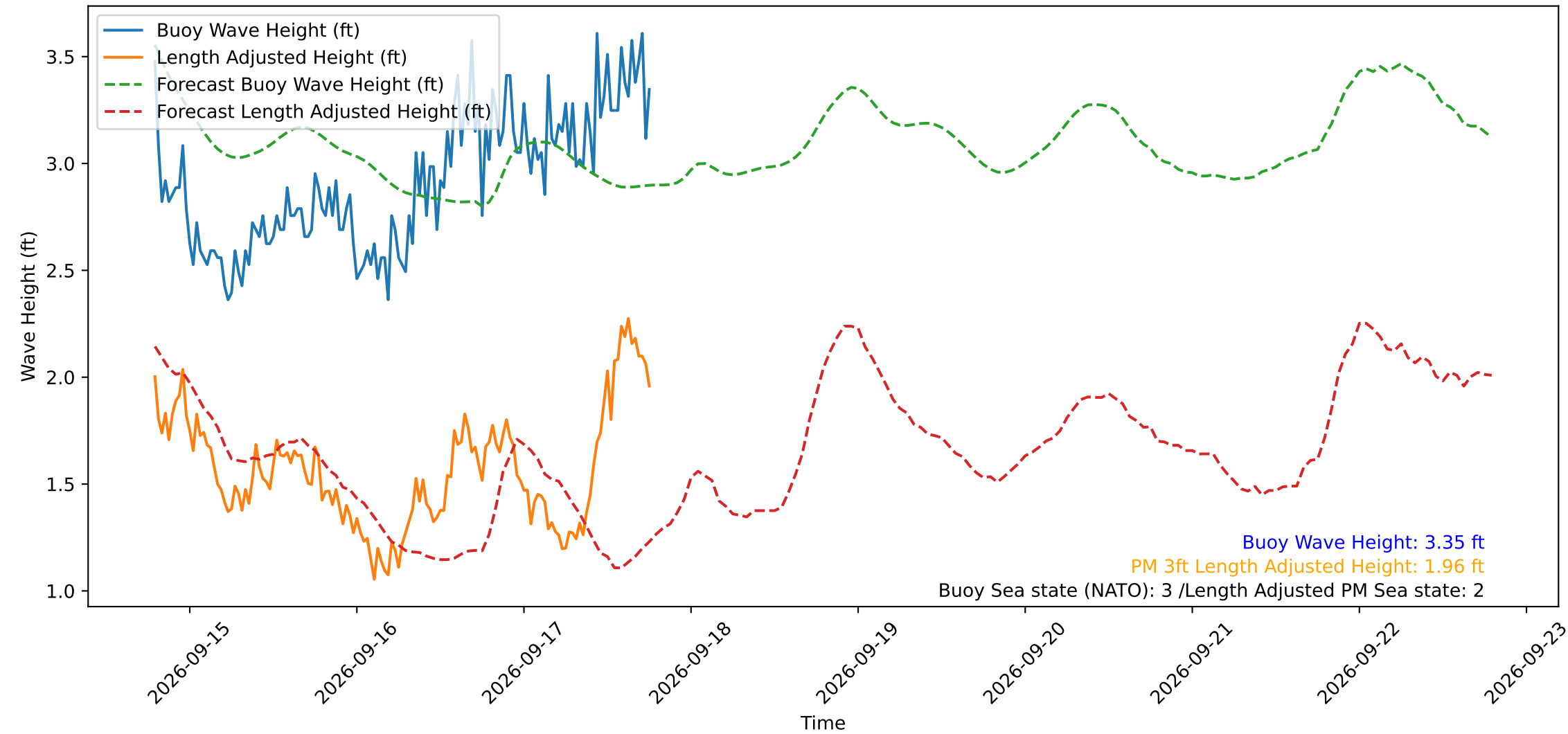
Wave Heights over Time for Oceanside Harbor at 2026-09-17 18:50:29
