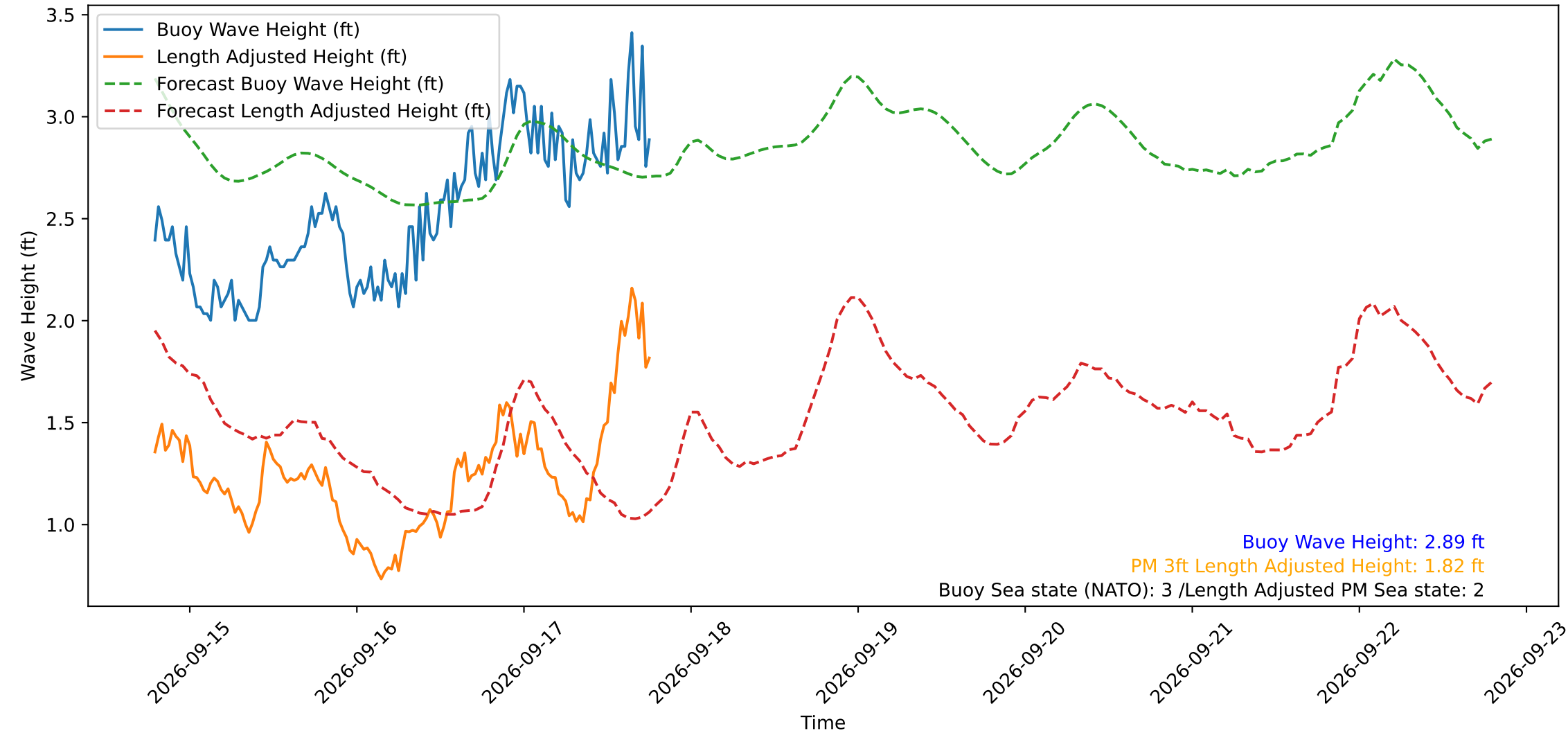
Wave Heights over Time for Red Beach at 2026-09-17 18:50:50
