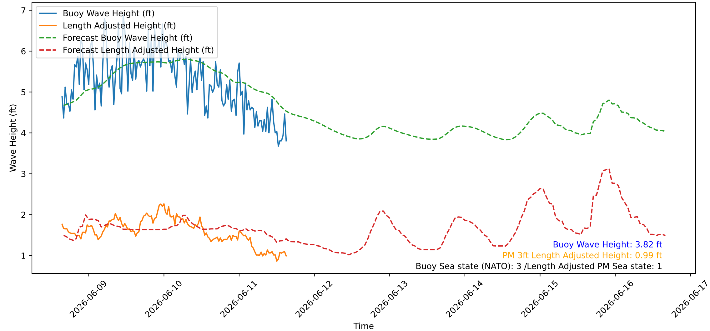
Wave Heights over Time for Green Beach at 2026-06-11 15:41:09
