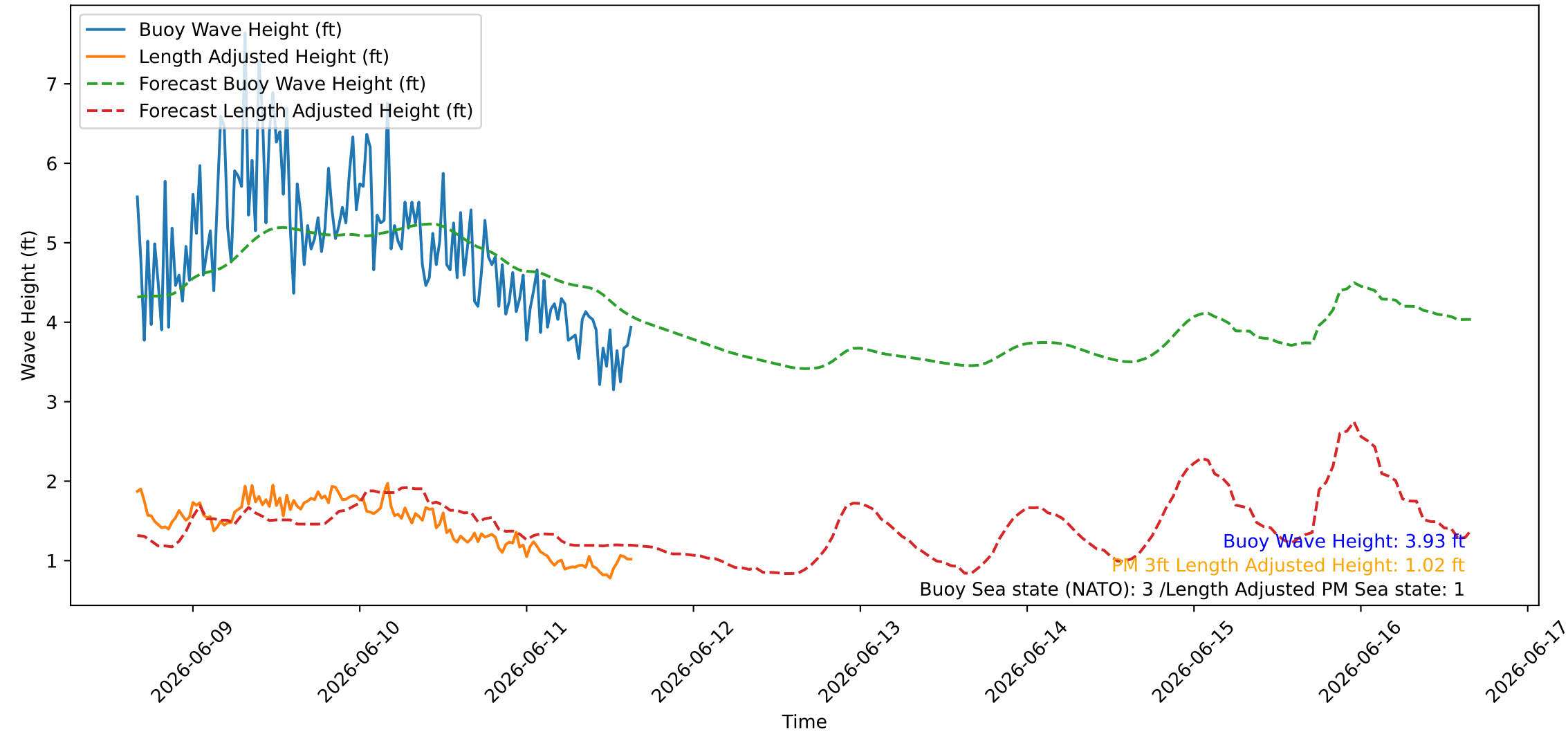
Wave Heights over Time for Red Beach at 2026-06-11 15:40:47
