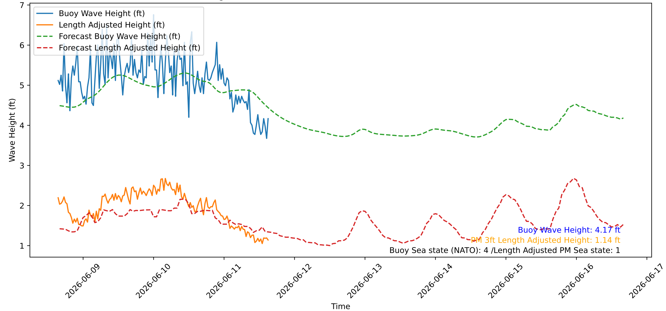
Wave Heights over Time for Oceanside Harbor at 2026-06-11 15:40:26
